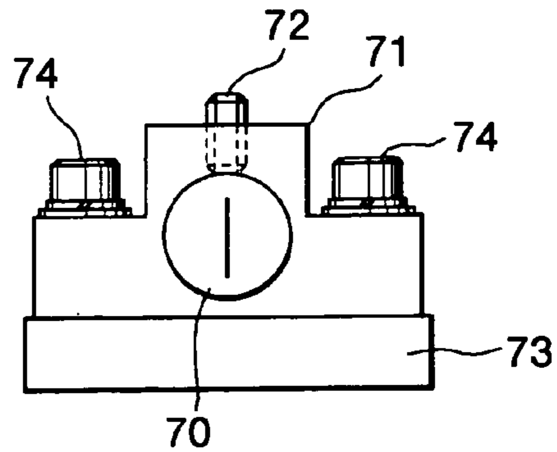
FIG. 3 PRIOR ART
