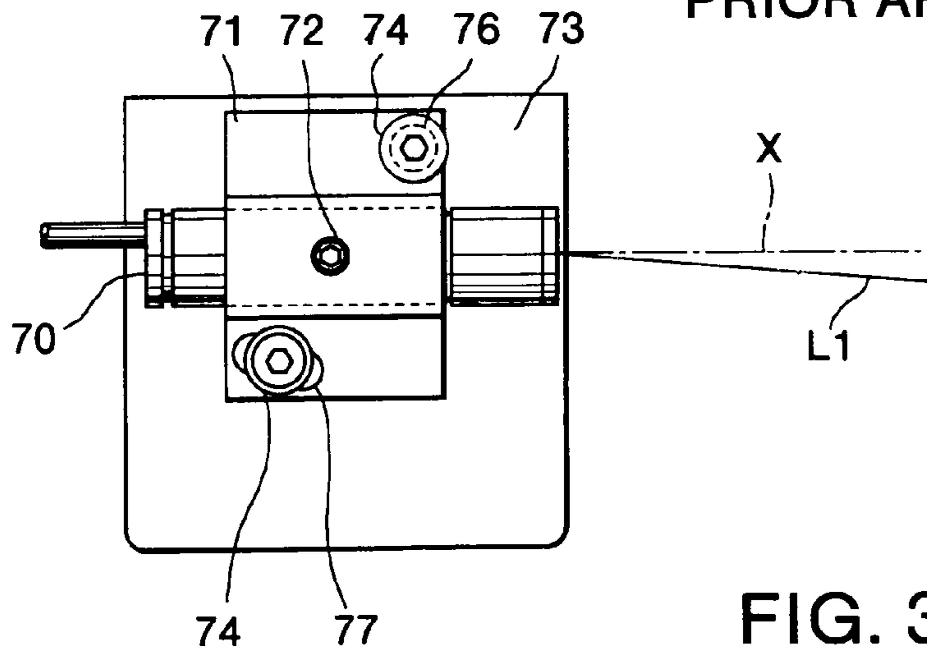
FIG. 2 PRIOR ART
