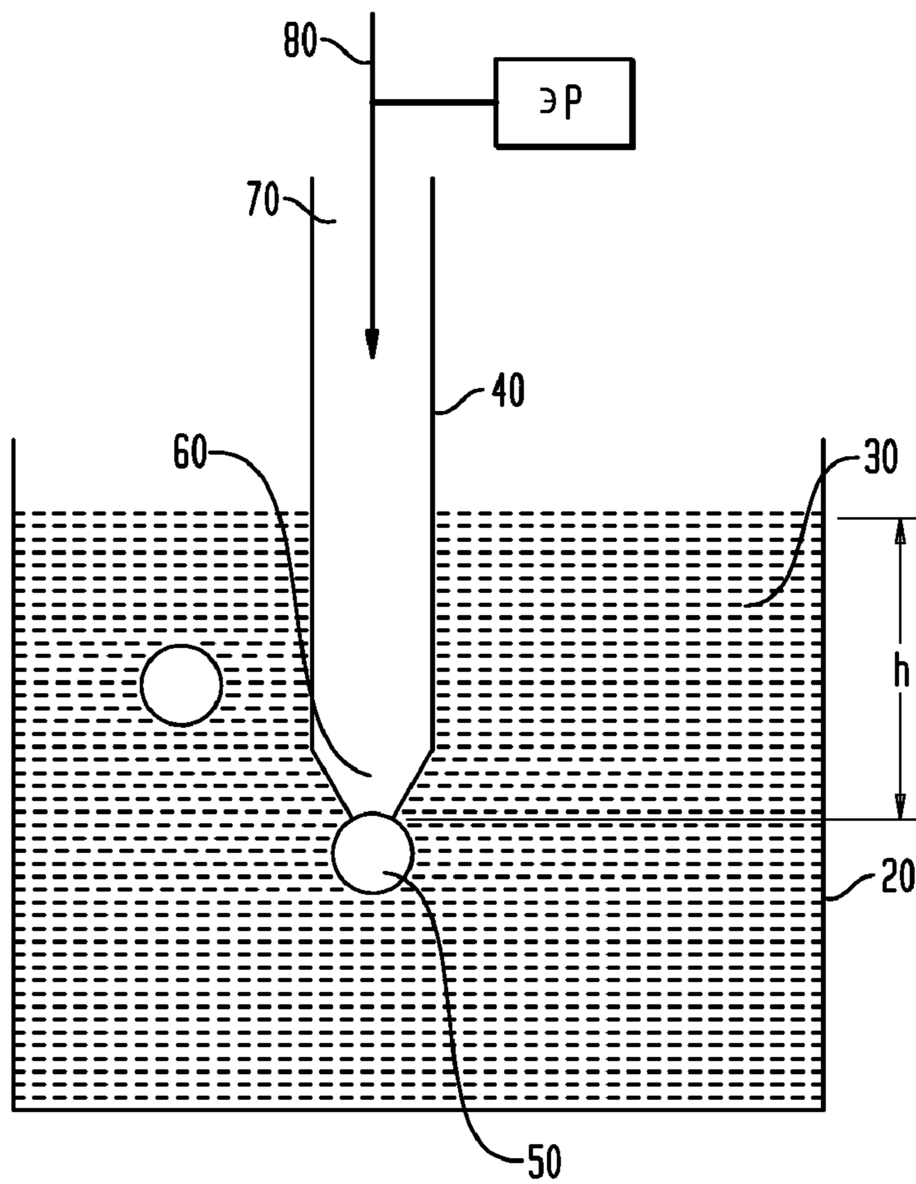
FIG. 2 MAXIMUM BUBBLE PRESSURE (MBP) METHOD
