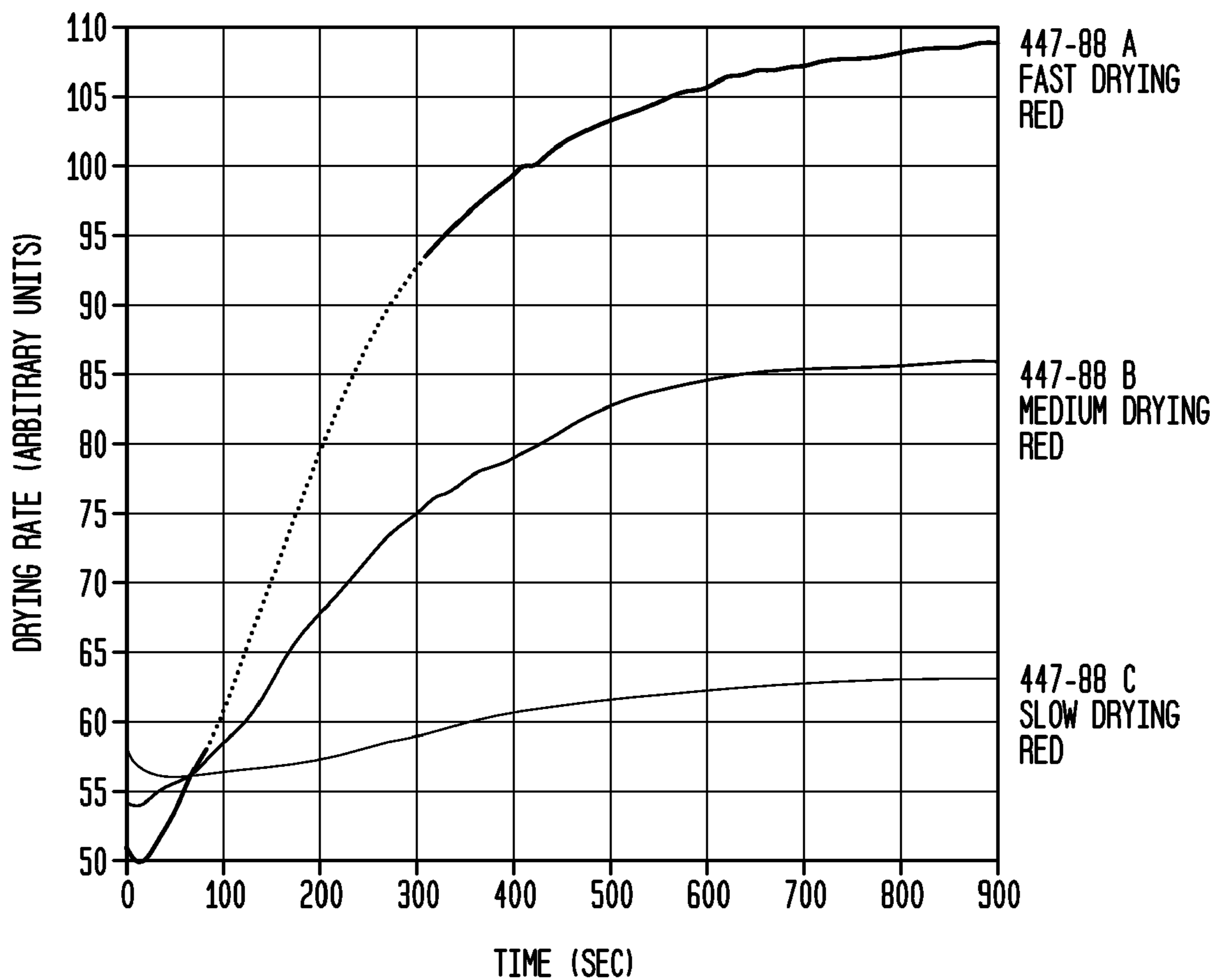
FIG. 8 DRYING/RESOLUBILITY RATE OF WATER-BASED INKS (SENSADYNE PC500L)
