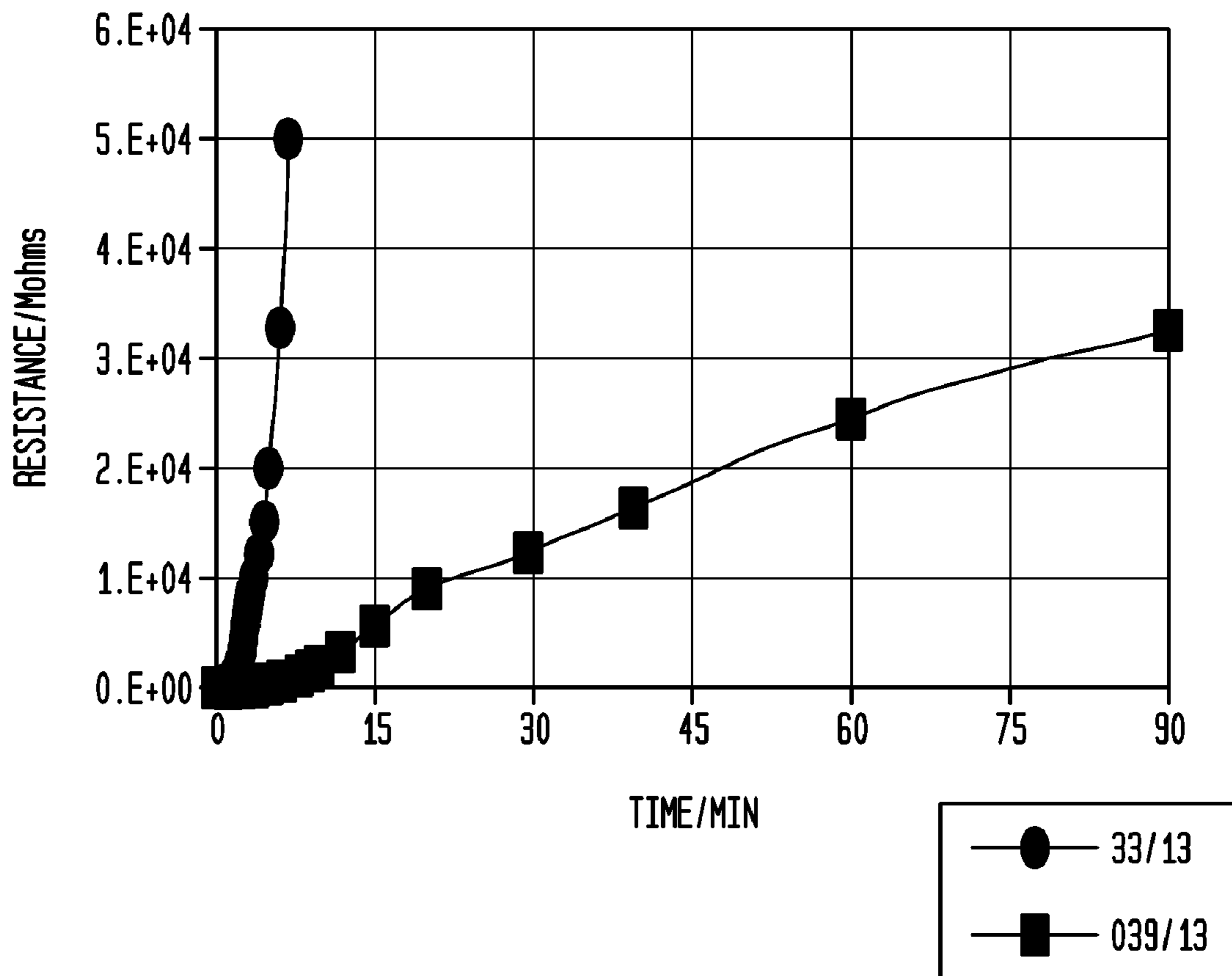
FIG. 12 FLEXOMAX 33 vs. 039 - (MAYER BAR #13)
