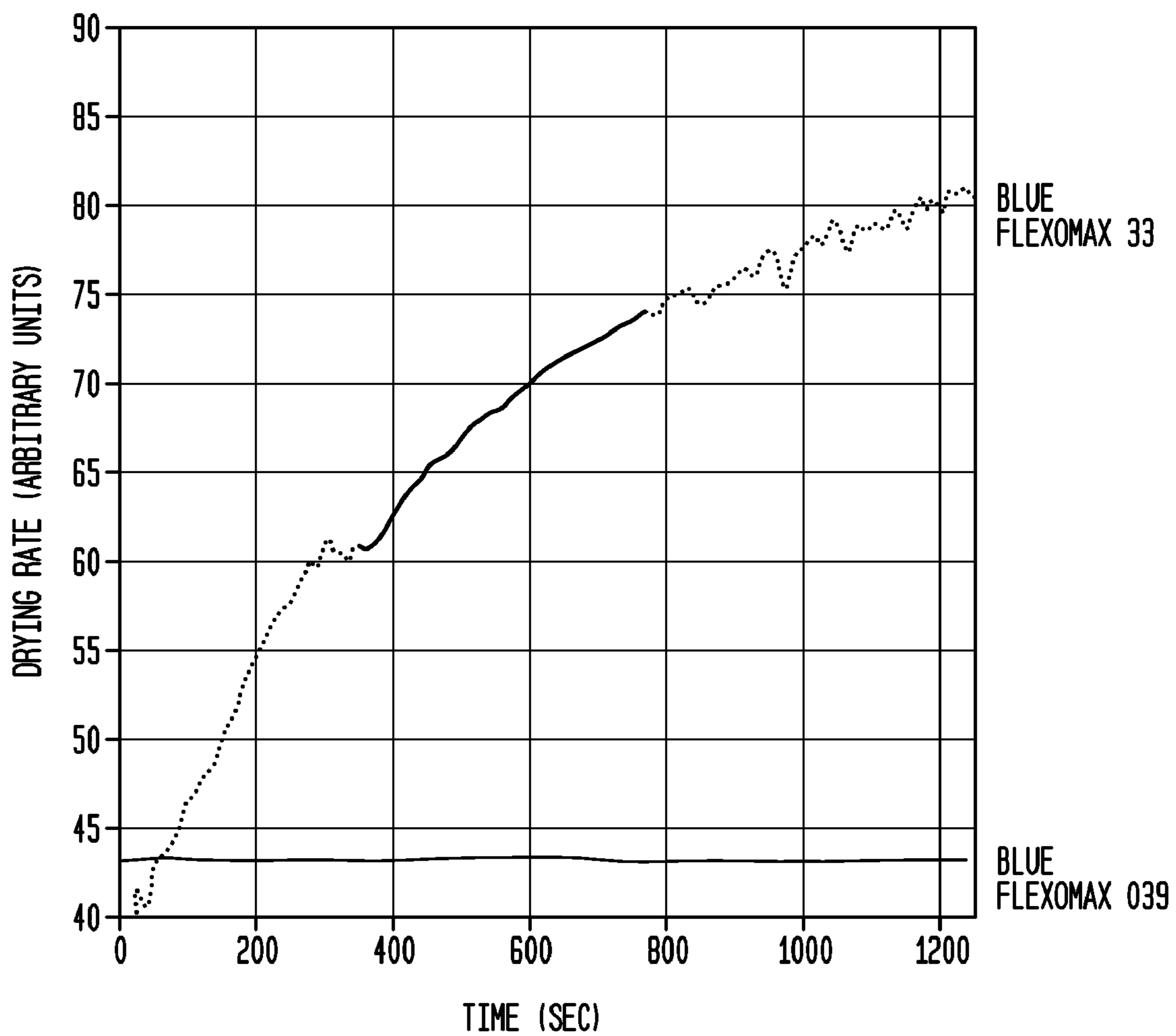
FIG. 9 DRYING/RESOLUBILITY RATE OF SOLVENT-BASED LAMINATING INKS (PC500L)
