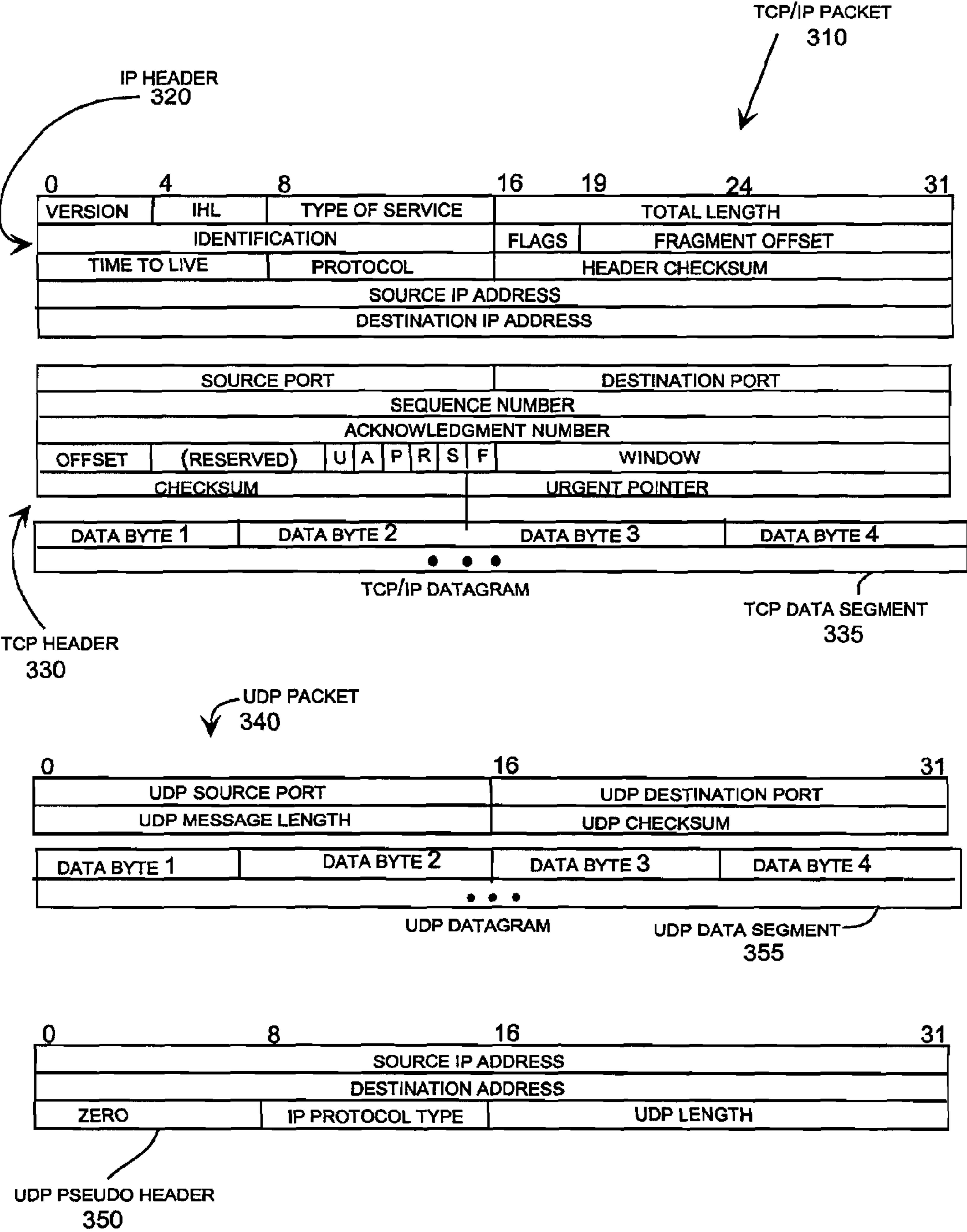
PACKET HEADERS FIG. 3
