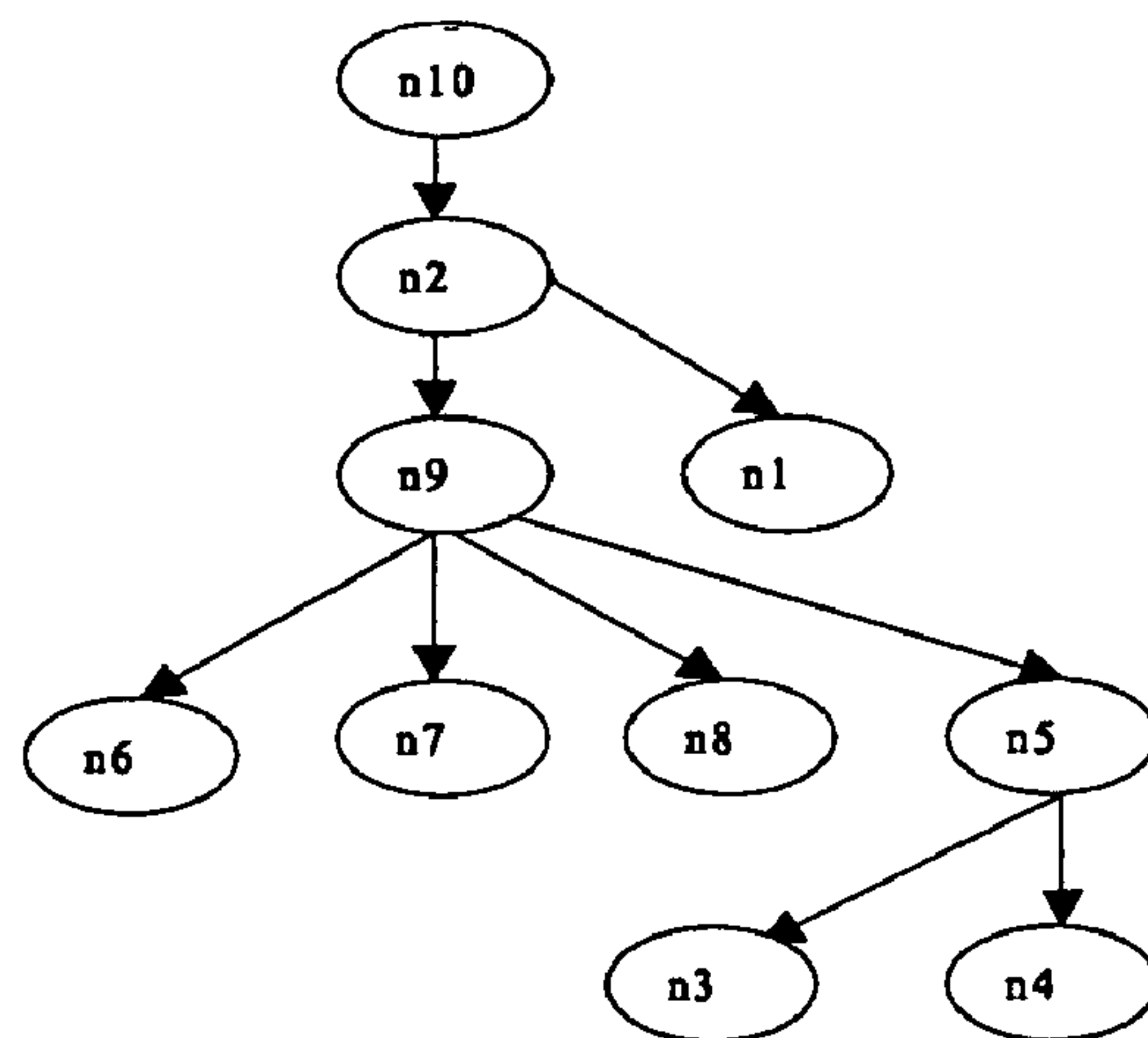
Fig. 4 (Example prior art post-dominator graph)
