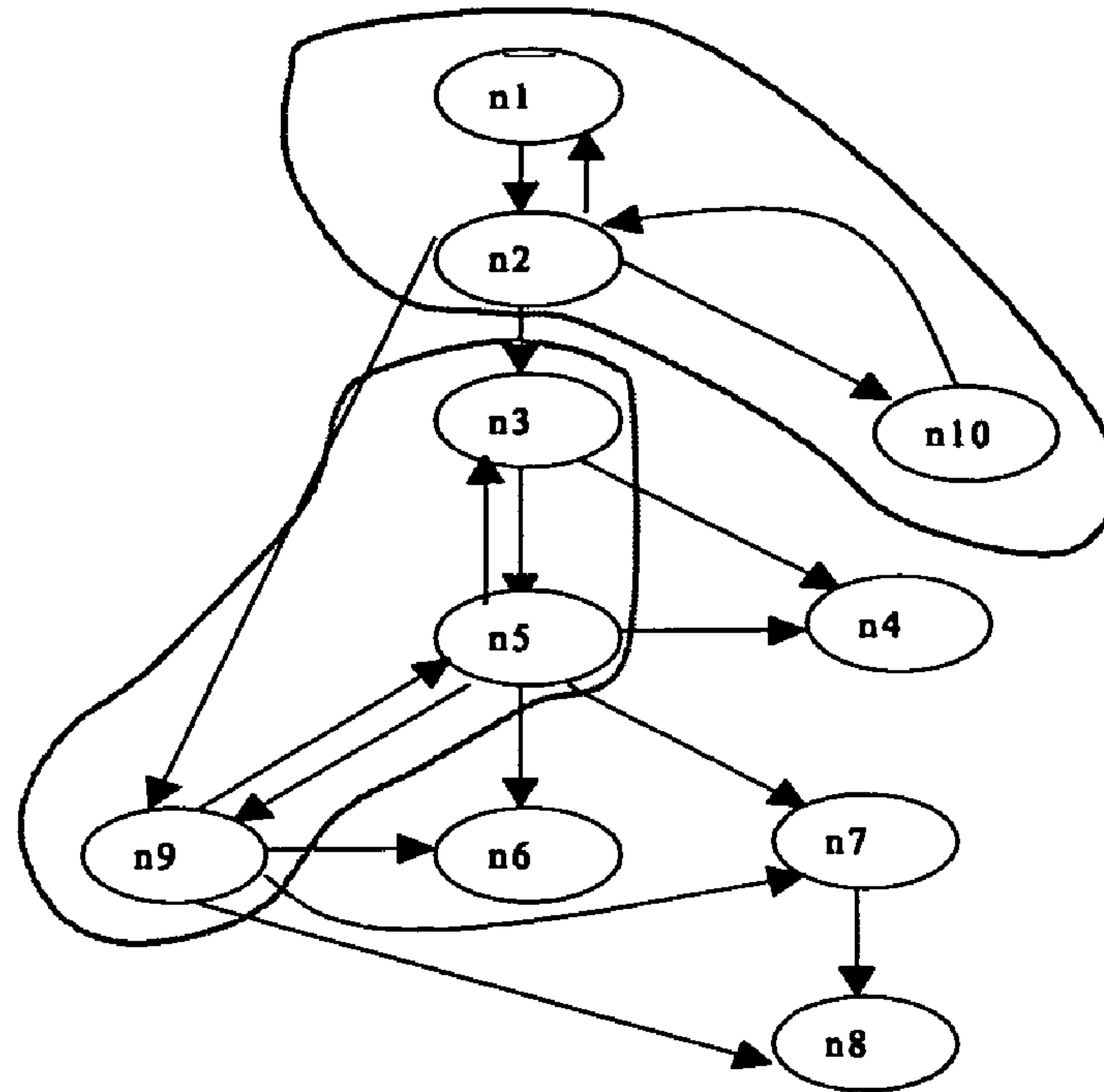
Fig. 5 (Example prior art combination graph)
