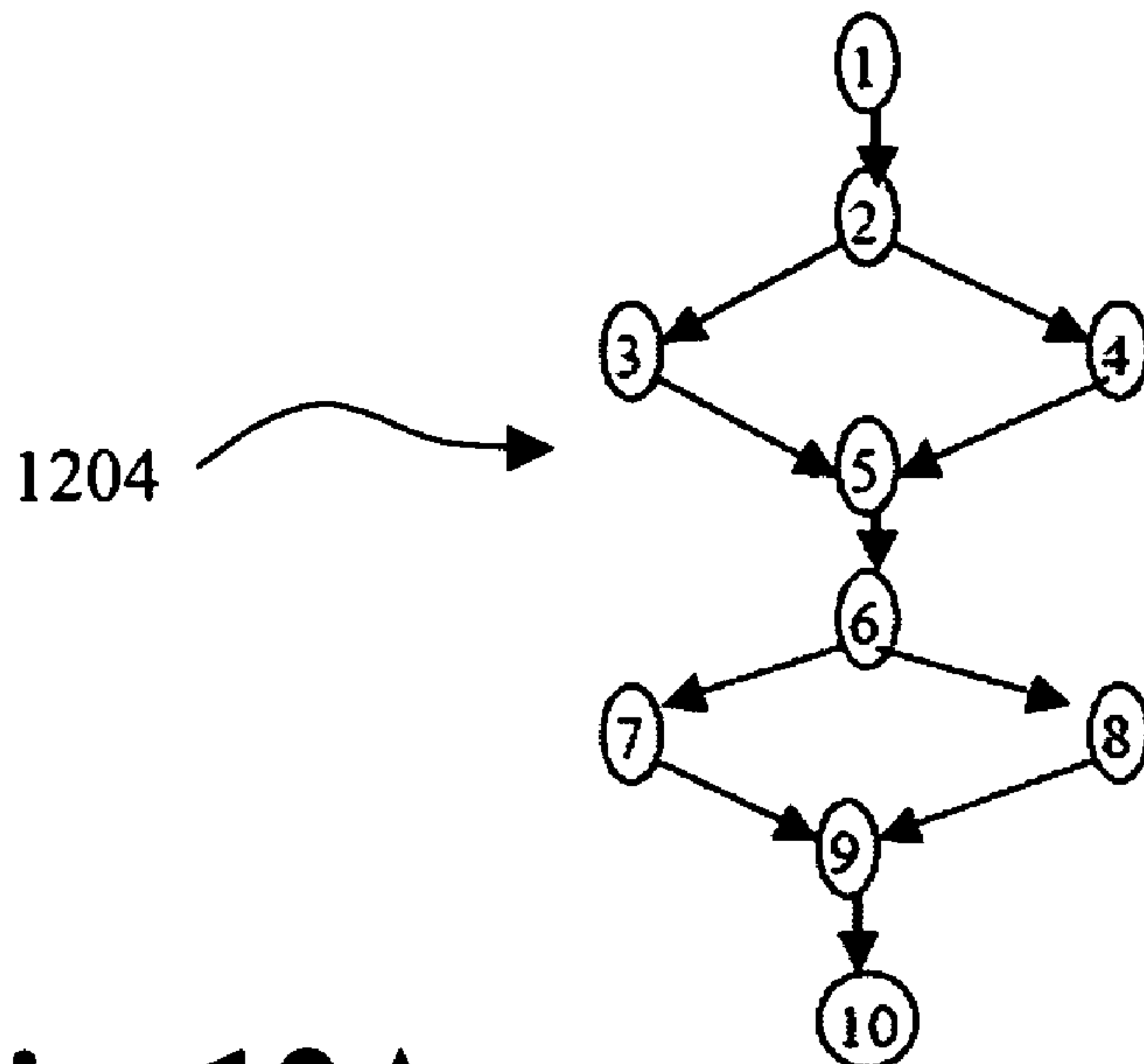
Fig. 12A A control flow diagram example
