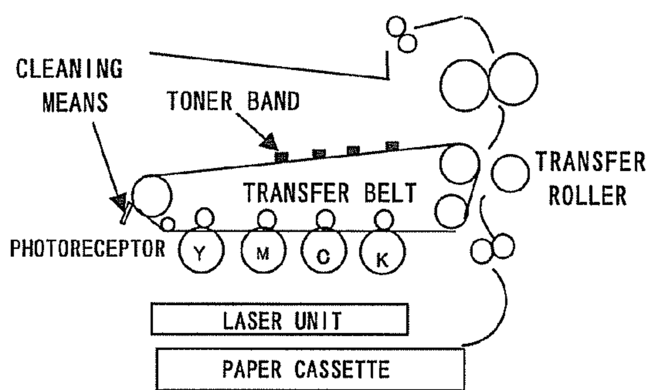
TONER BAND AVOIDING TIMING AT ACTIVATION
