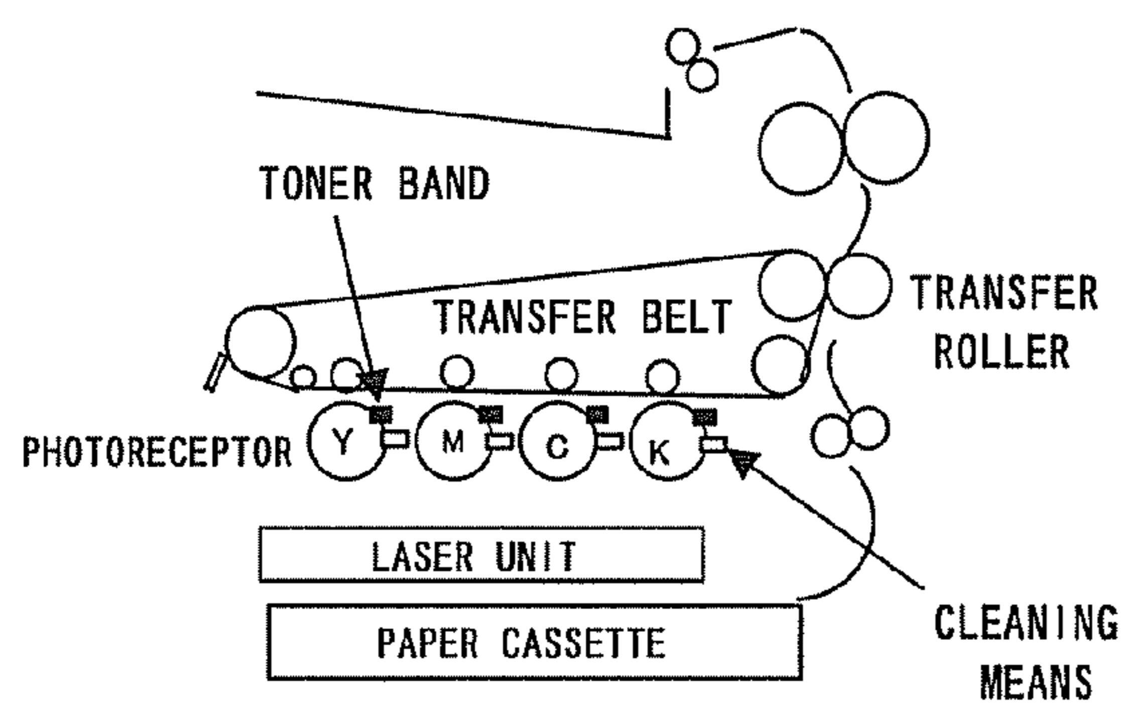
TONER BAND AVOIDING TIMING AT ACTIVATION
