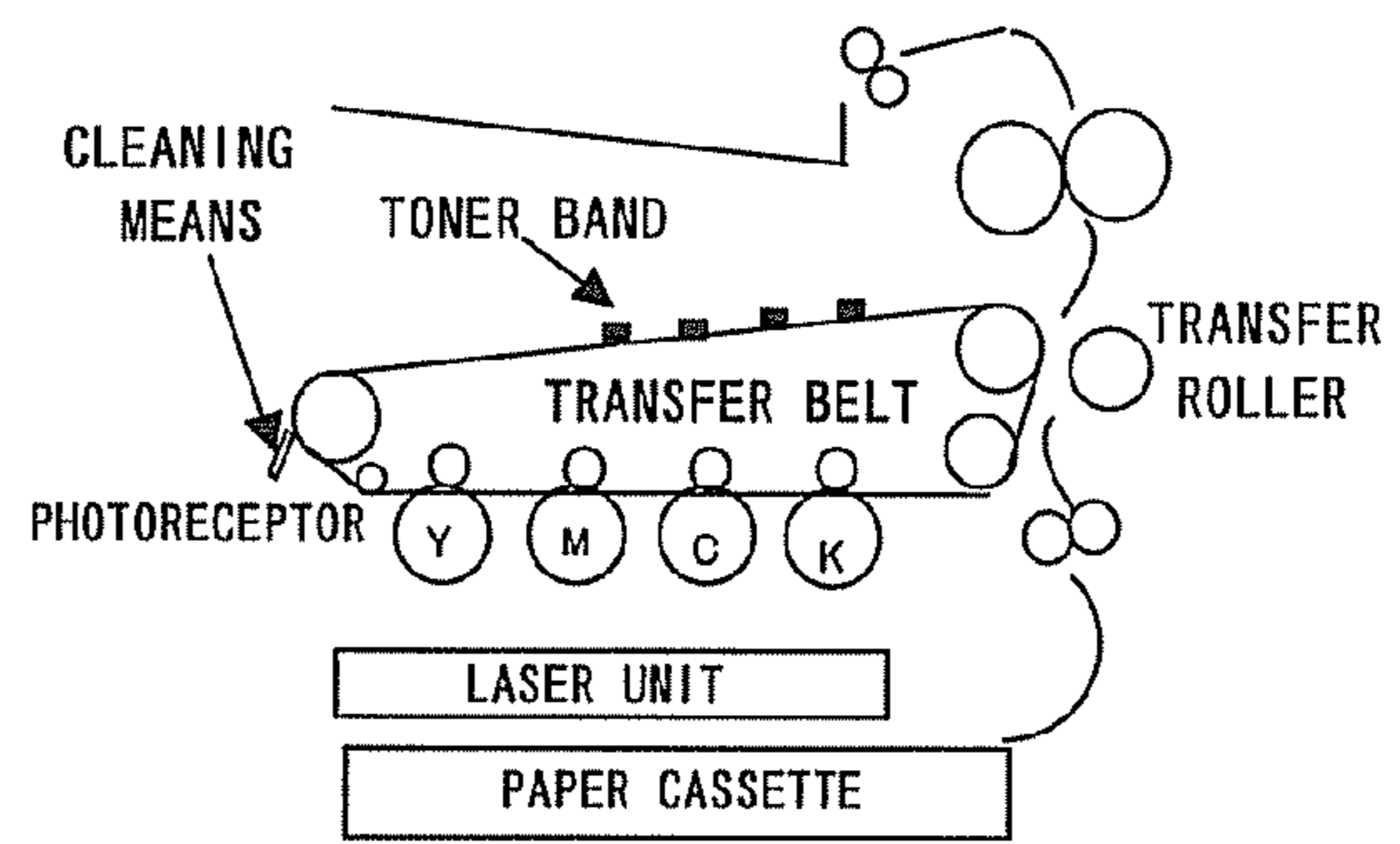
TONER BAND AVOIDING TIMING AT STOPPAGE
