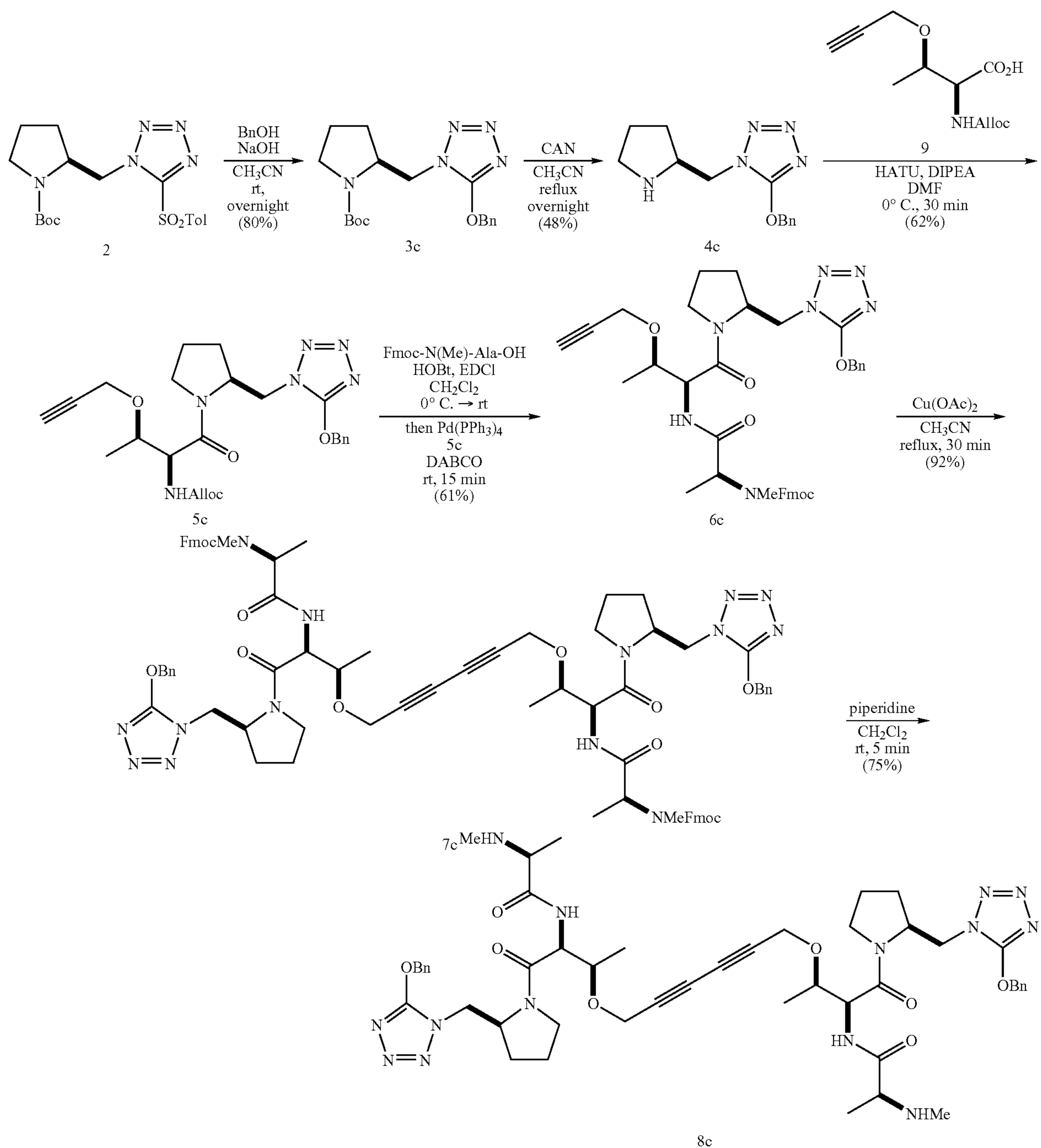
Scheme 3
