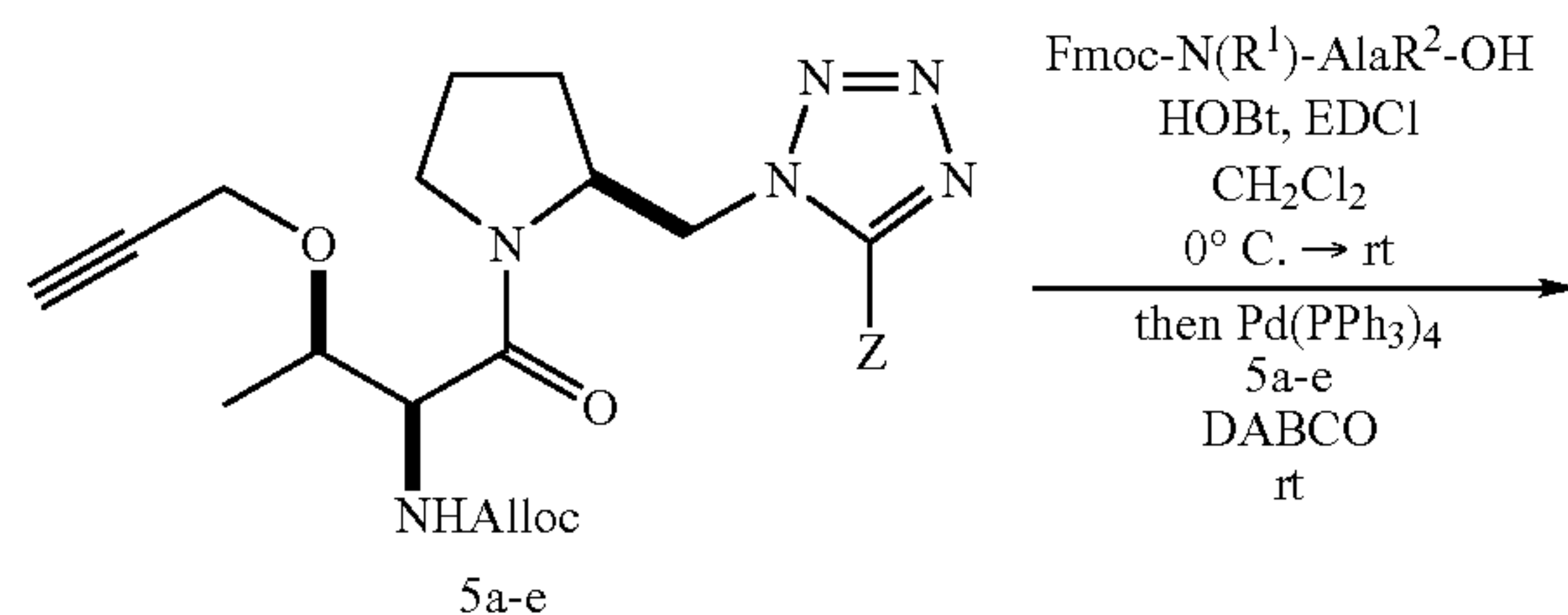
Scheme 9
