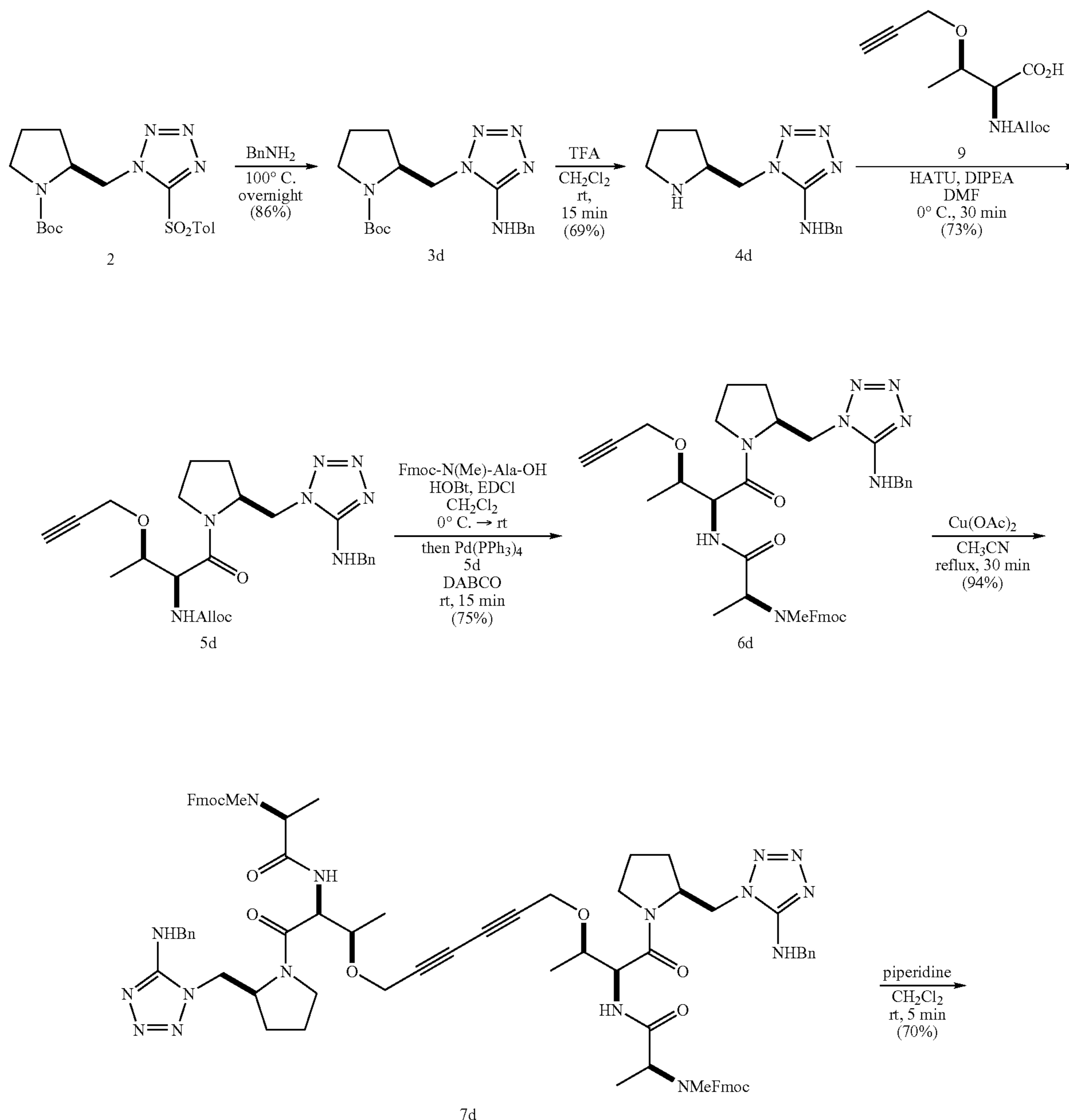
Scheme 4
