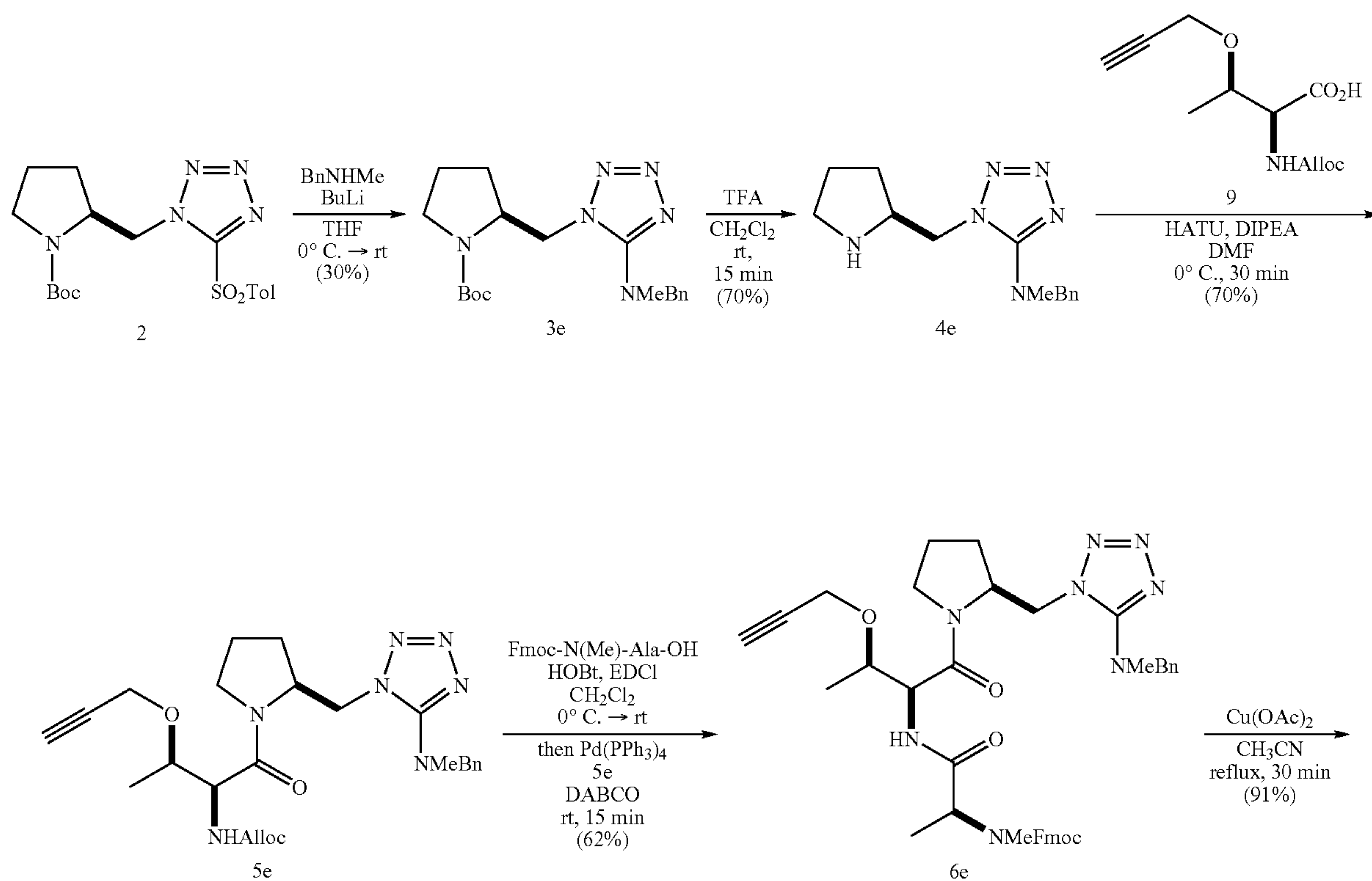
Scheme 5
