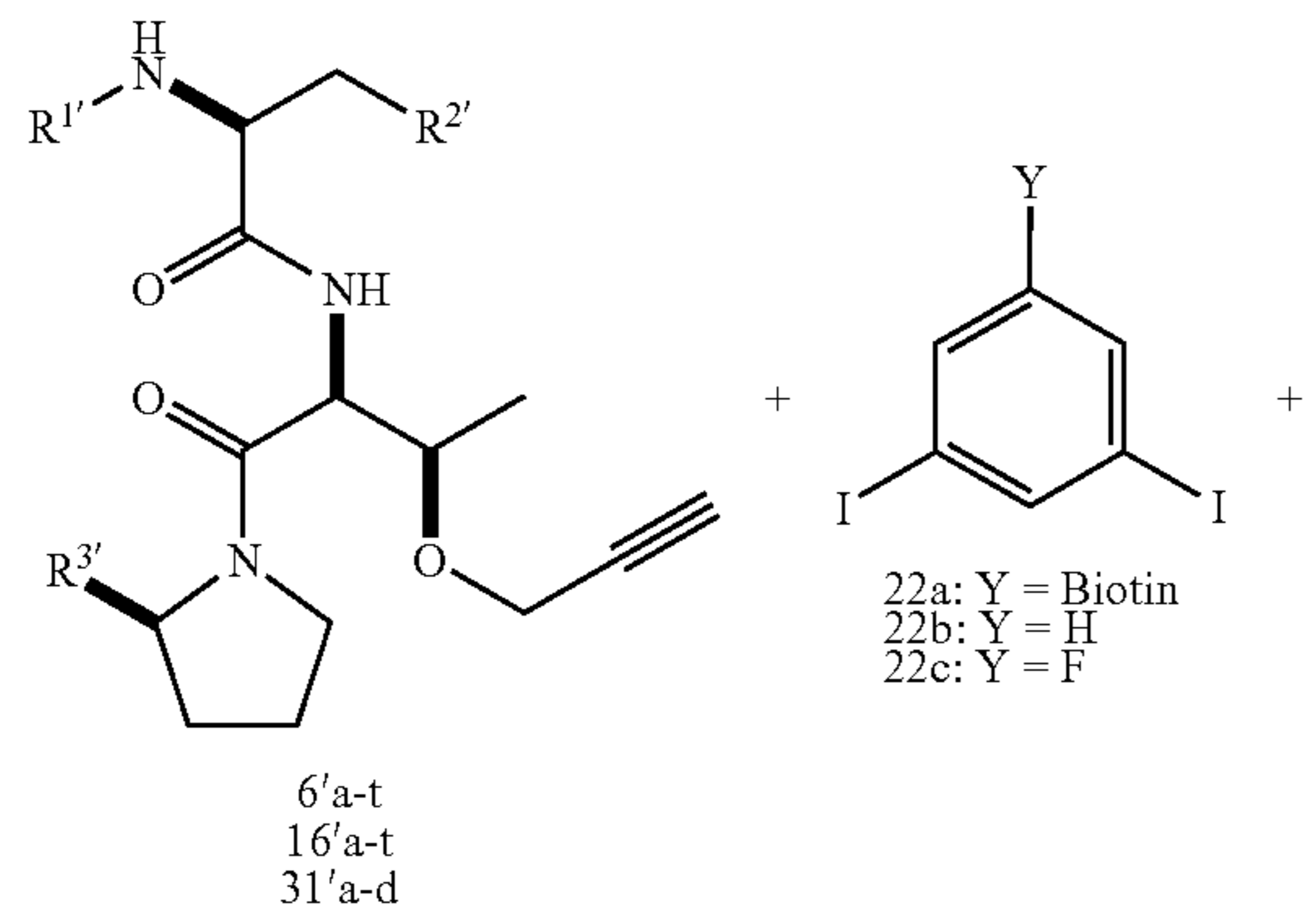
Scheme 13
