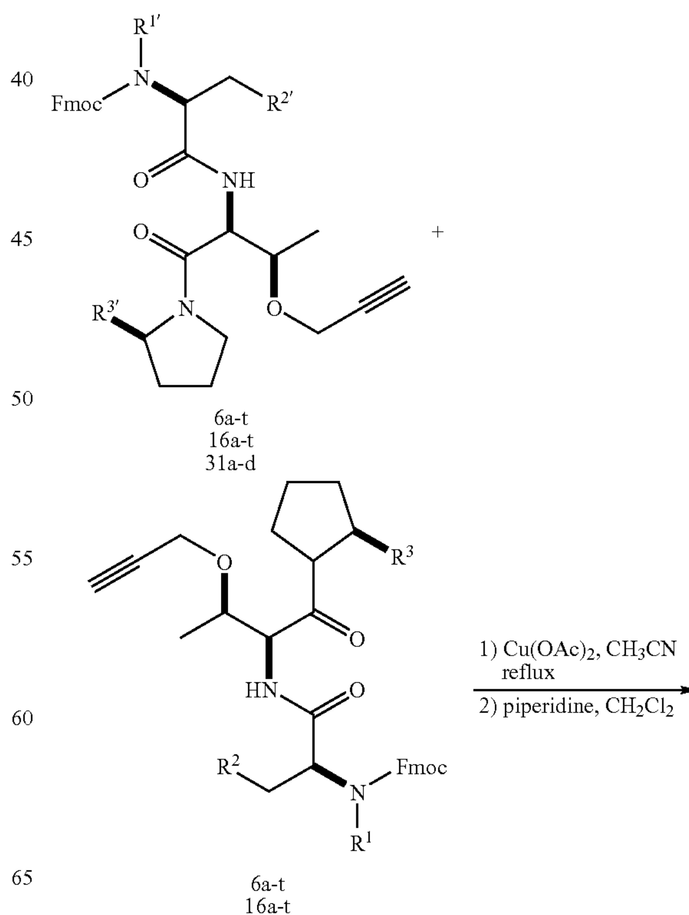
Scheme 12
