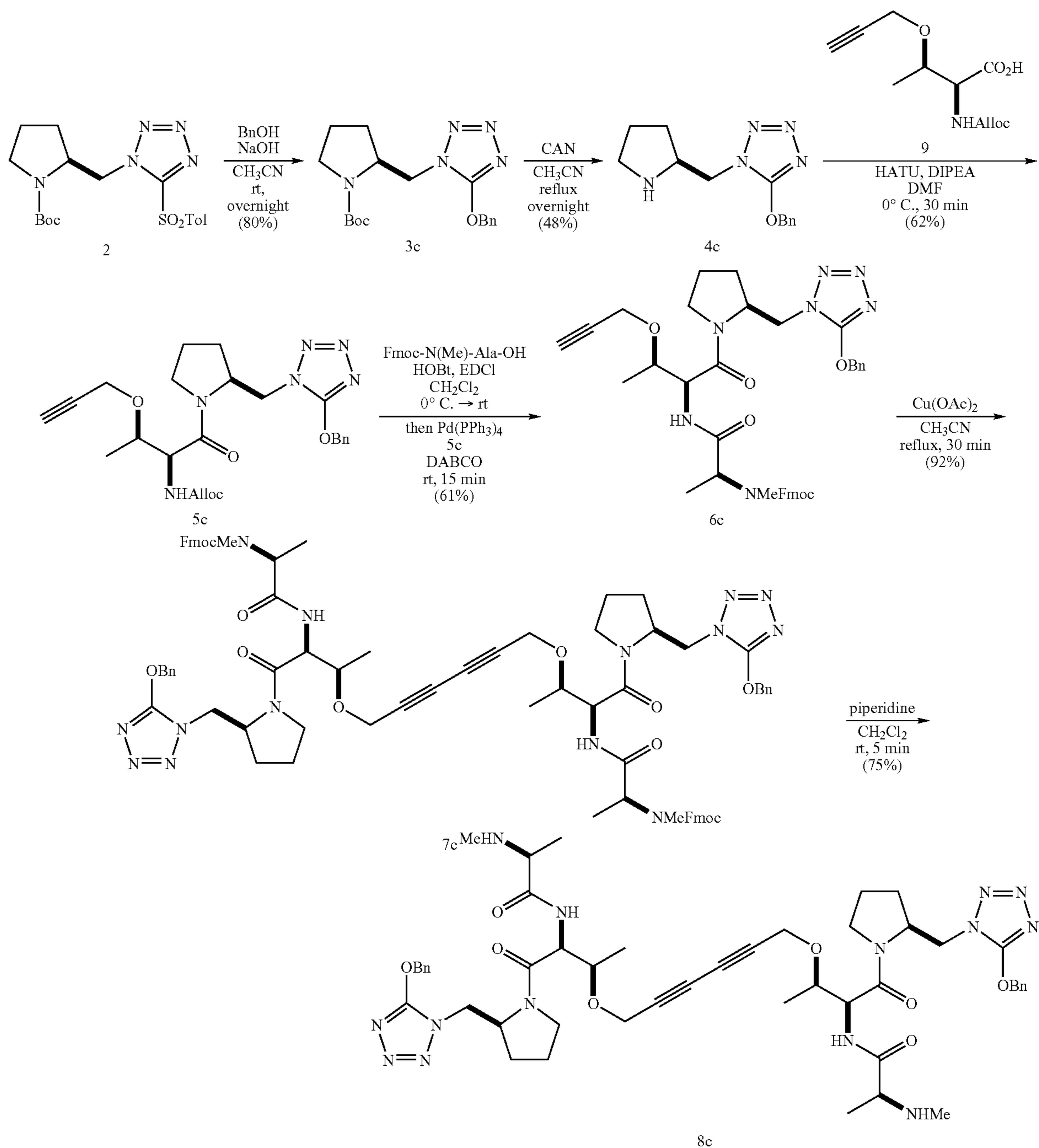
Scheme 3
