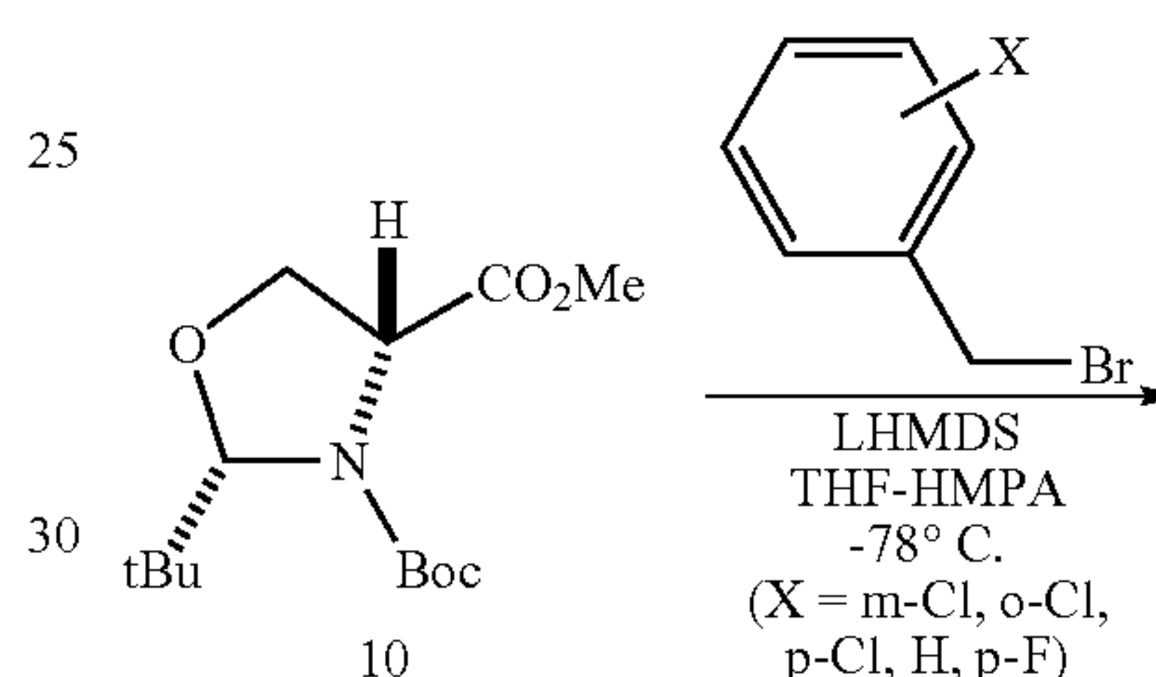
Scheme 10
