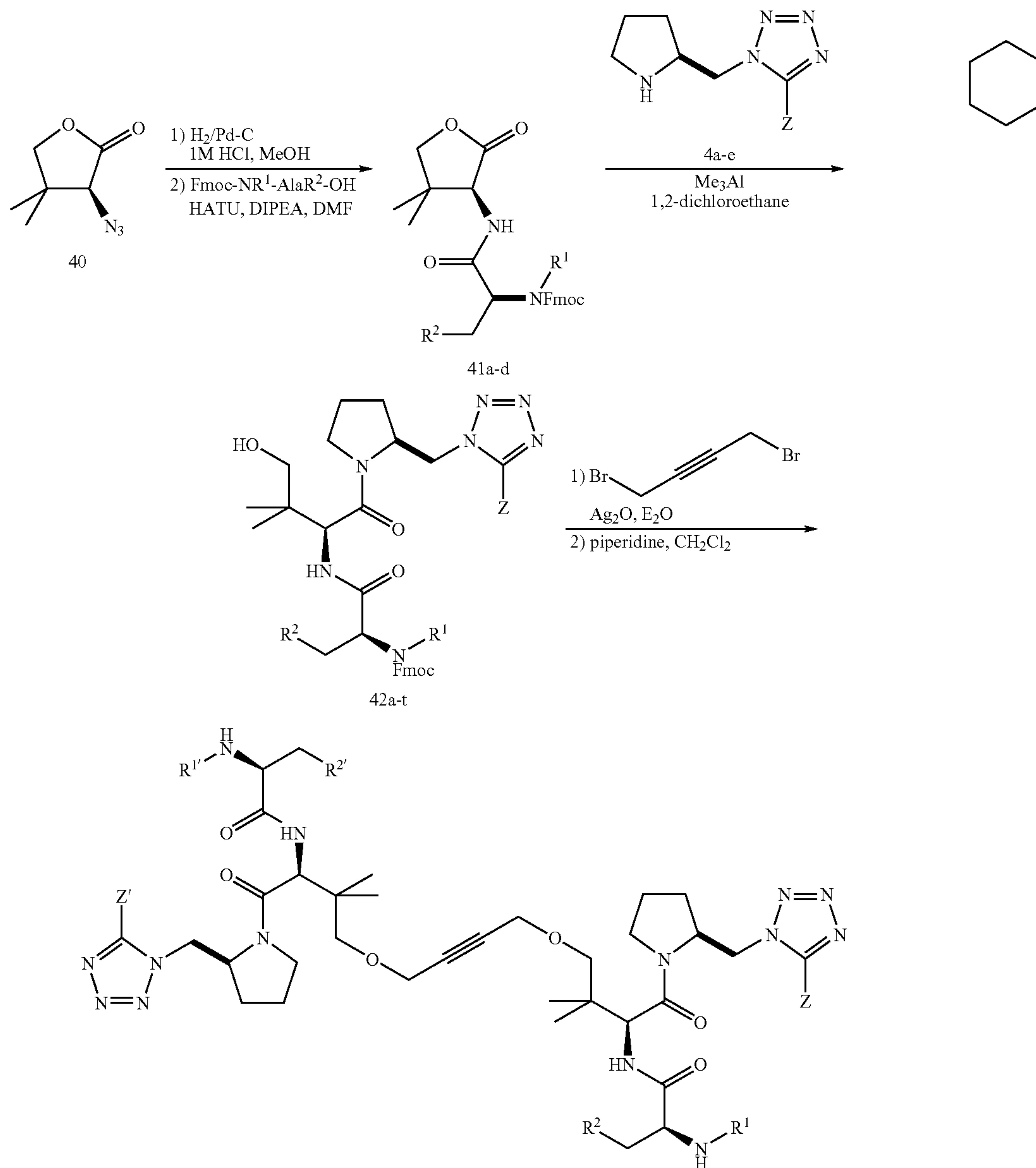
Scheme 14
