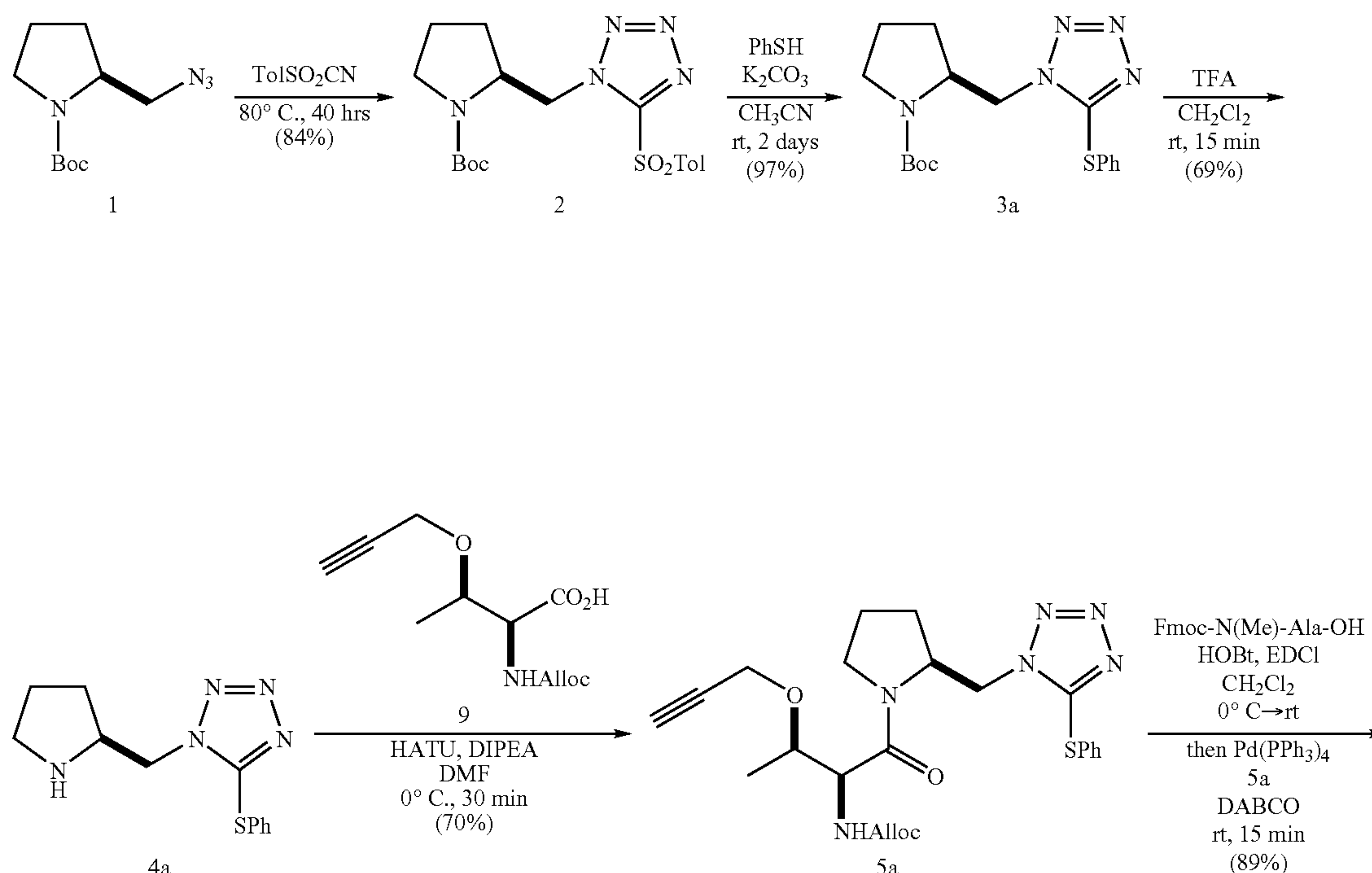
Scheme 1
