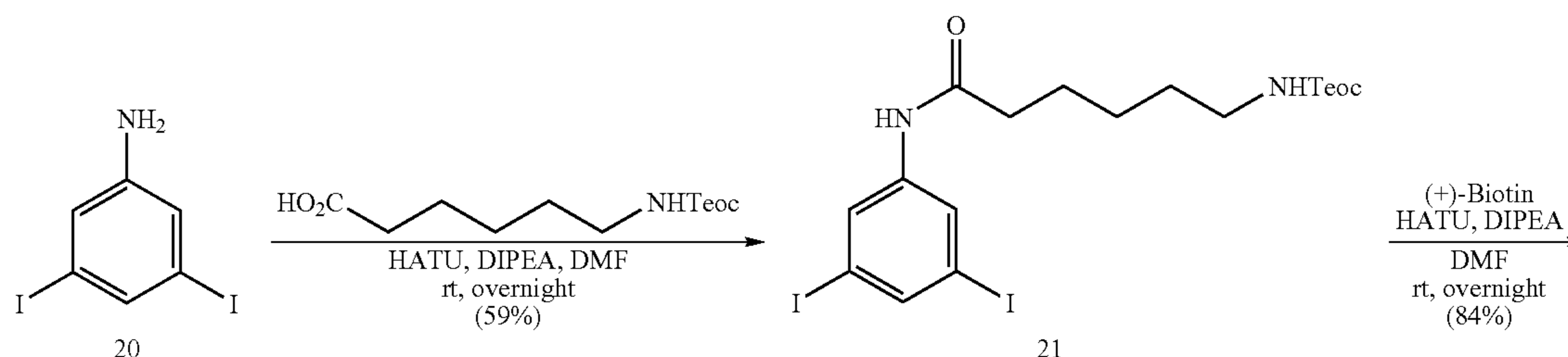
Scheme 7
