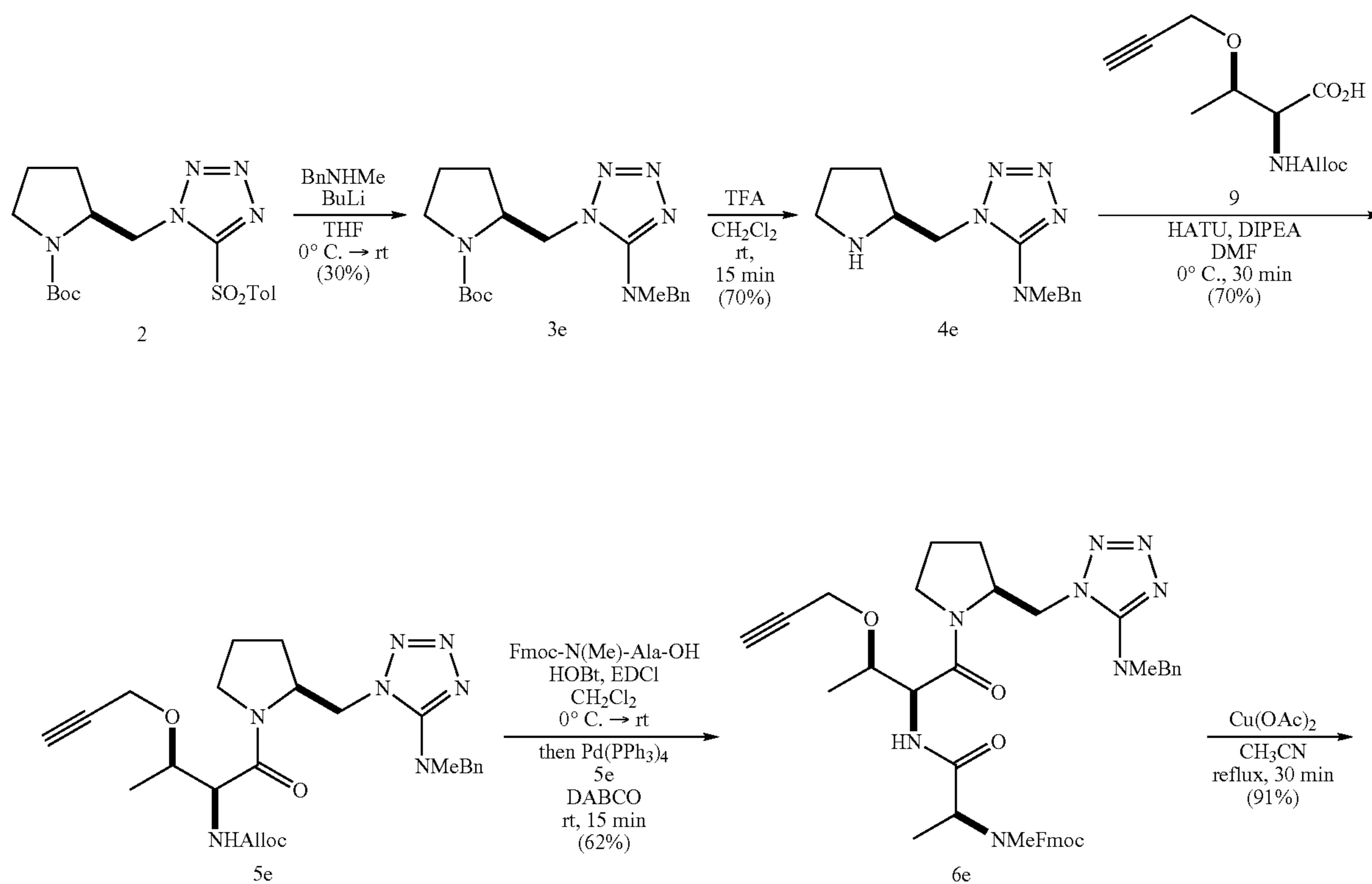
Scheme 5
