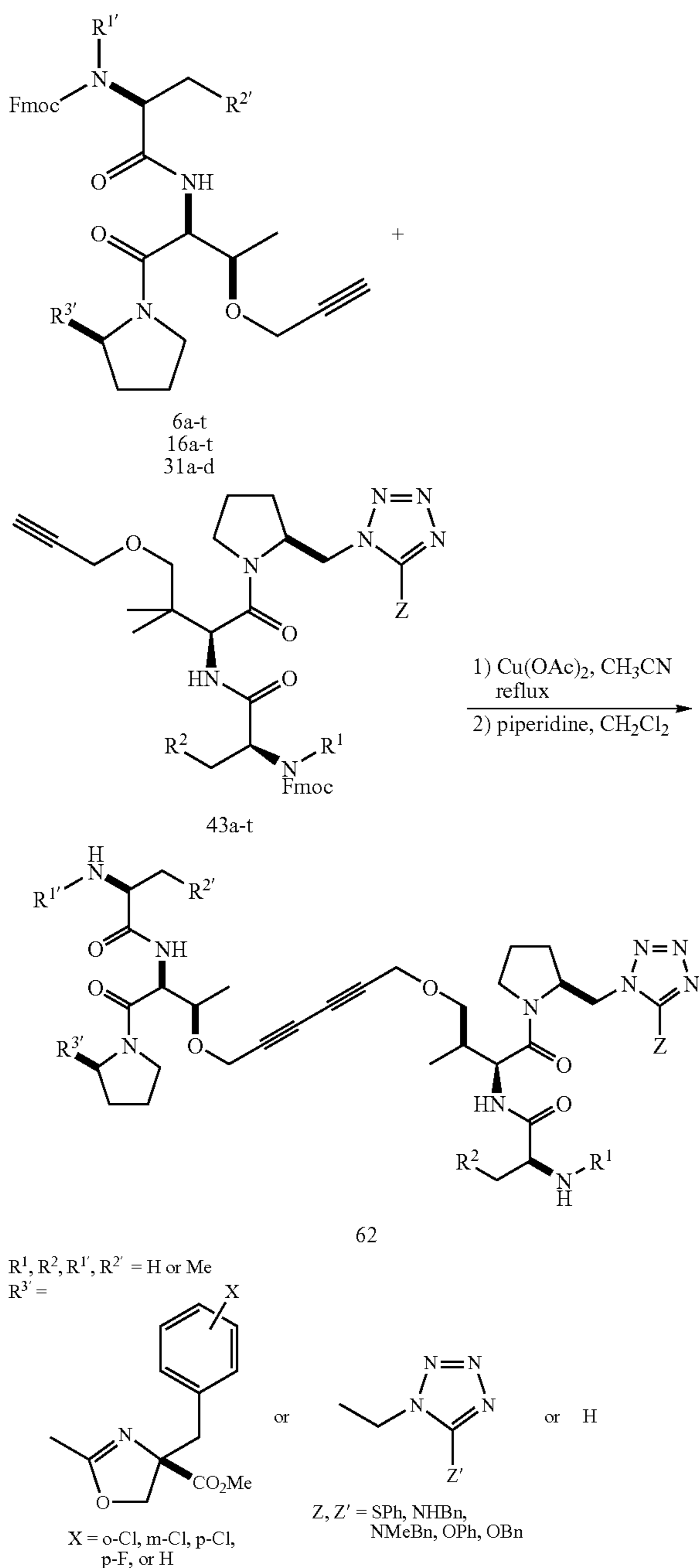
Scheme 17
