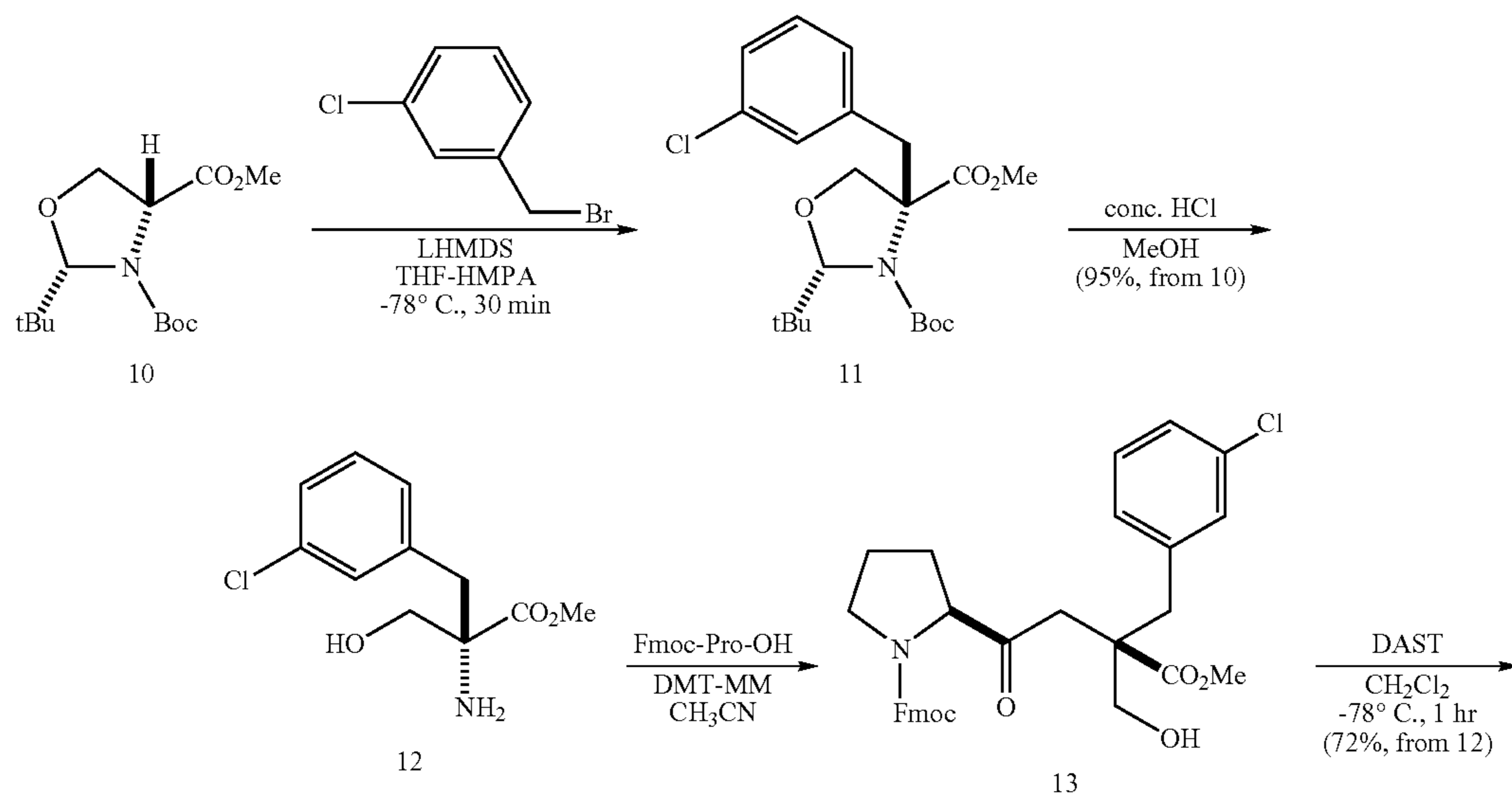
Scheme 6
