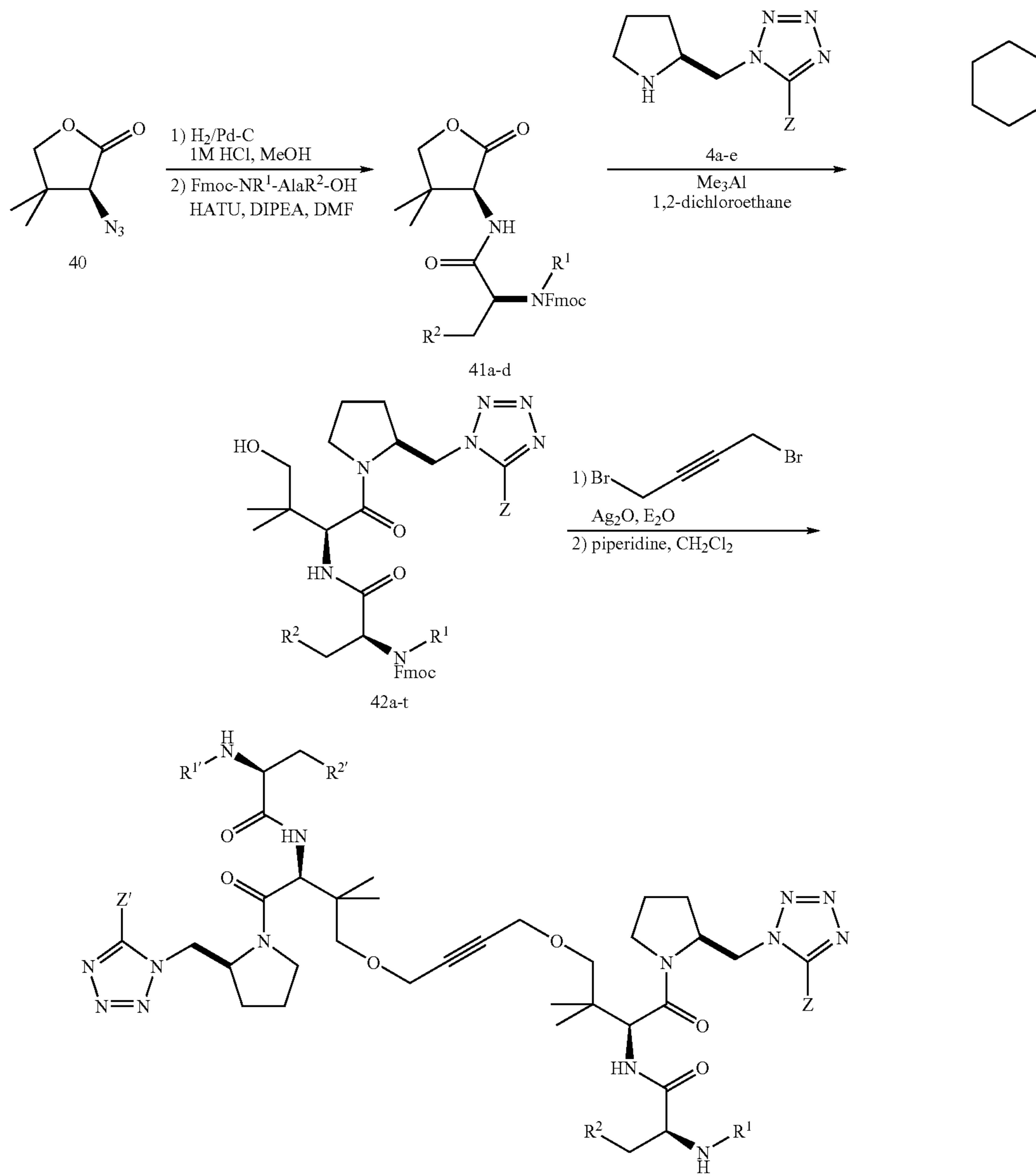
Scheme 14
