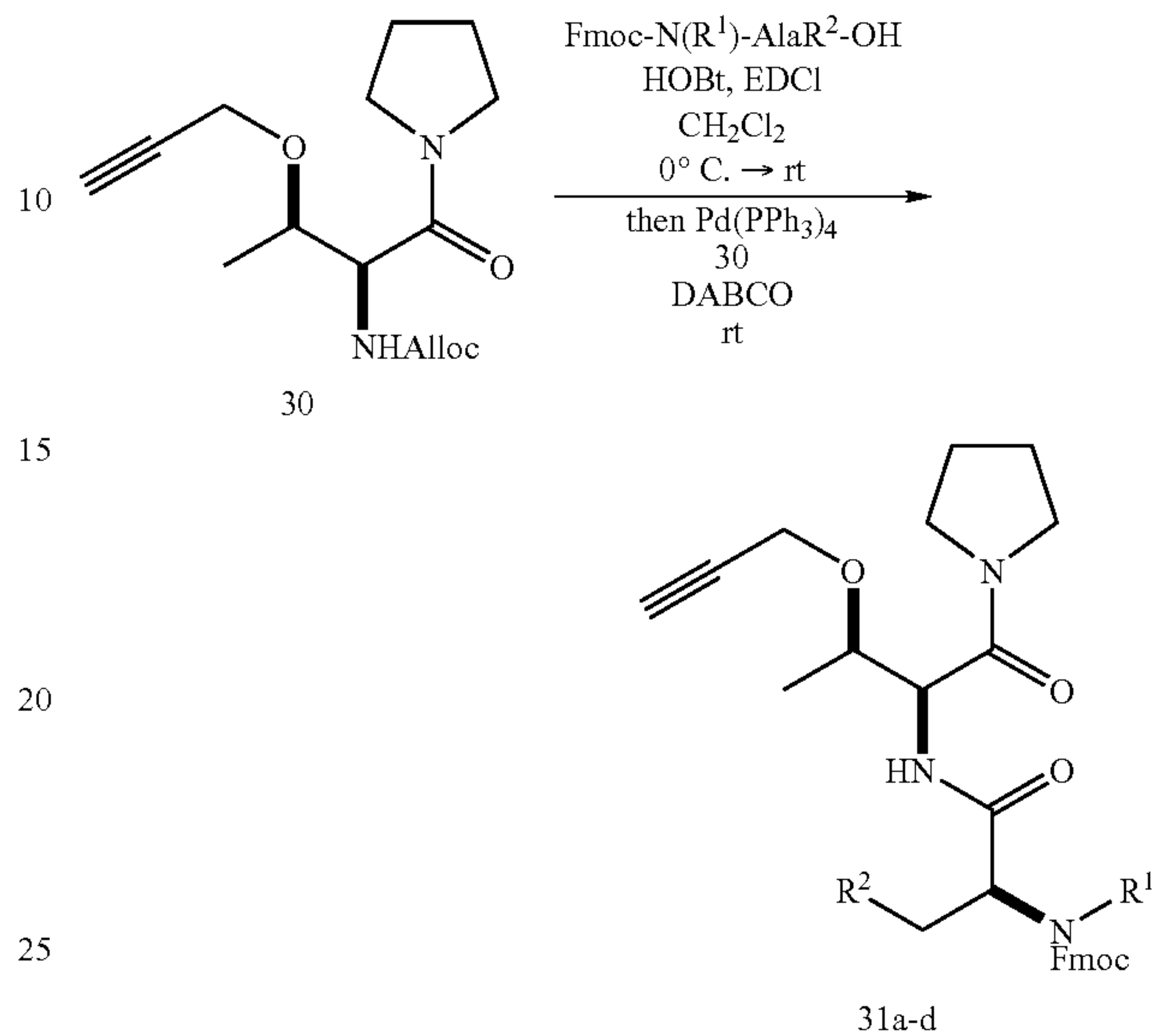
Scheme 11
