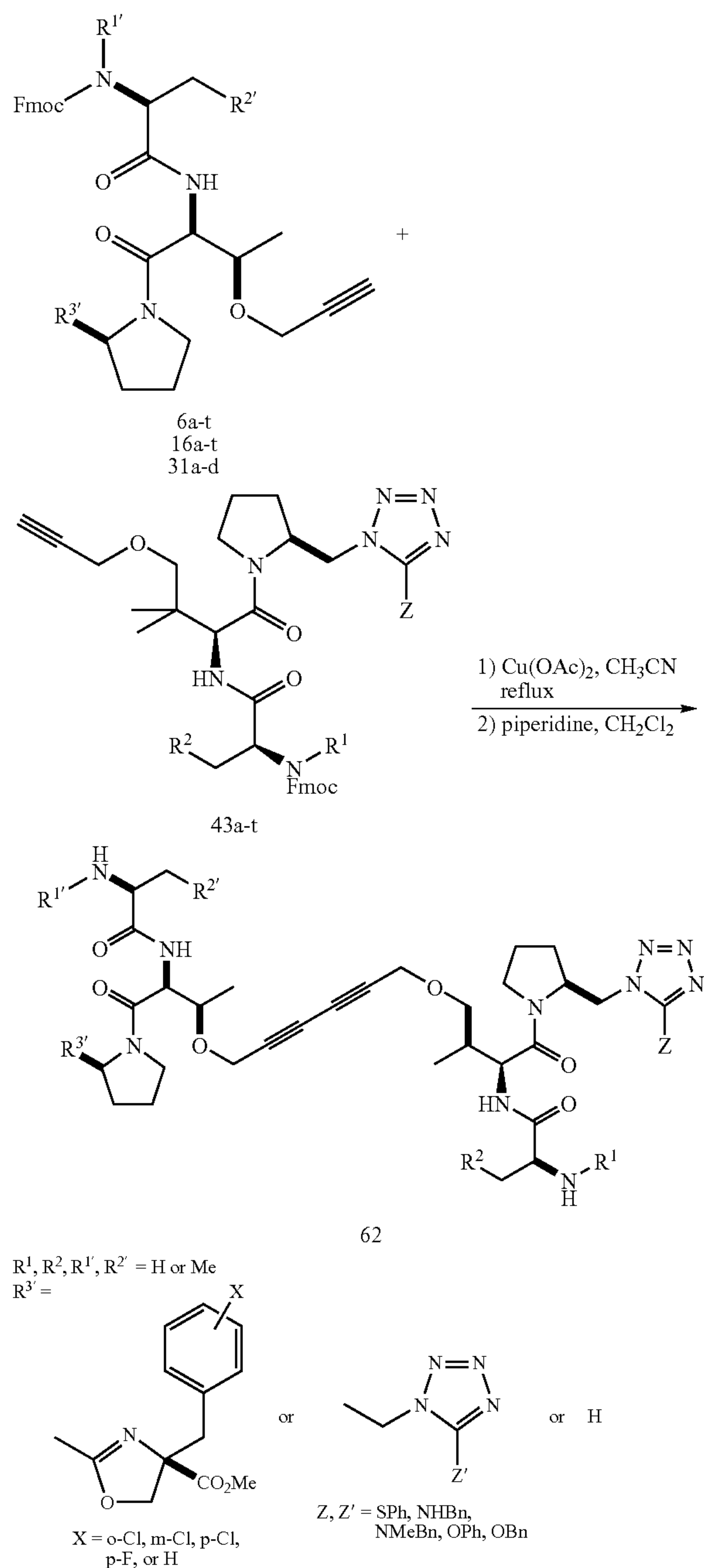
Scheme 17
