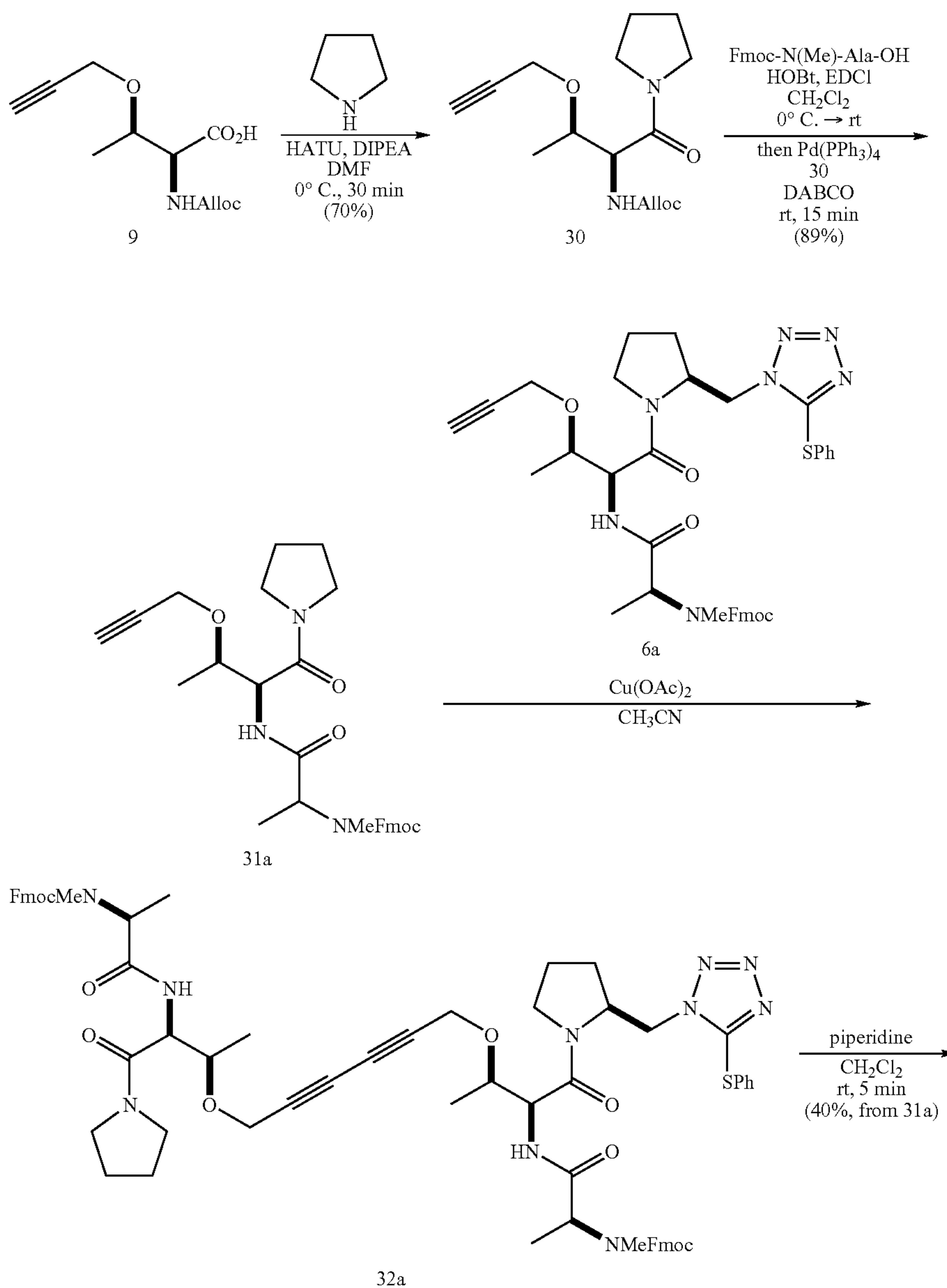
Scheme 8
