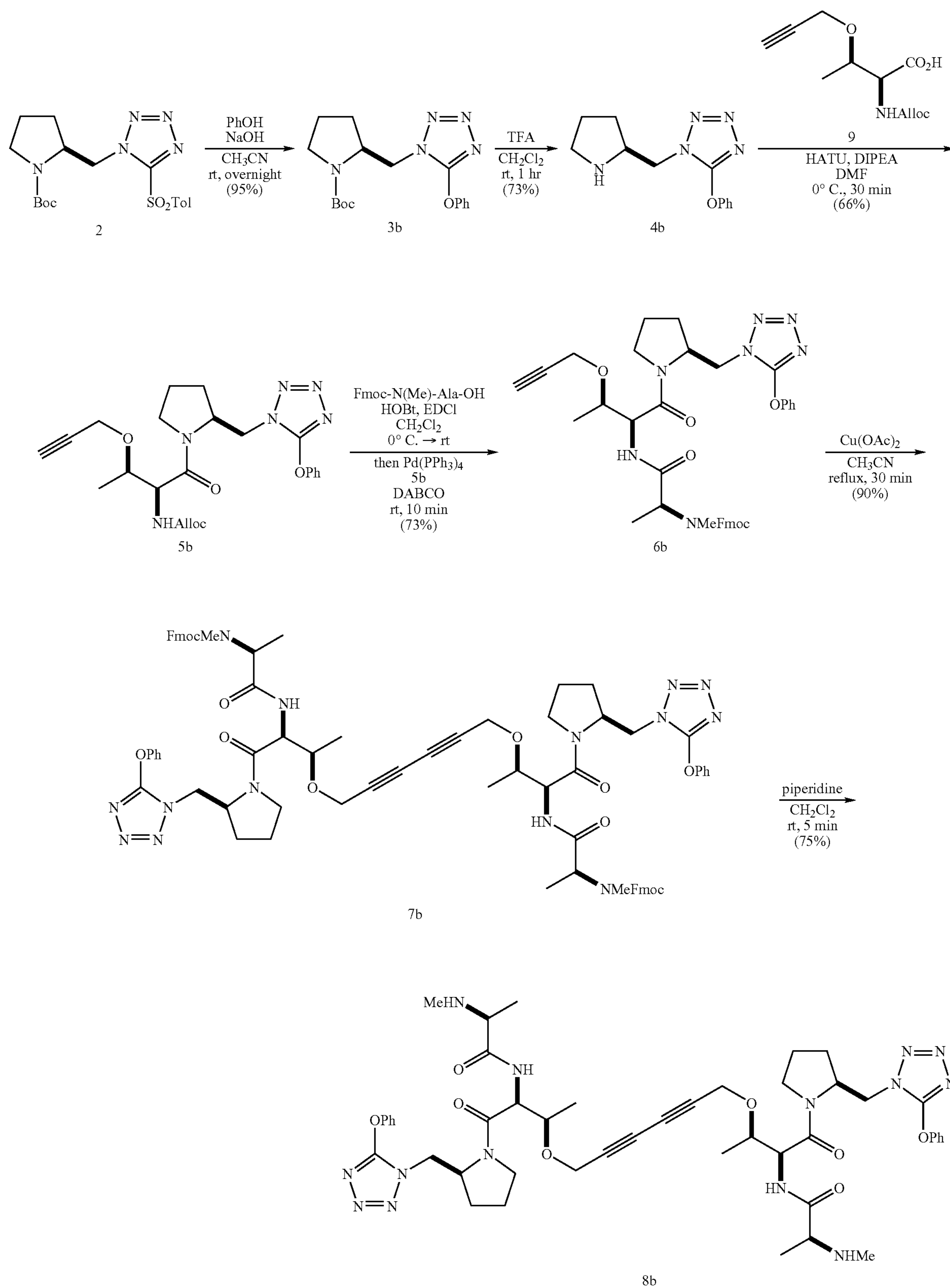
Scheme 2
