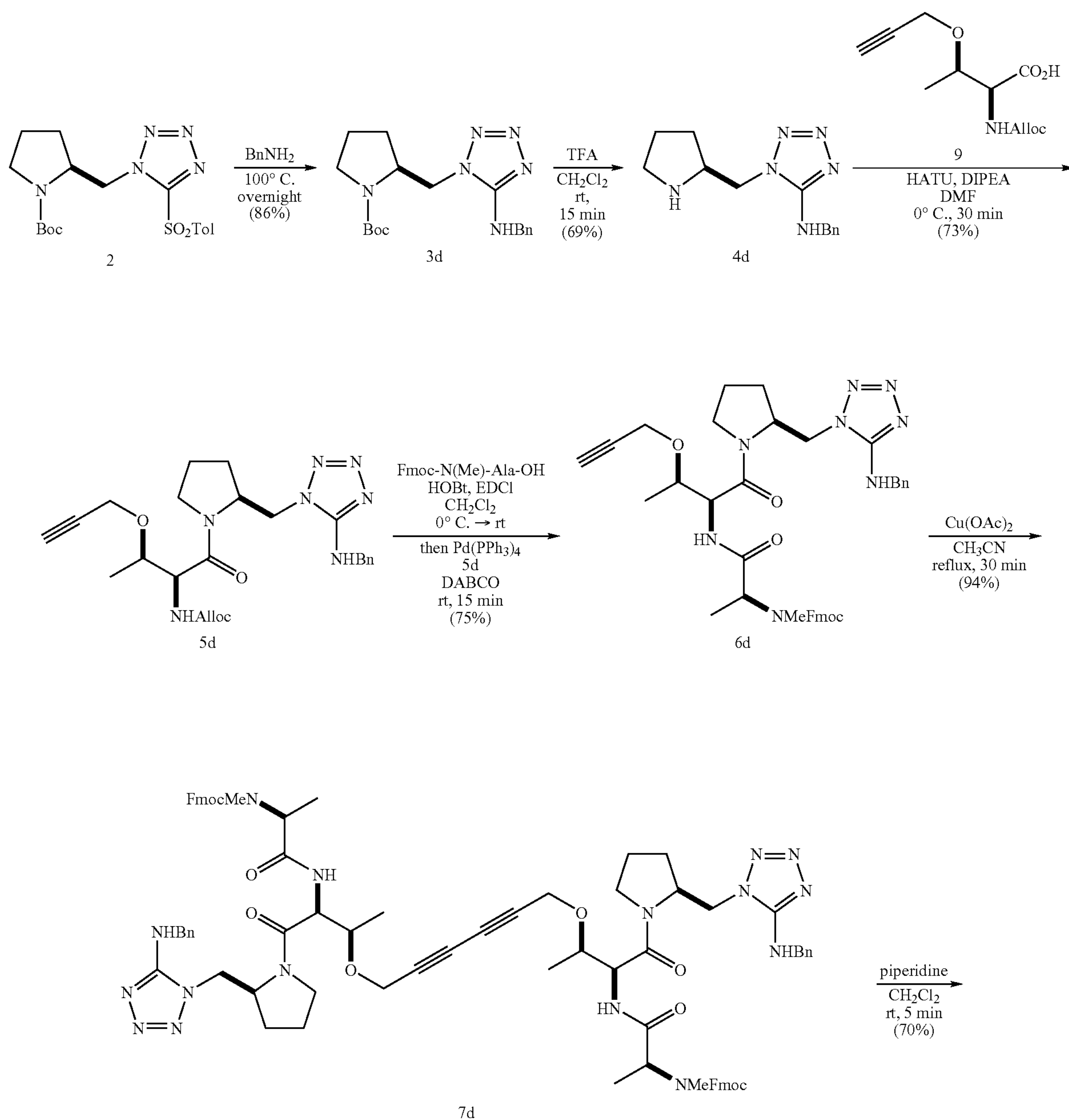
Scheme 4
