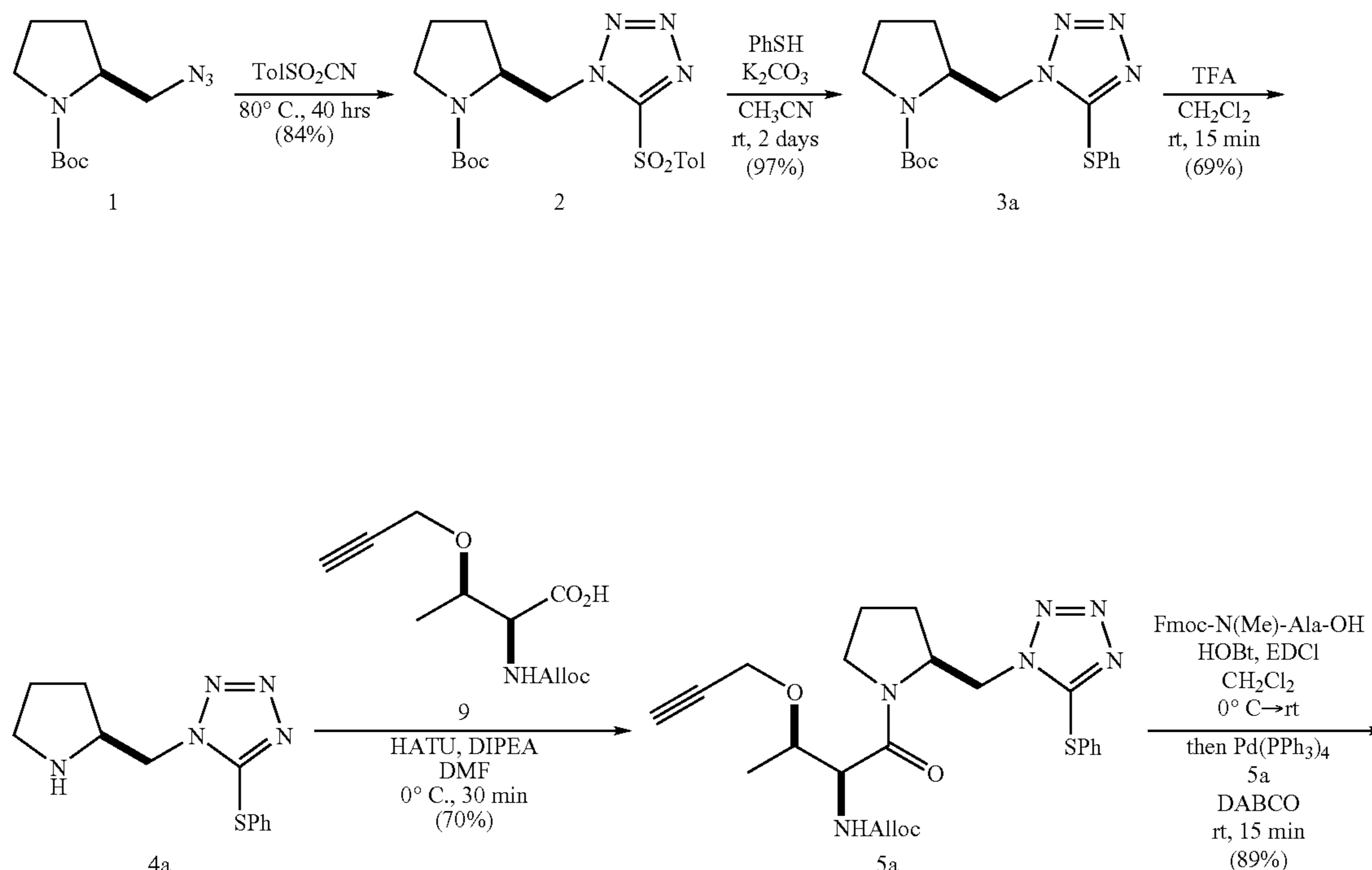
Scheme 1
