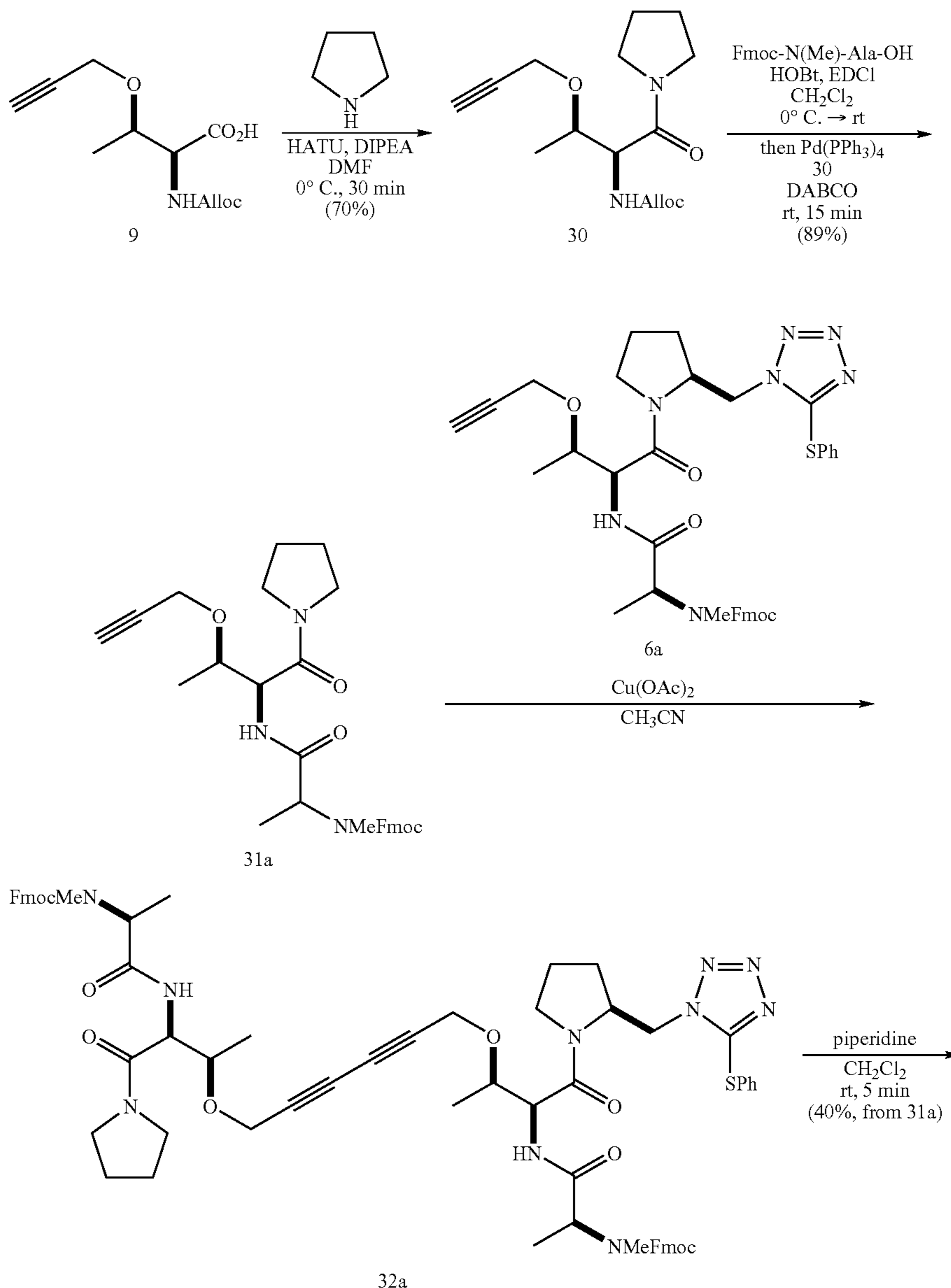
Scheme 8
