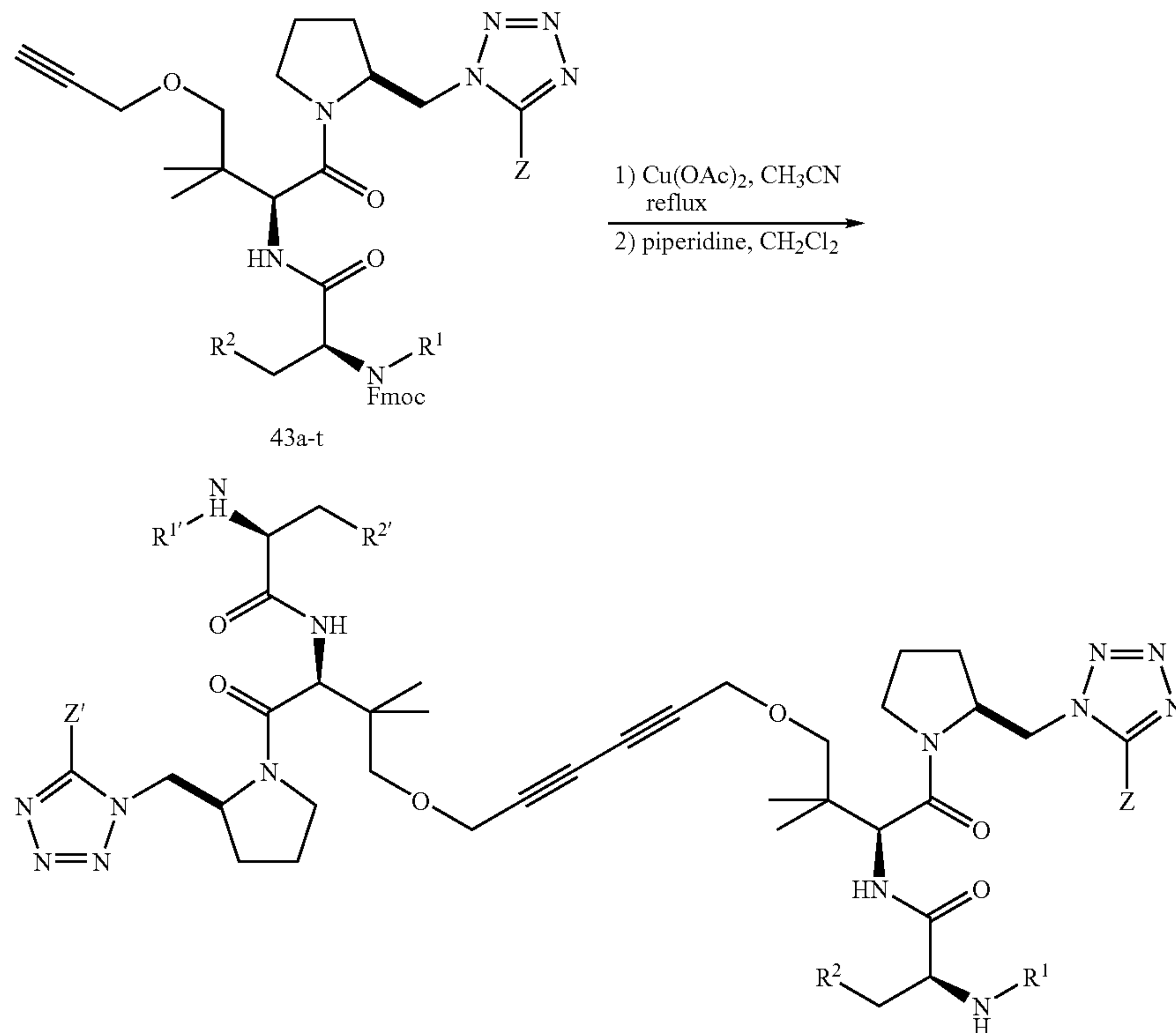
Scheme 16
