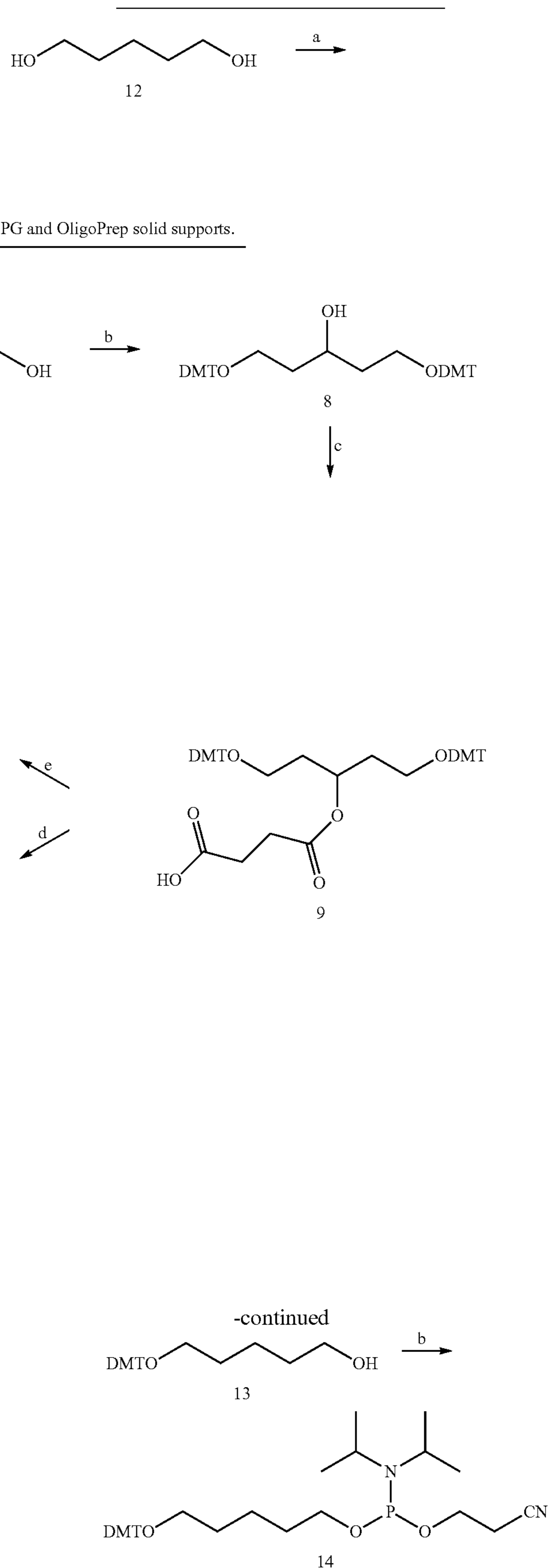
Scheme 3. Synthesis of pentanediol phosphoramidite.
