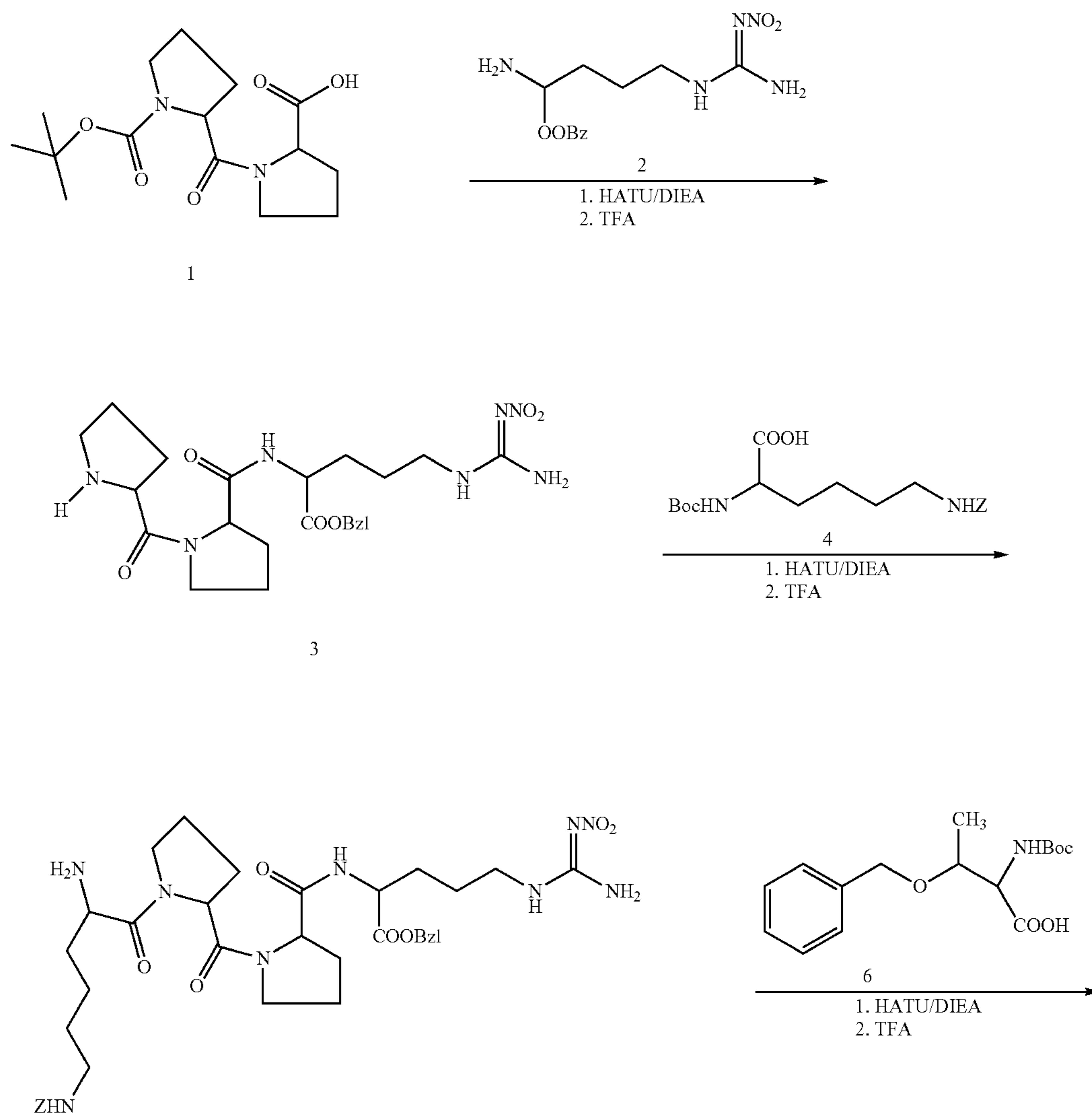
Scheme 2
