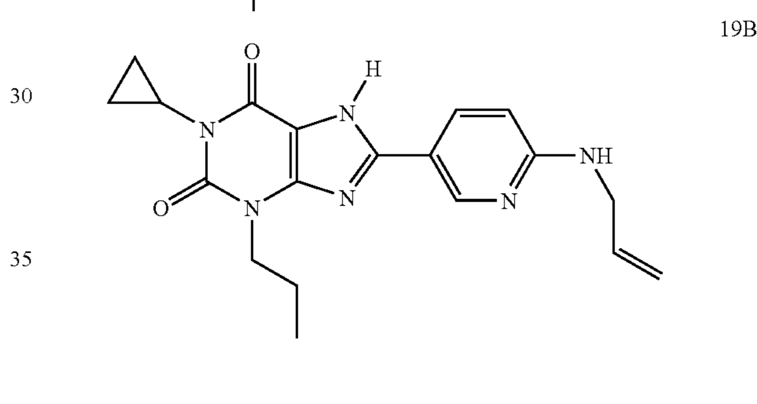
1B: 1-Cyclopropyl-3-propyl-8-[6-methylamino-3-pyridyl]xanthine
