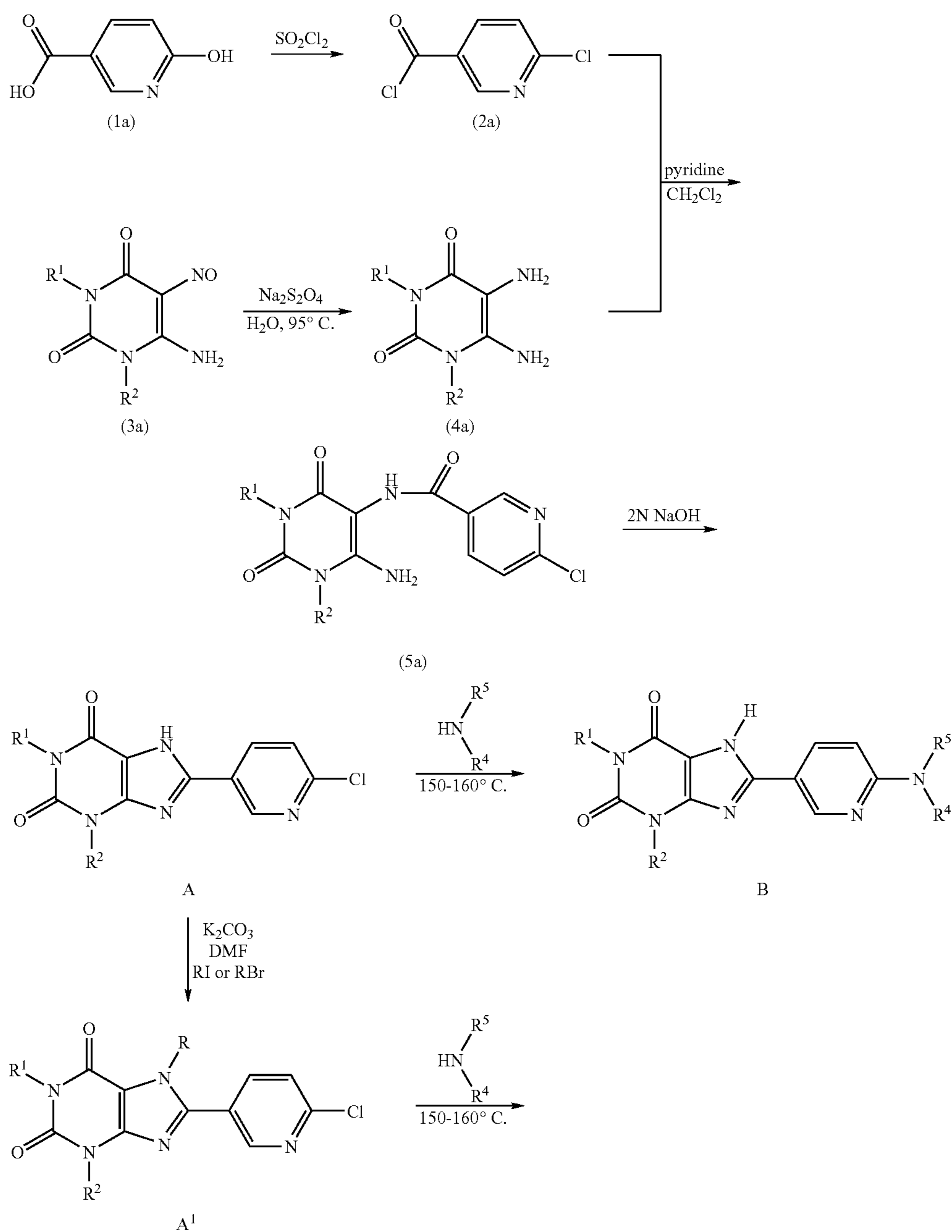
REACTION SCHEME 1
