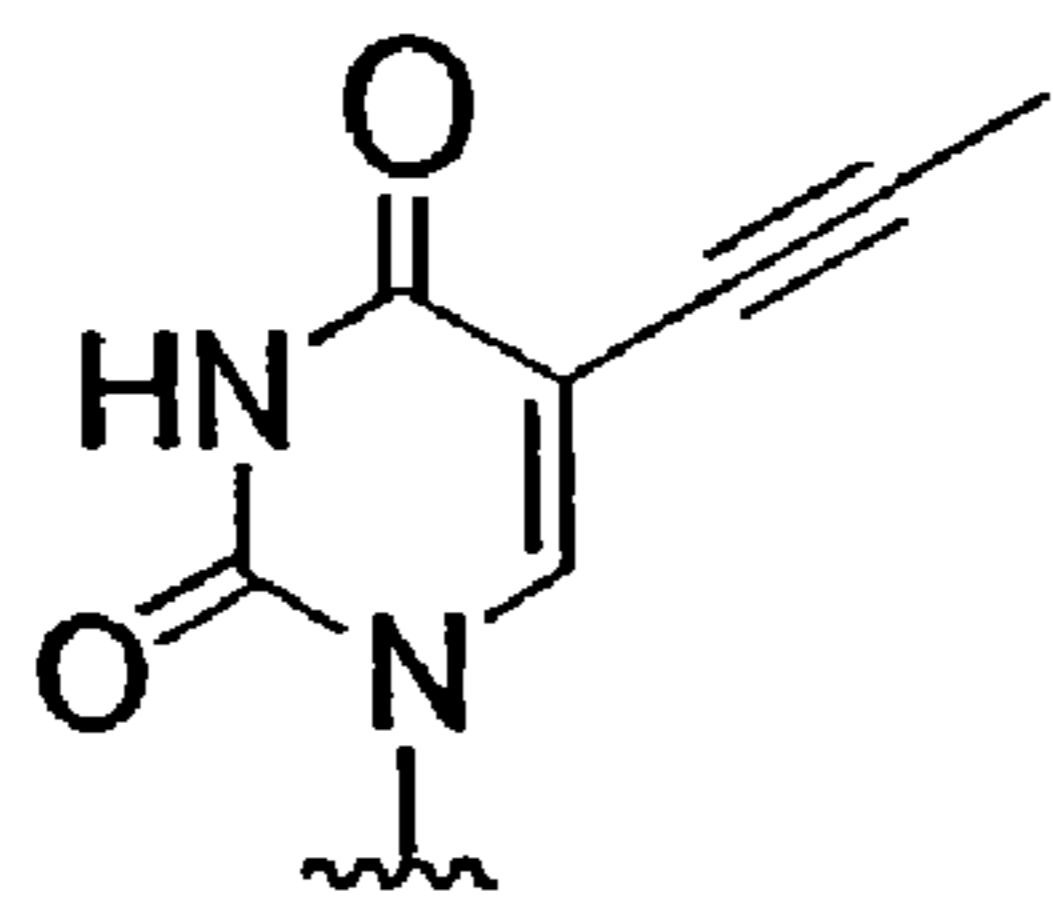
5-propynyl-U
