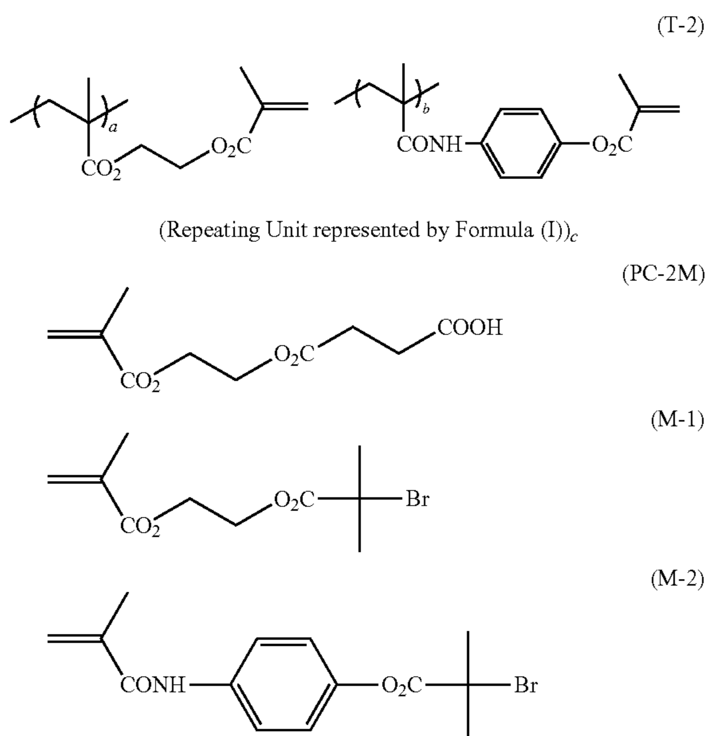
Synthesis Example 3, Binder Polymer (P-23)
