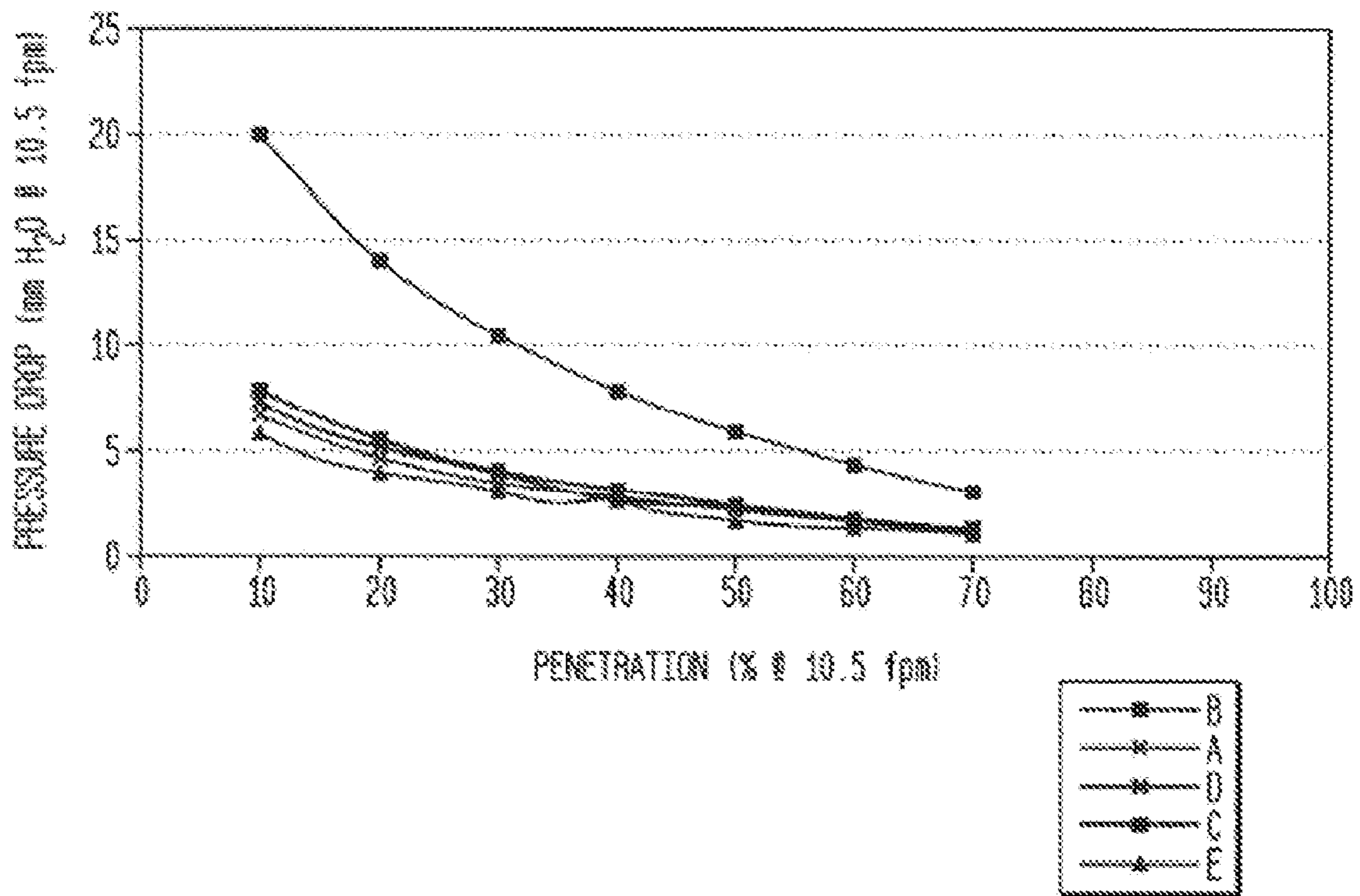
DISCHARGED DOP PENETRATION VERSUS PRESSURE DROP
