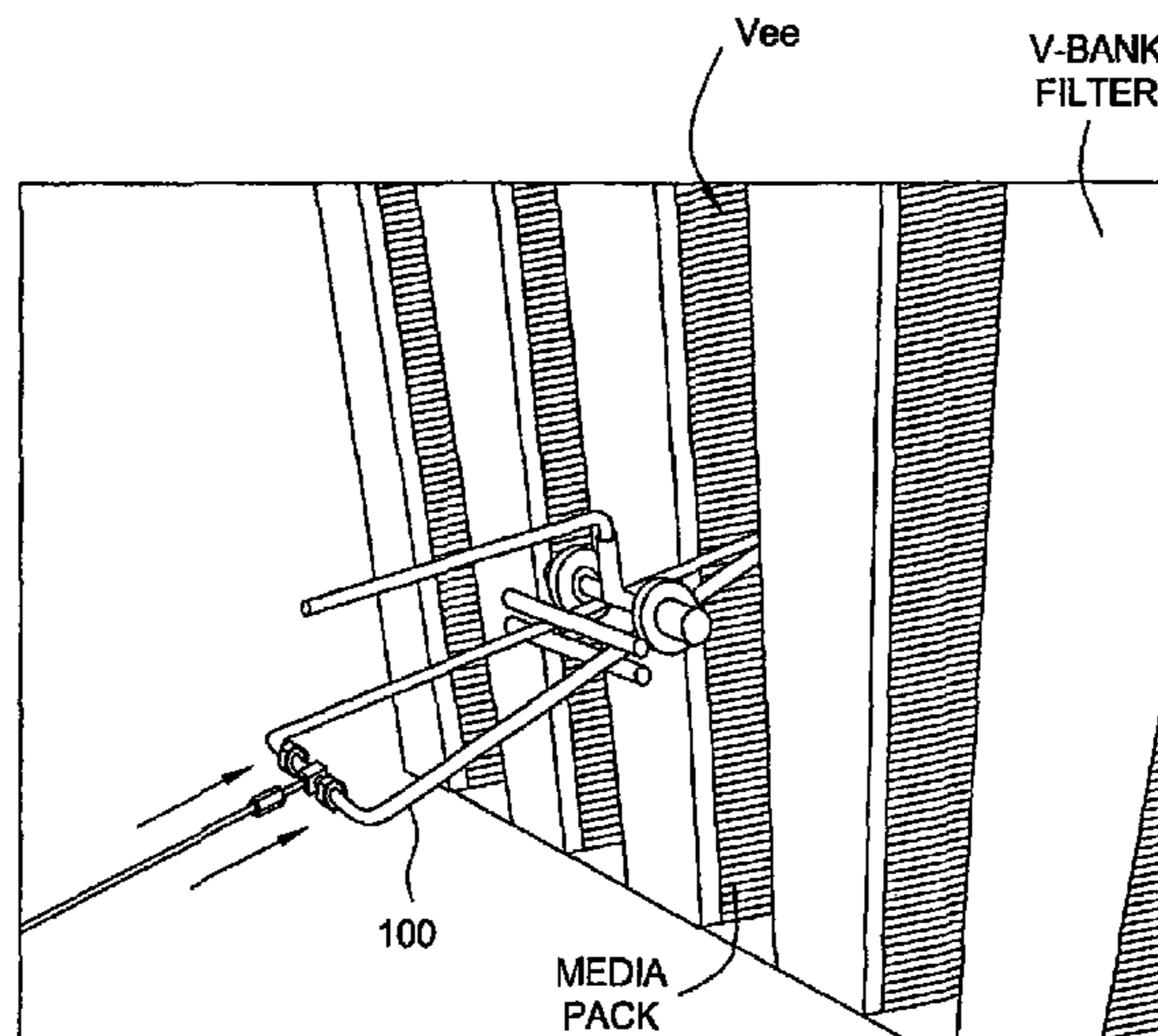
INSERTING PROBE
