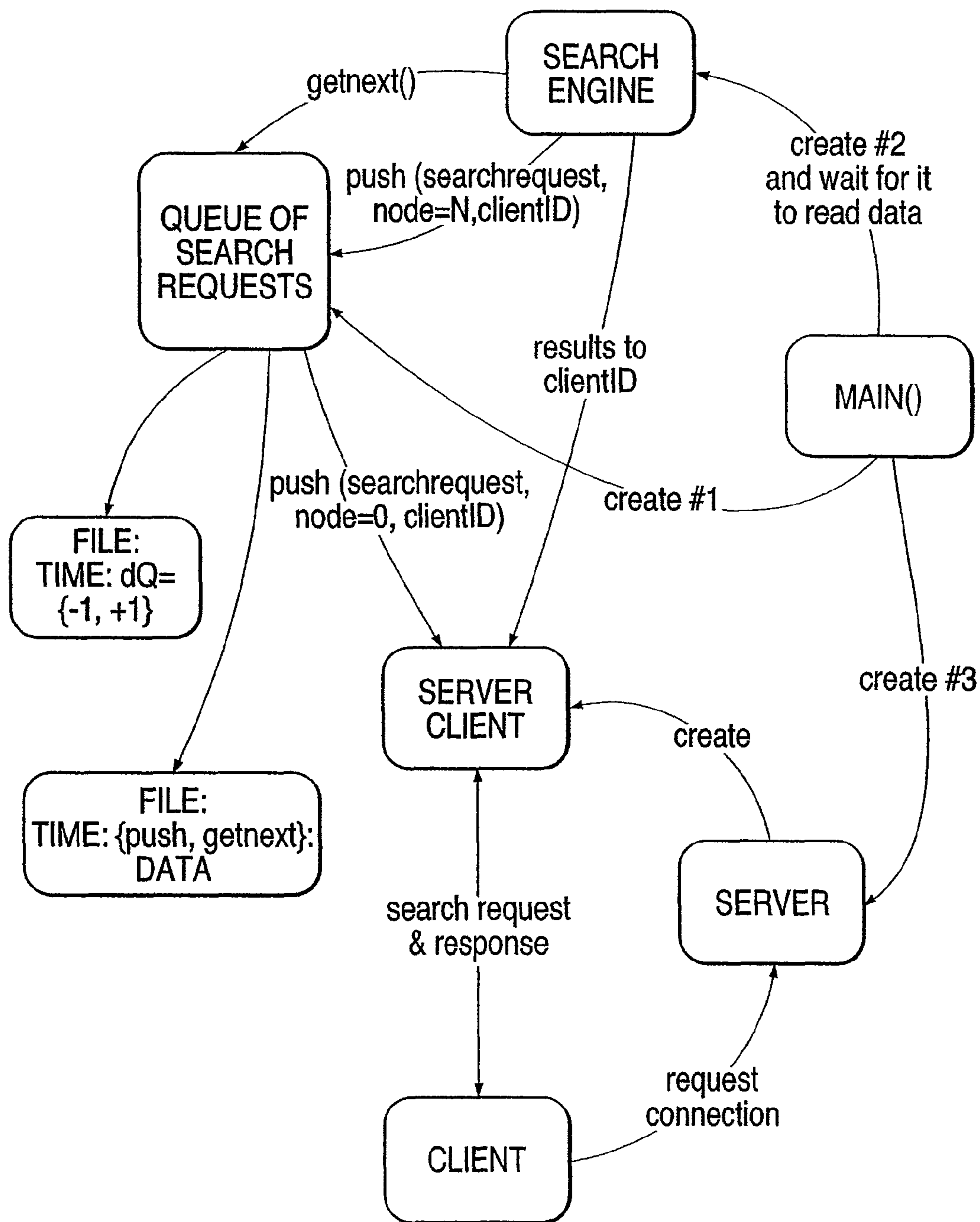
FIG. 3 SINGLE HOST SEARCH SERVER
