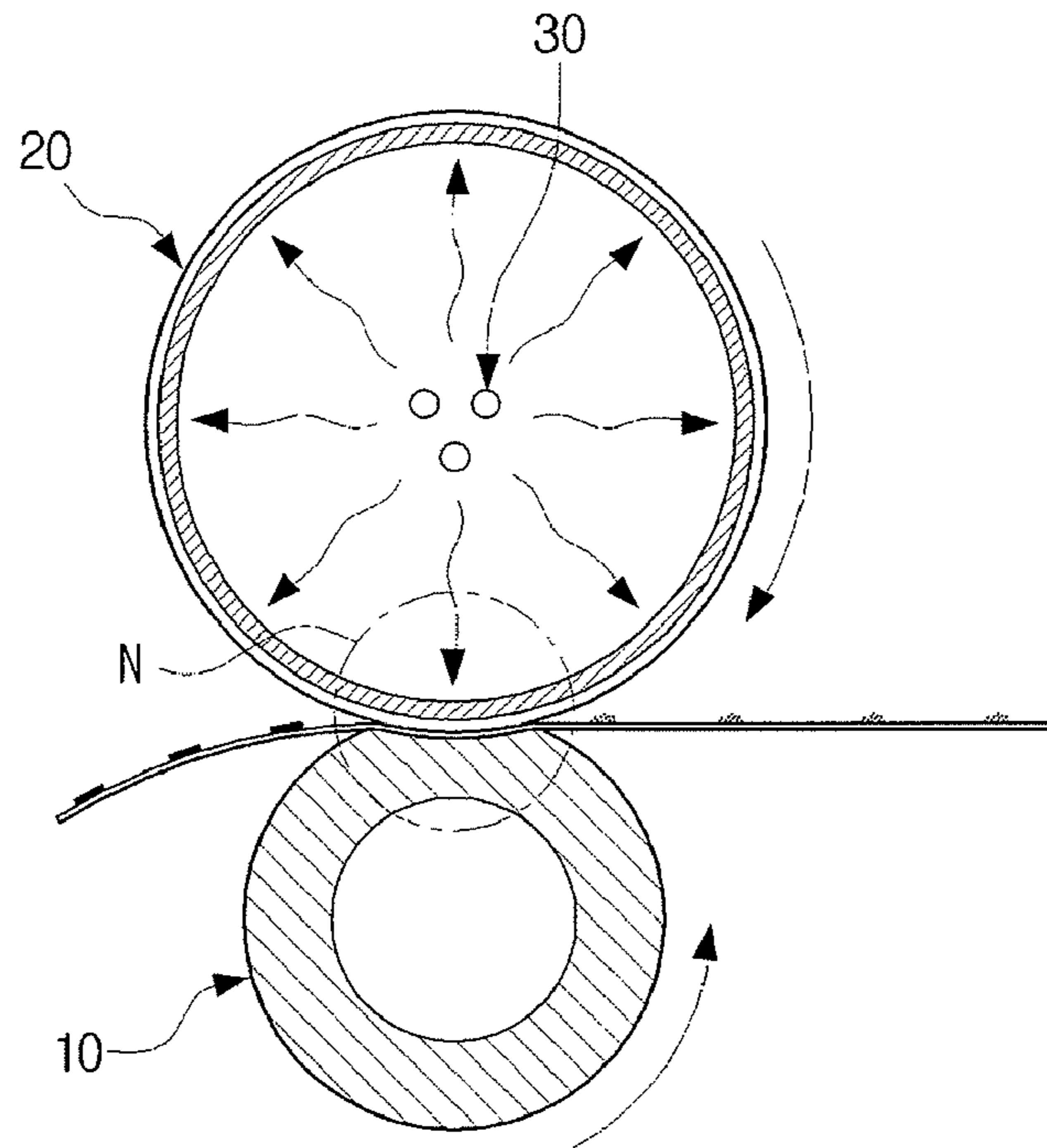
FIG. 1 (PRIOR ART)
