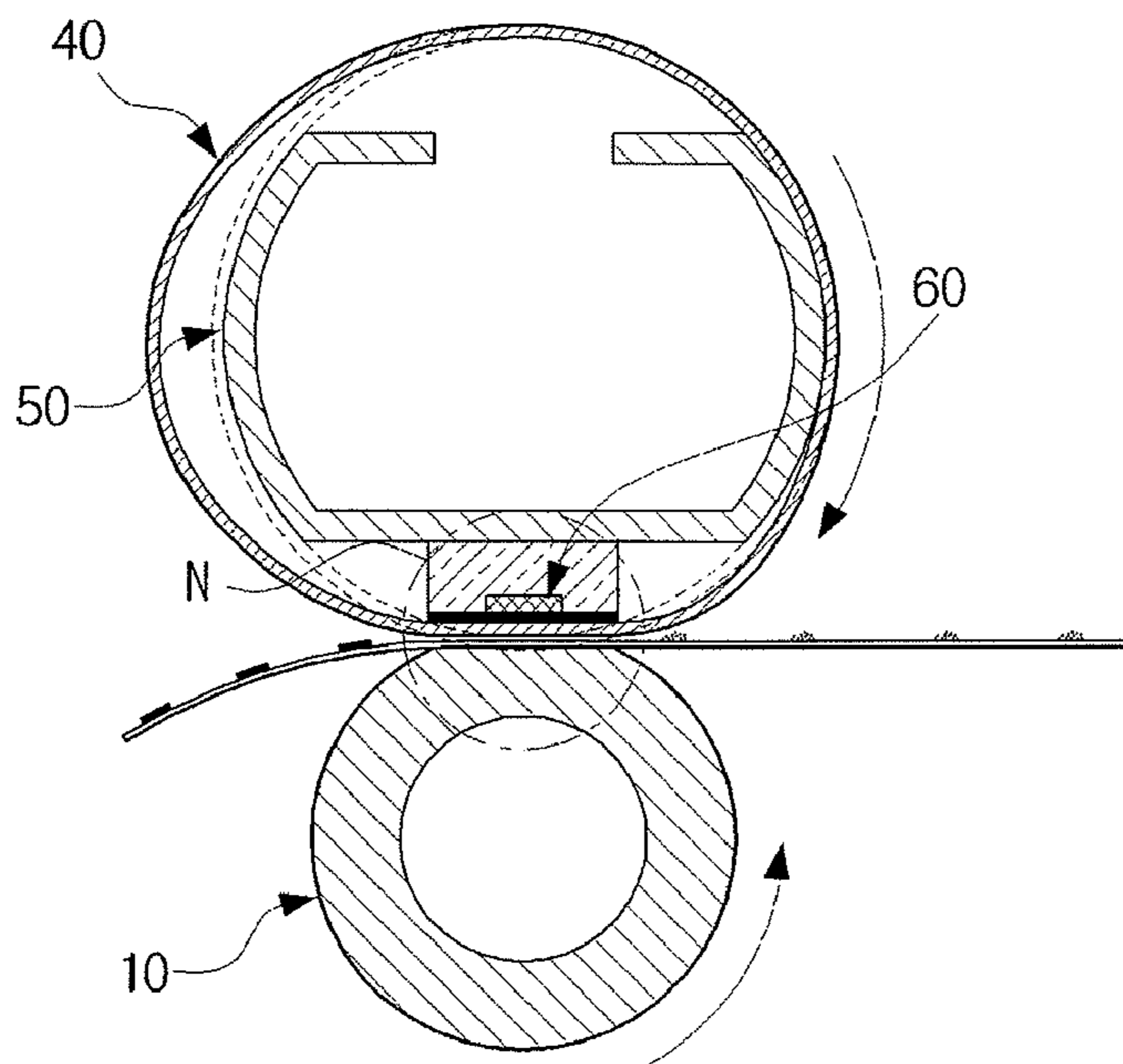
FIG. 2 (PRIOR ART)
