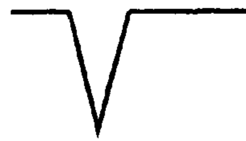
Less asymmetric Lineshape
