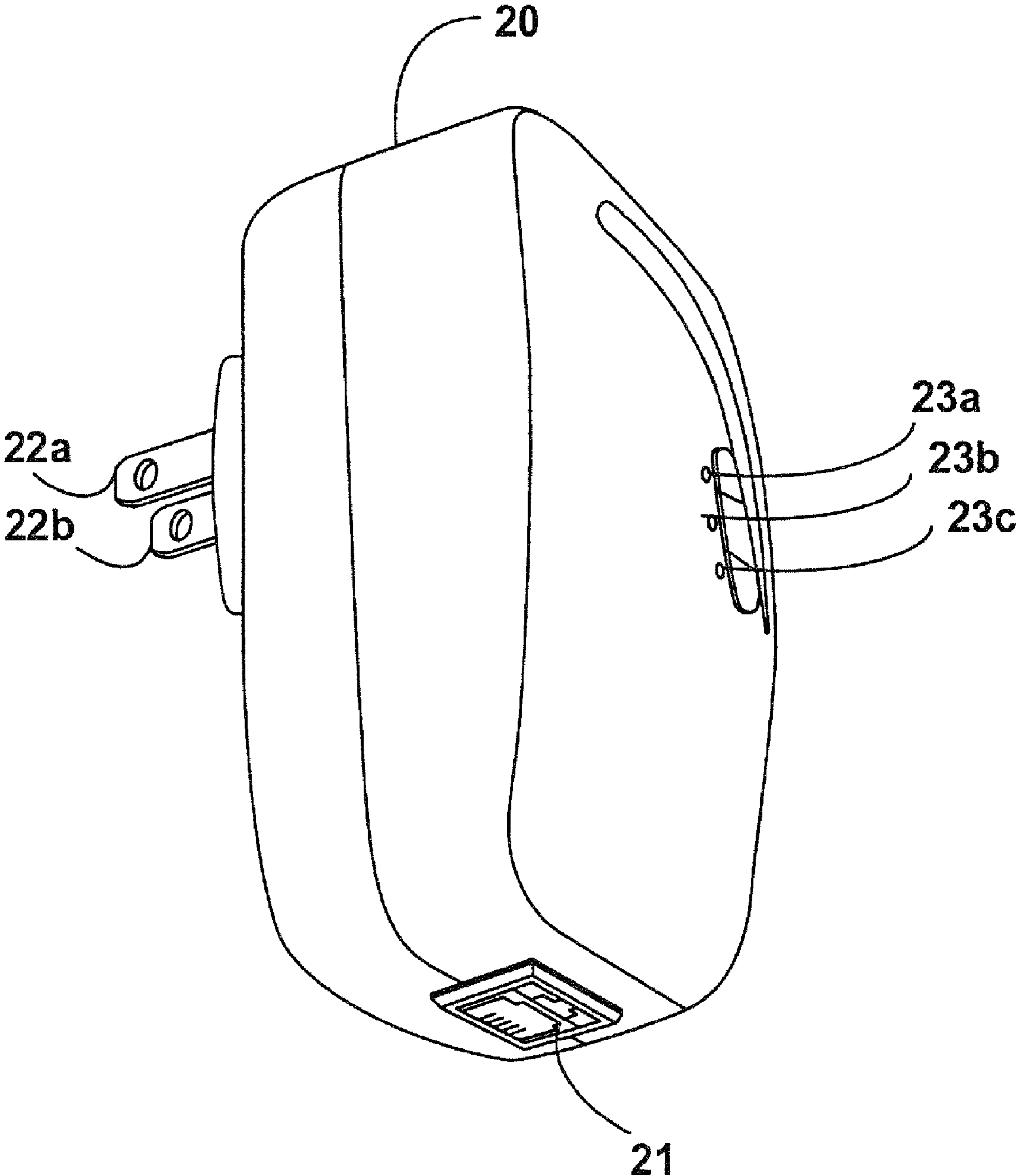
Figure 2 (Prior Art)
