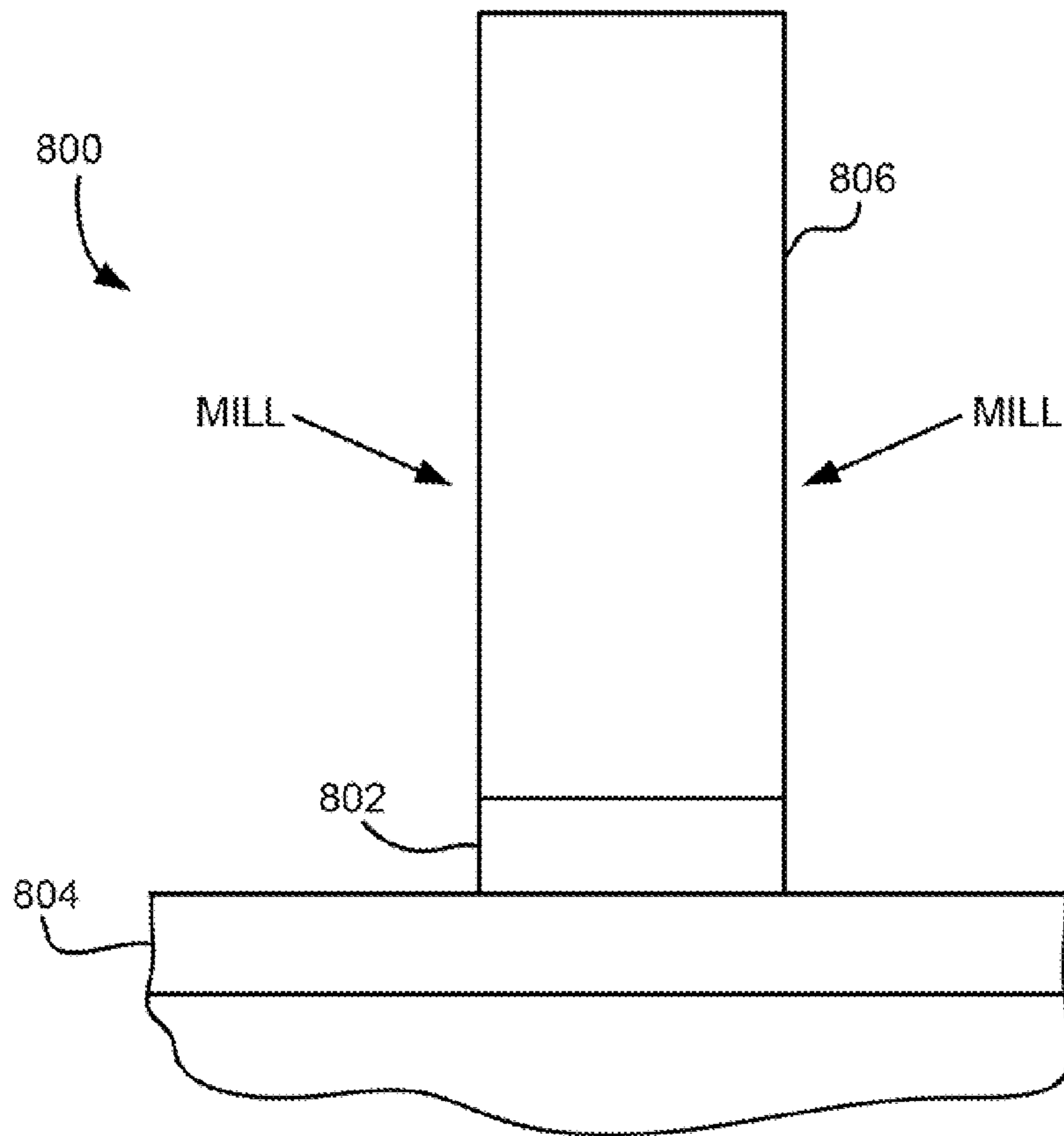
FIG. 8 PRIOR ART
