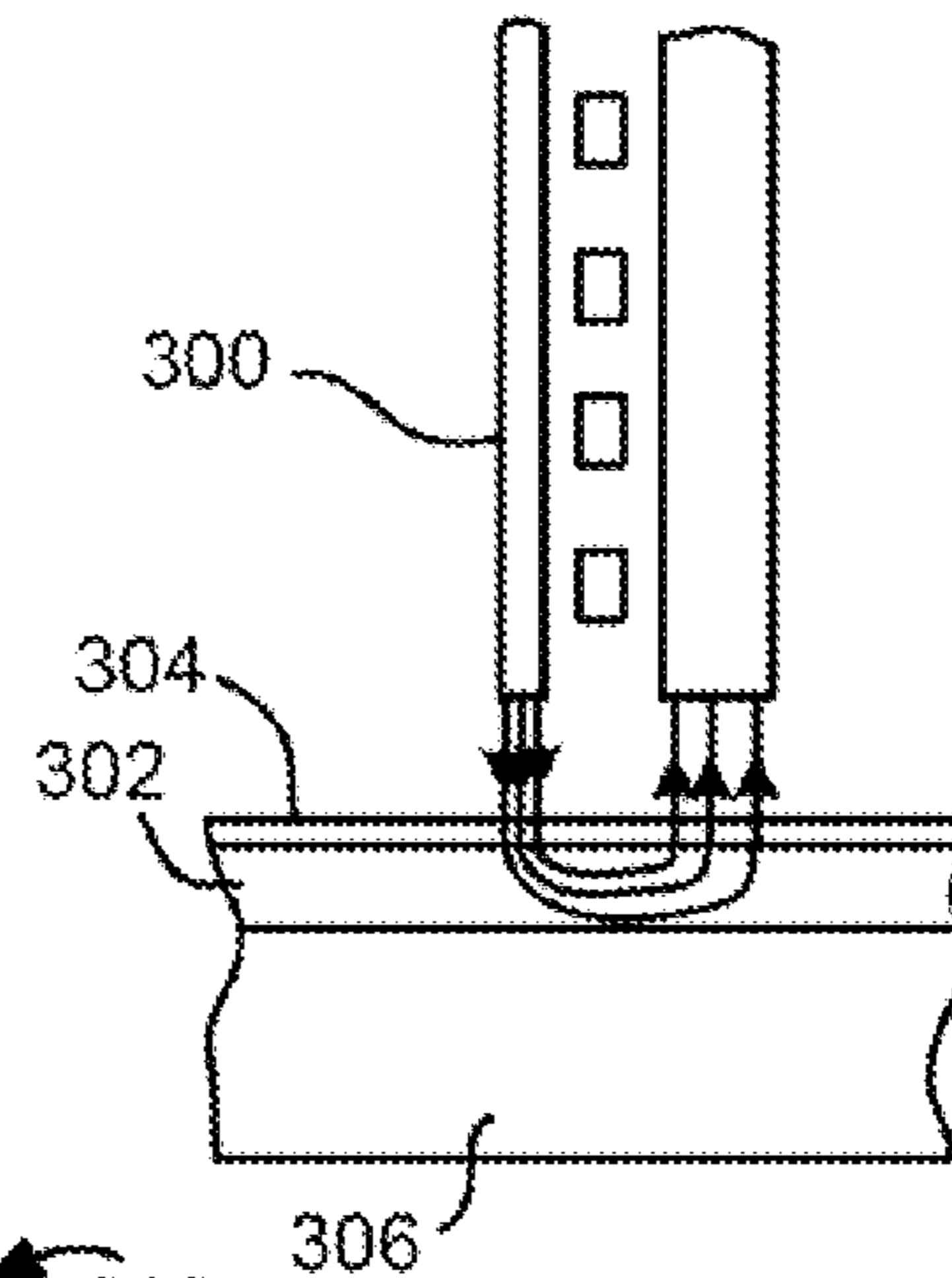
FIG. 4 PRIOR ART
