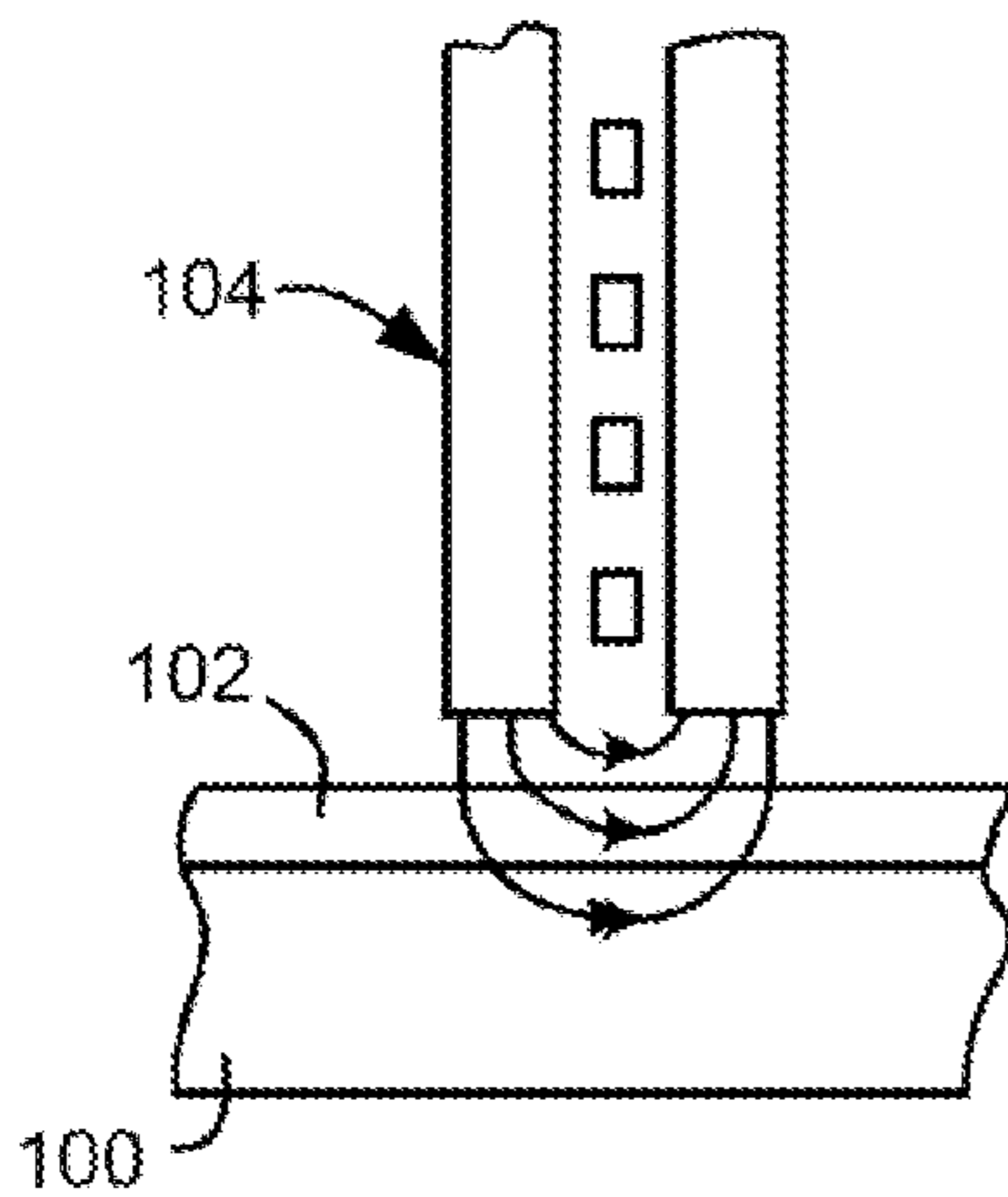
FIG. 2 PRIOR ART
