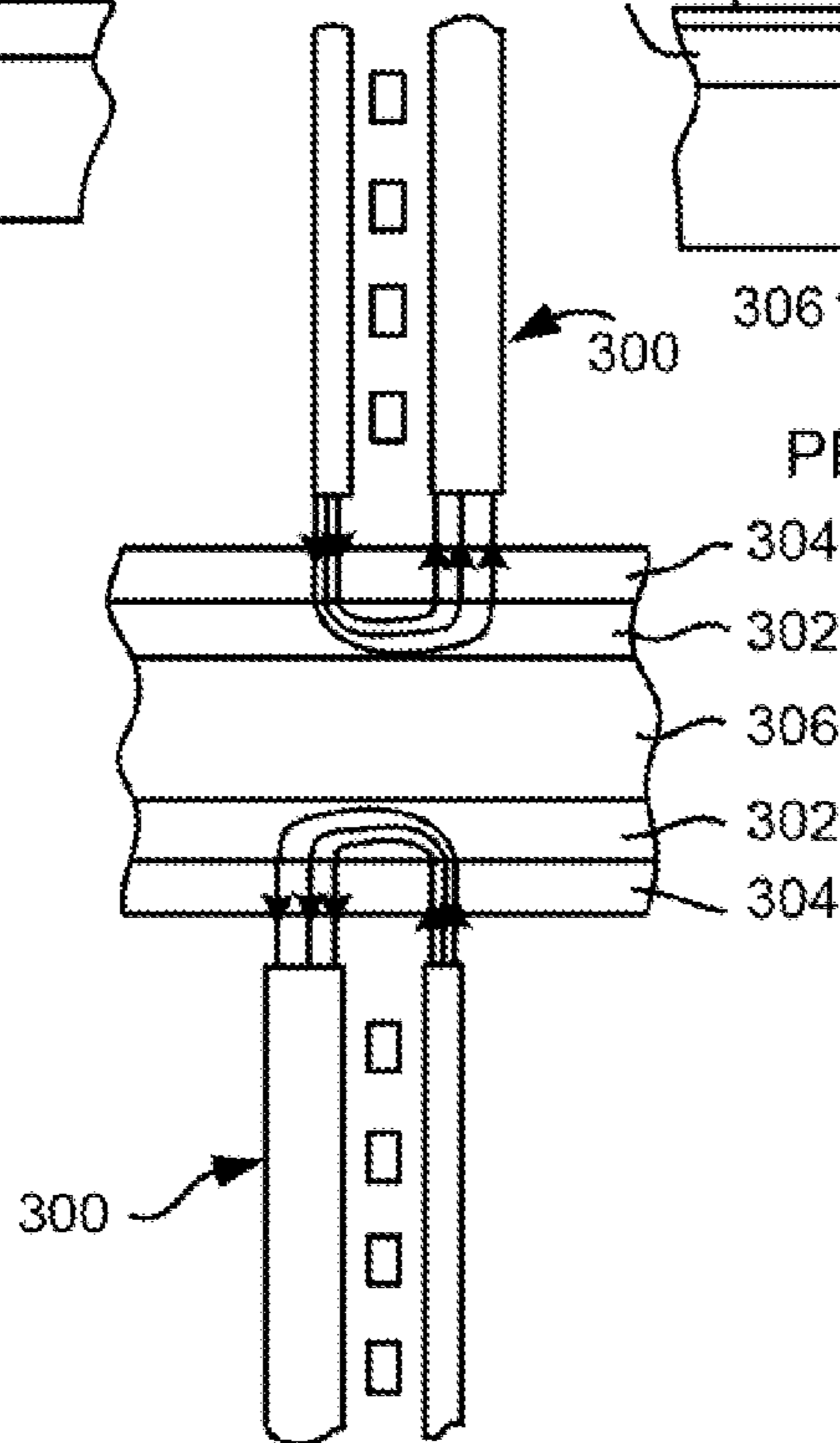
FIG. 5 PRIOR ART
