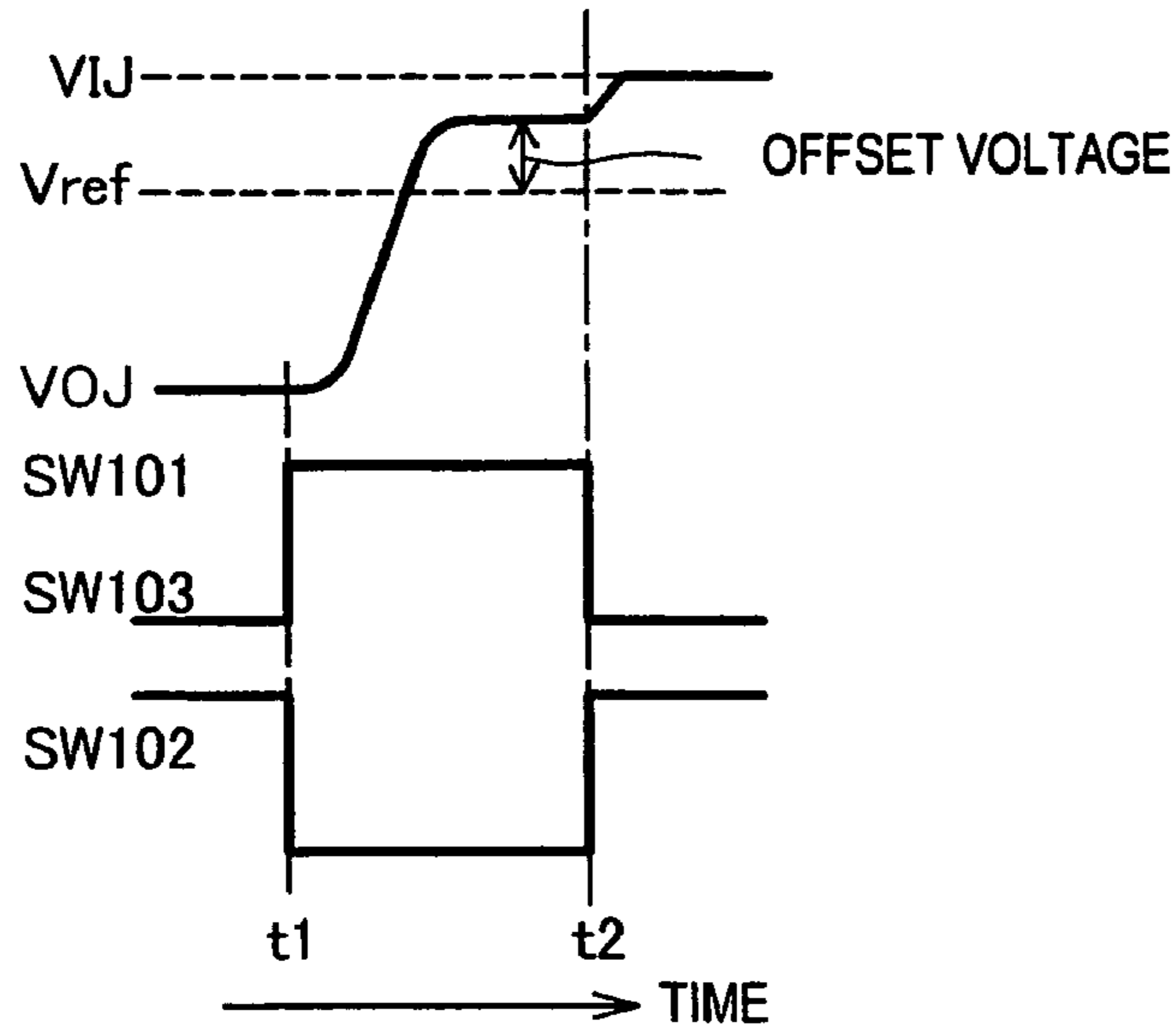
TIMING CHART OF OPERATIONALAMPLIFIER EQUIPPED WITH CONVENTIONAL OFFSET CANCEL FUNCTION
