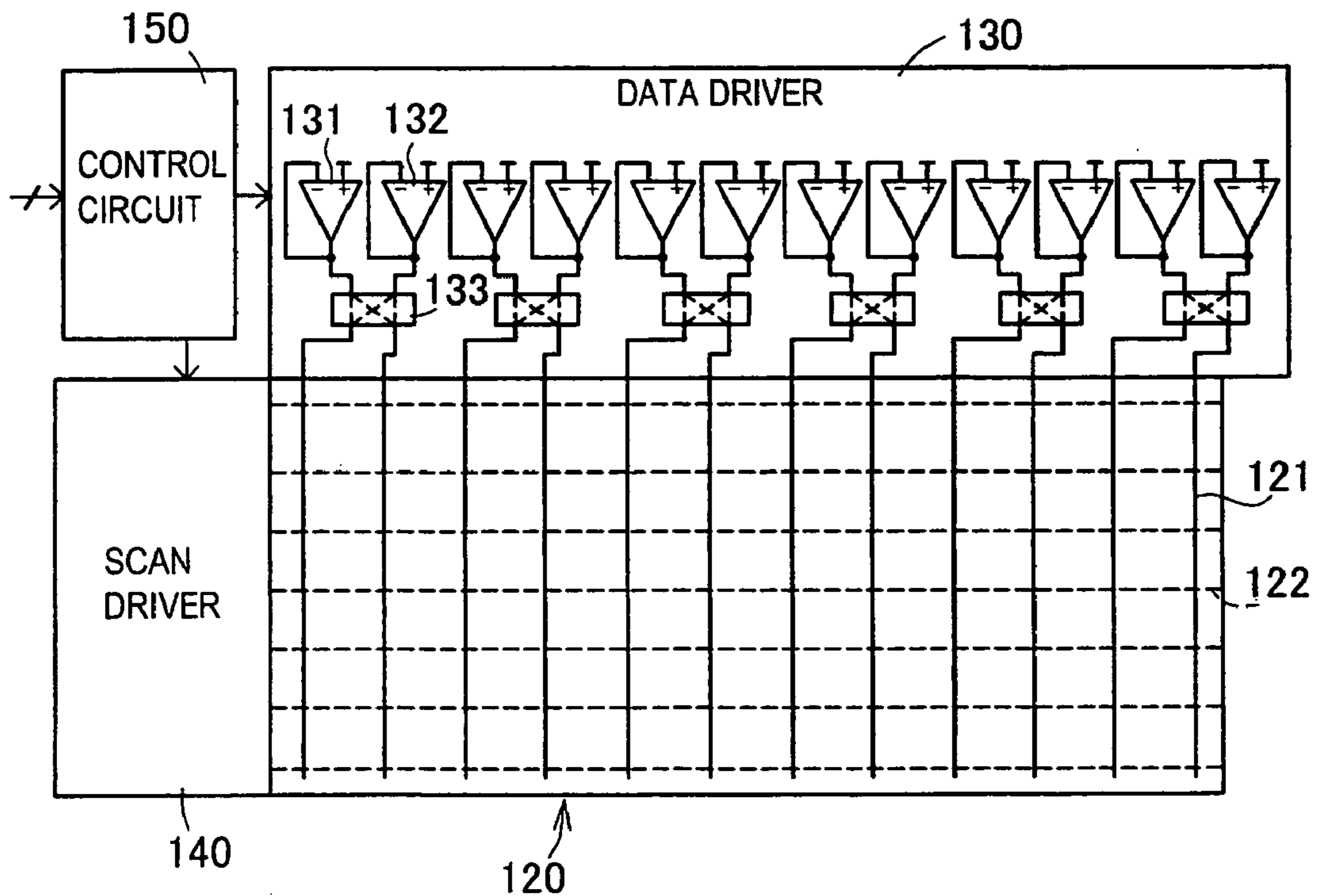
SCHEMATIC STRUCTURE OF LIQUID CRYSTAL DISPLAY DEVICE
