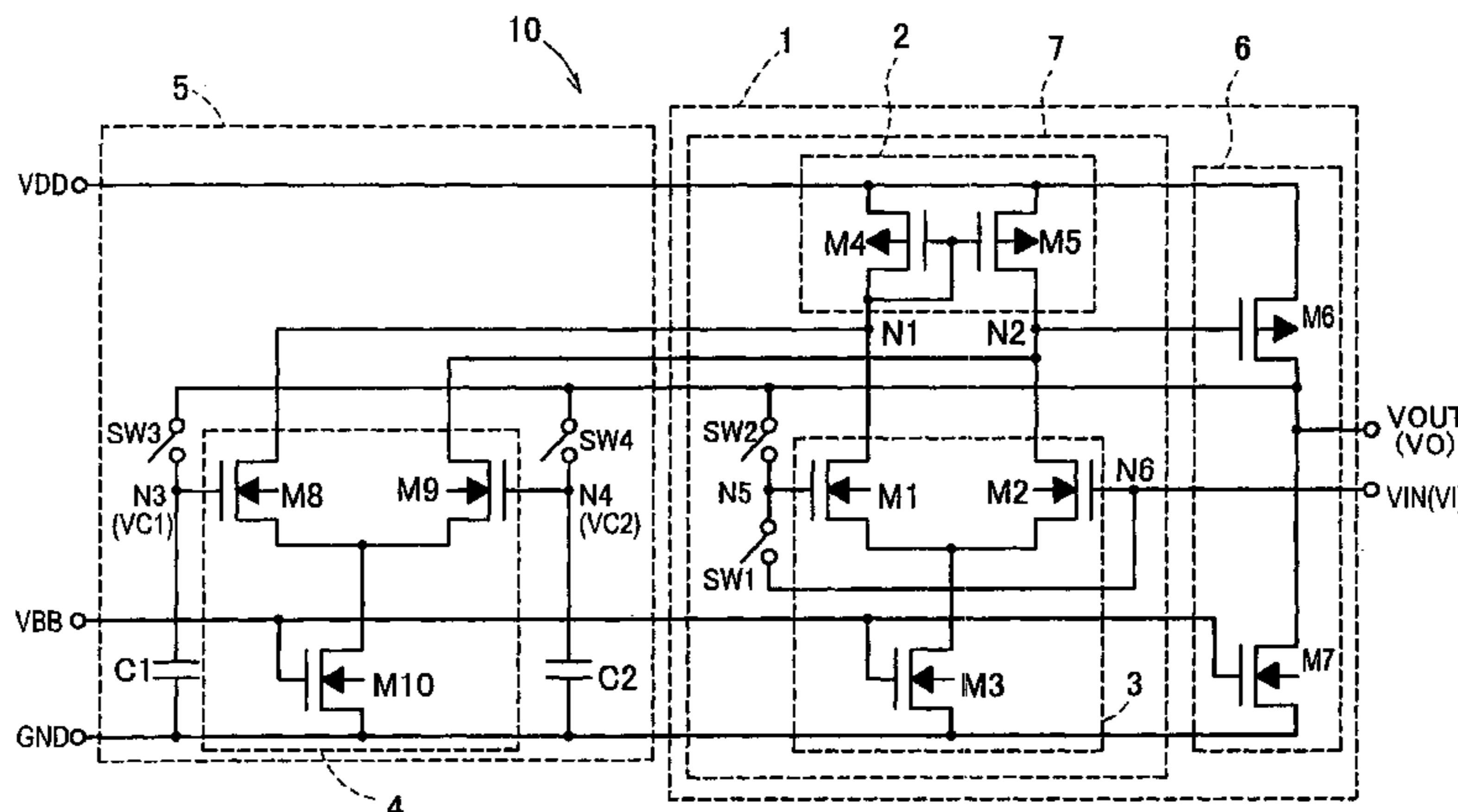
CIRCUIT DIAGRAM OF OPERATIONAL AMPLIFIER DIRECTED TO FIRST EXAMPLE OF FIRST EMBODIMENT
