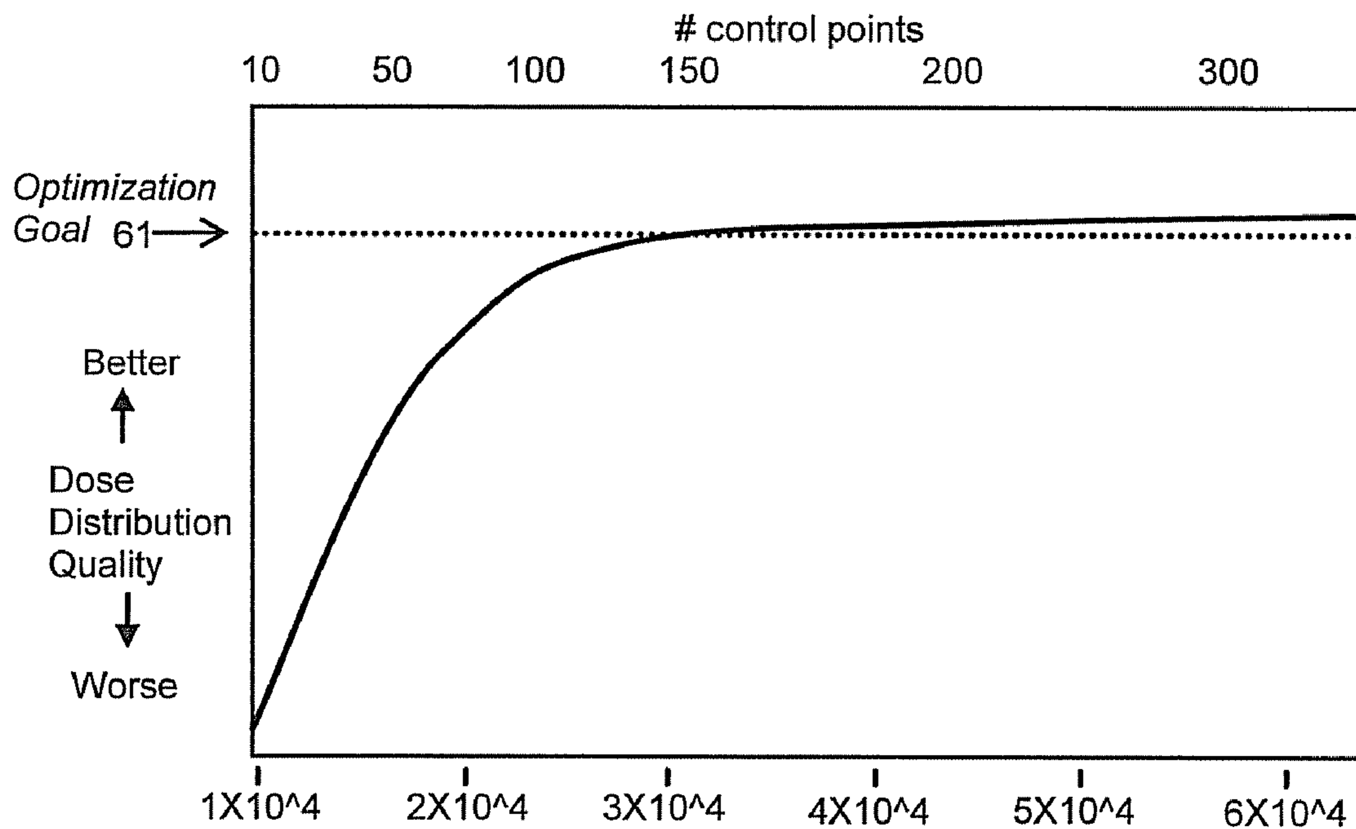
# OF ITERATIONS
