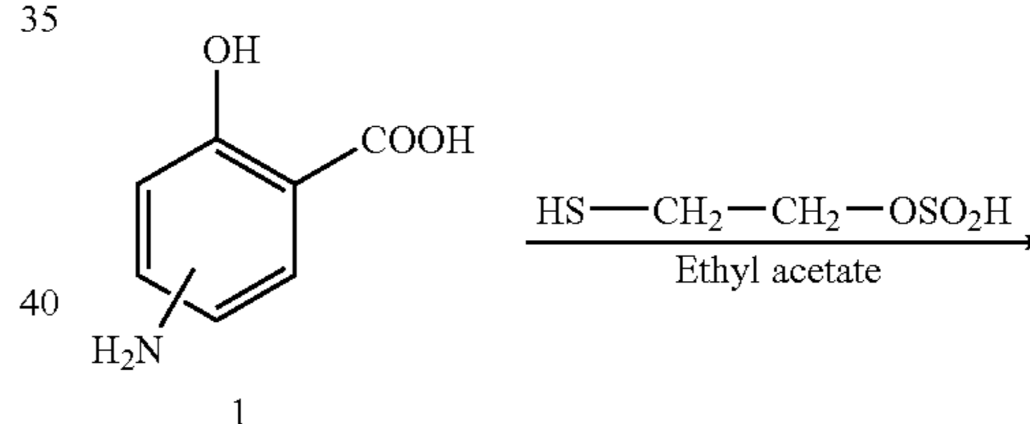
Synthesis of 4- or 5-tert-Butoxycarbonylamino-2-tert-butoxy-benzoic acid (2)
