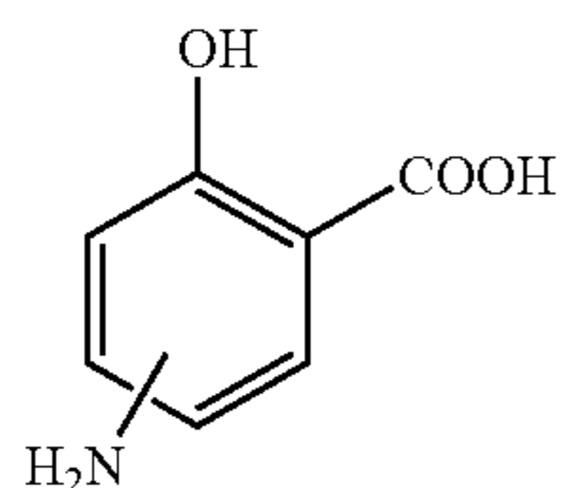
4- or 5-aminosalicylic acid
