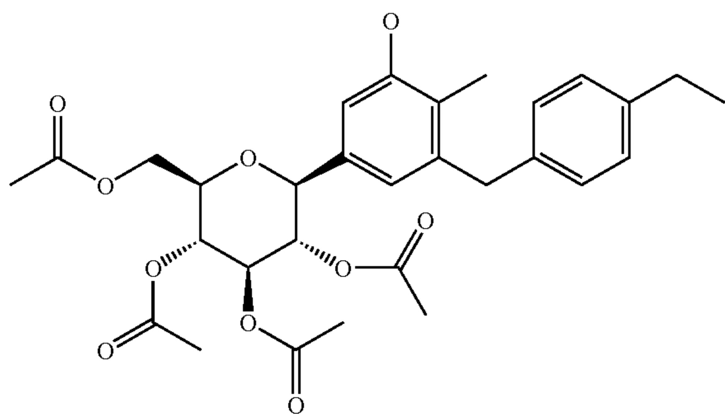
3-(4-Ethylbenzyl)-1-hydroxy-2-methyl-5-(2,3,4,6-tetra-O-acetyl-D-glucopyranos-1-yl)-benzene
