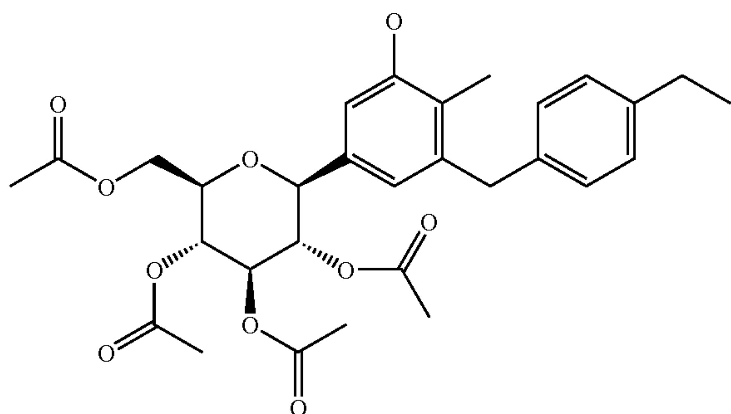
3-(4-Ethylbenzyl)-1-hydroxy-2-methyl-5-(2,3,4,6-tetra-O-acetyl-D-glucopyranos-1-yl)-benzene
