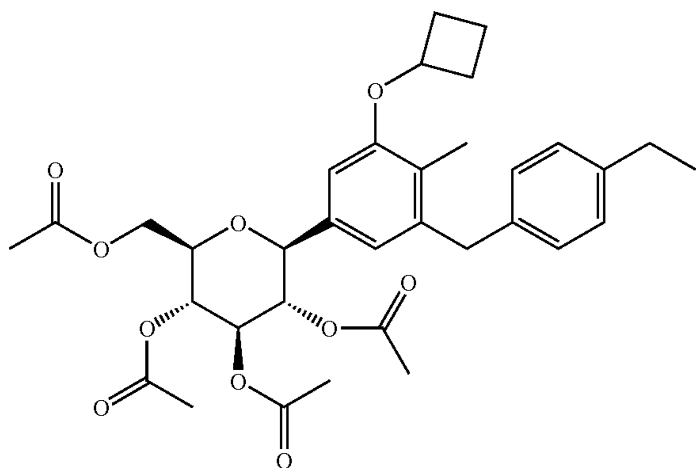
1-Cyclobutoxy-3-(4-ethylbenzyl)-2-methyl-5-(2,3,4,6-tetra-O-acetyl-D-glucopyranos-1-yl)-benzene
