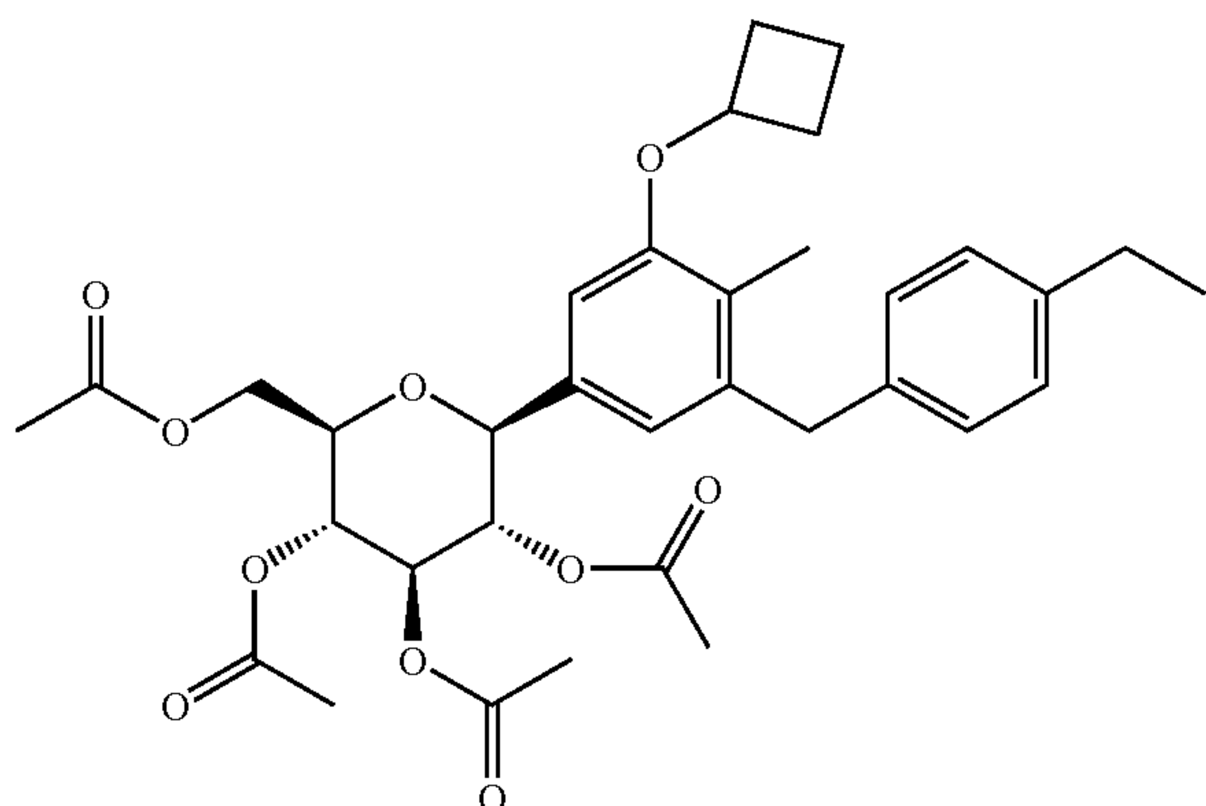
1-Cyclobutoxy-3-(4-ethylbenzyl)-2-methyl-5-(2,3,4,6-tetra-O-acetyl-D-glucopyranos-1-yl)-benzene
