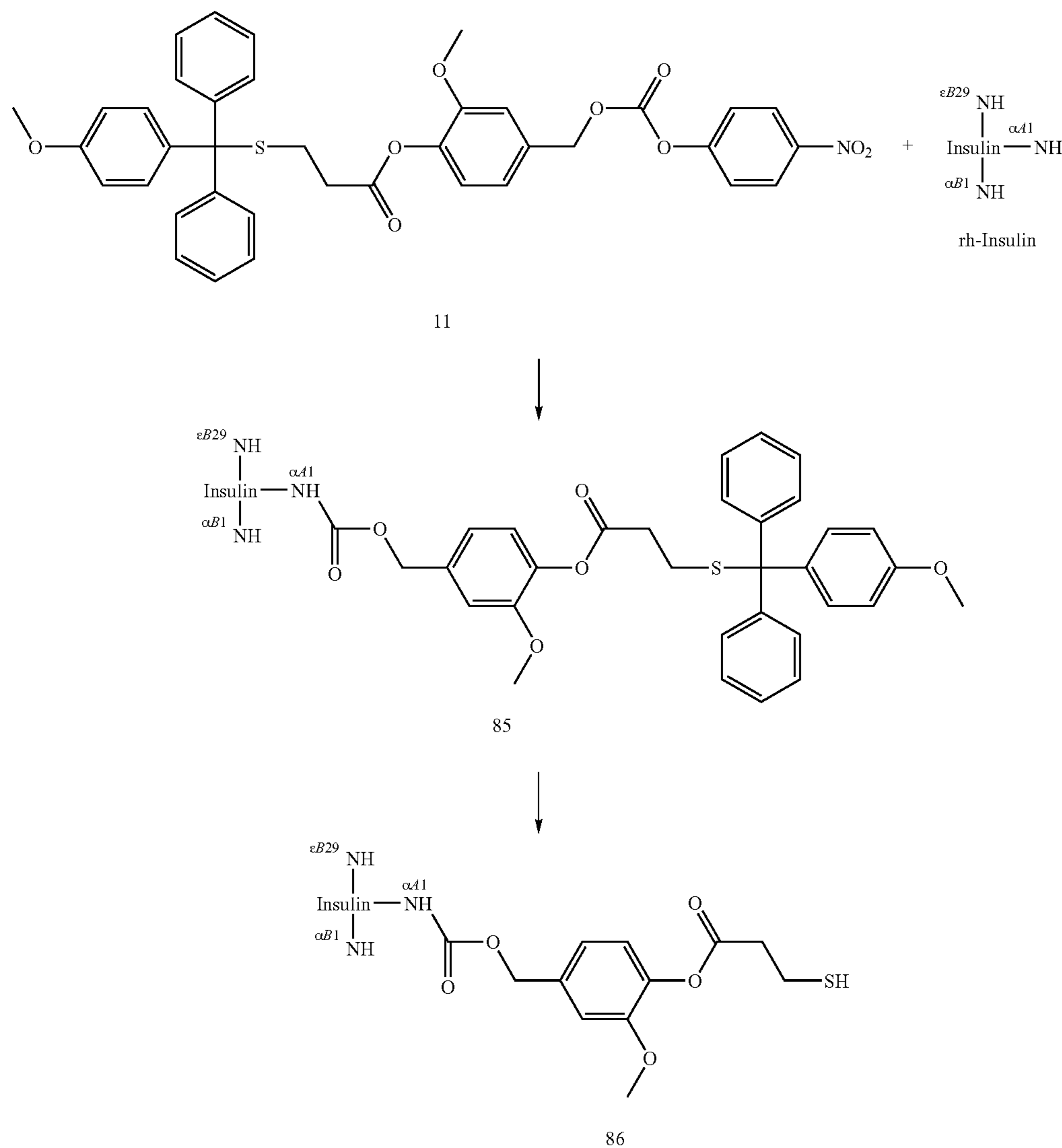
XI-4-1) Synthesis of N^{\alpha A1} -thiolinker-insulin 86
