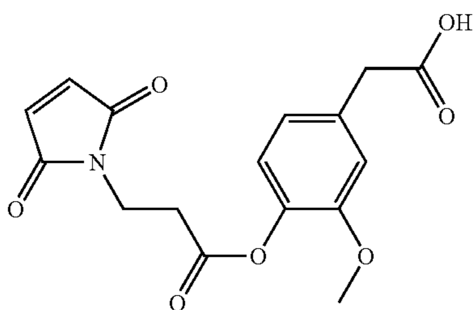
I-4) Synthesis of linker 6
