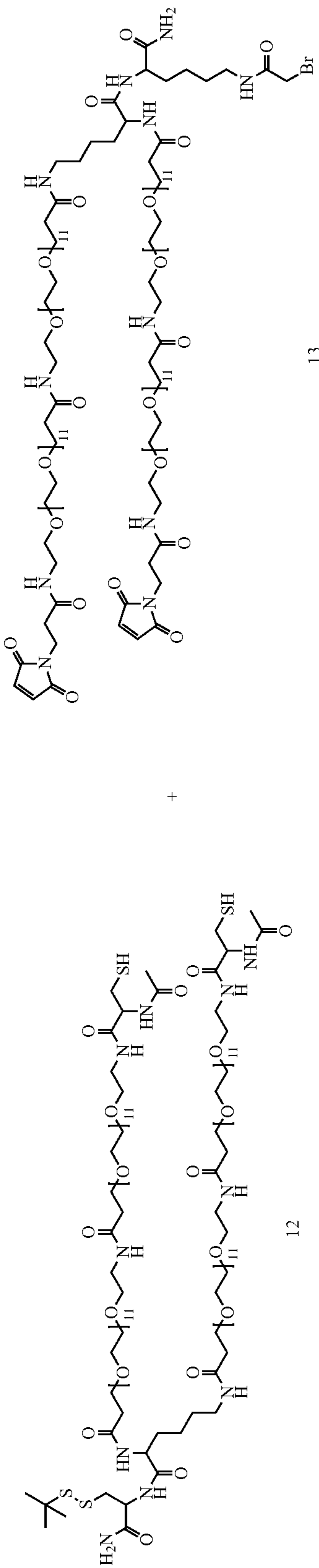
II-1). Synthesis of bis-maleimido-macrocylic structure 18
