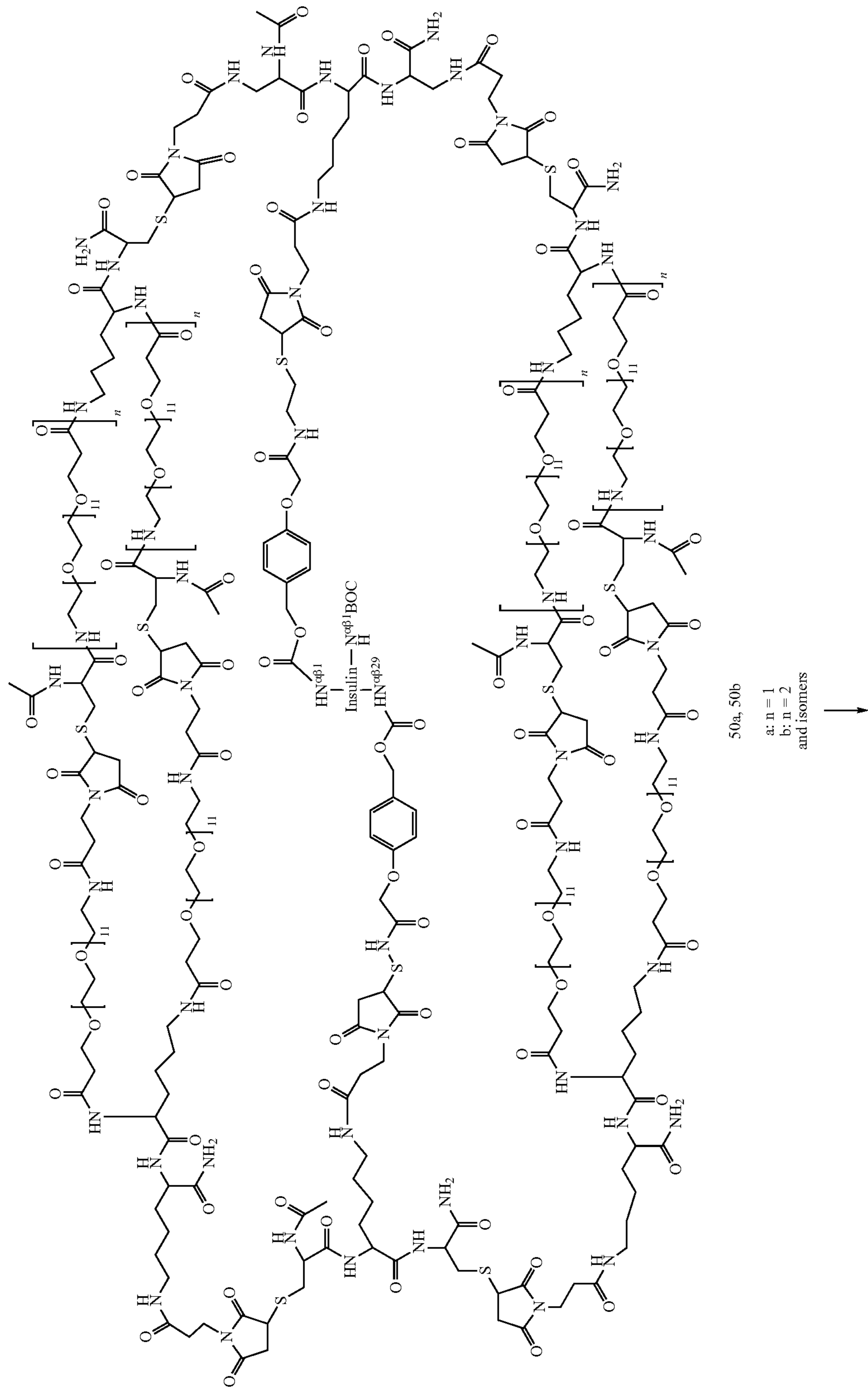
VII-4) Release of insulin from insulin_MPIC_50a/50b
