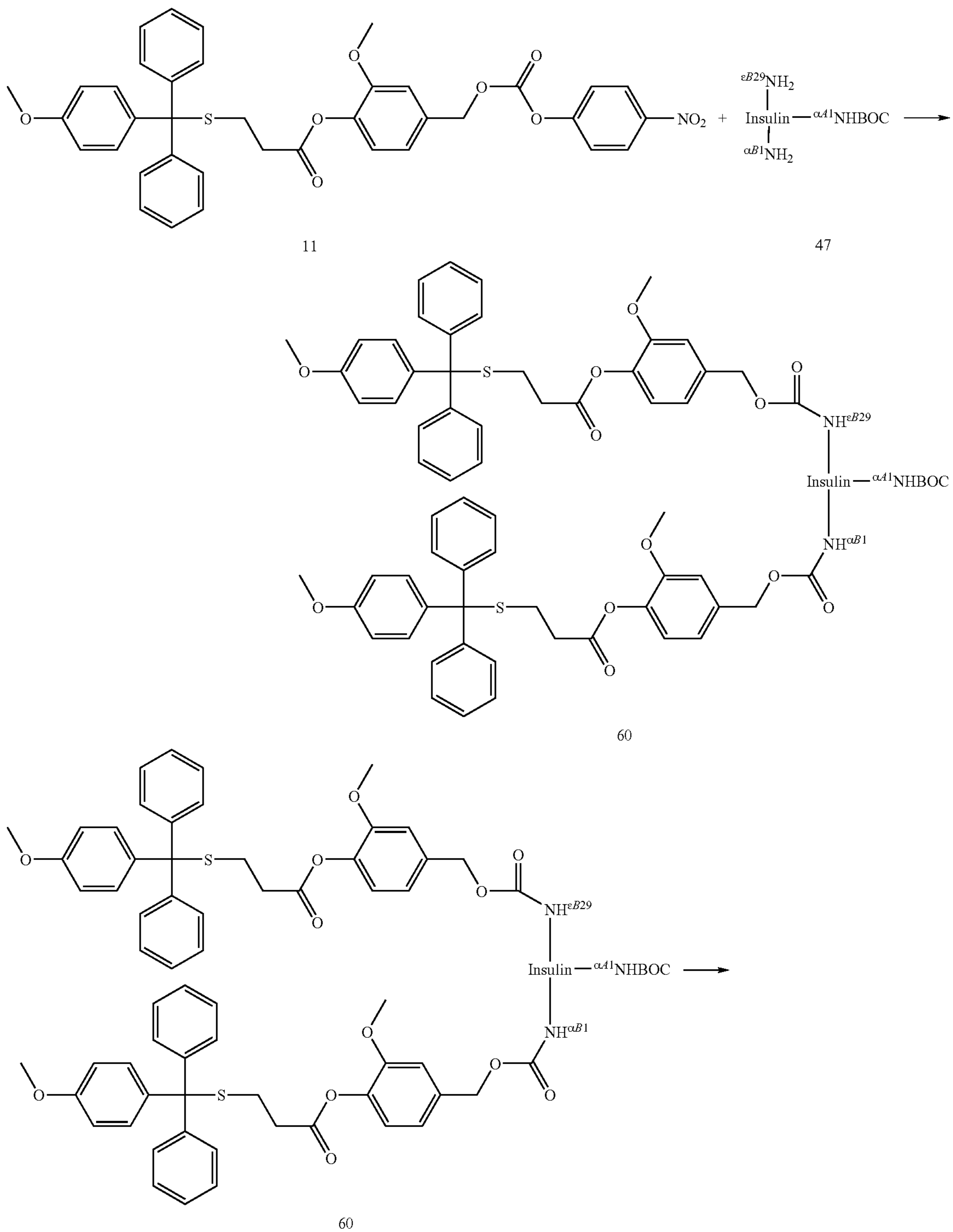
IX-1) Synthesis of N \alpha B1 ,N \epsilon B29 -bis-(thiolinker)-insulin 61
