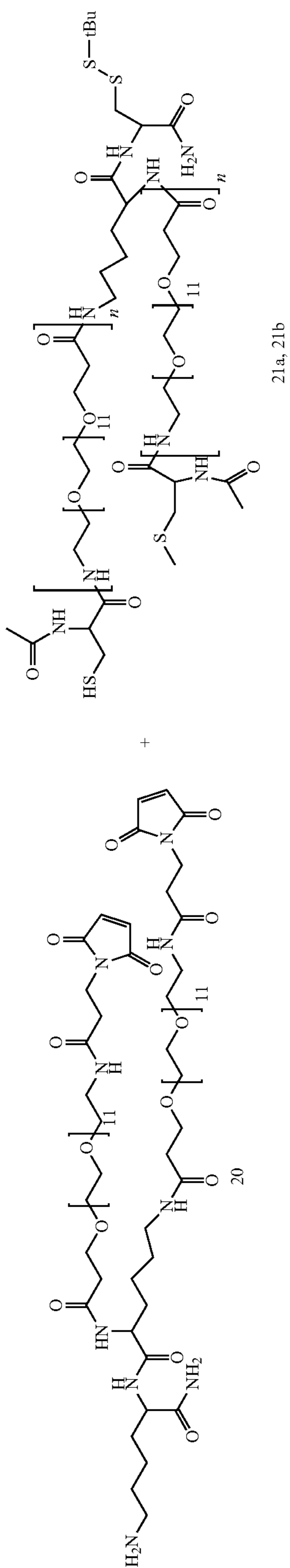
II-3) Synthesis of bis-maleimido-macrocylic structures 25a and 25b
