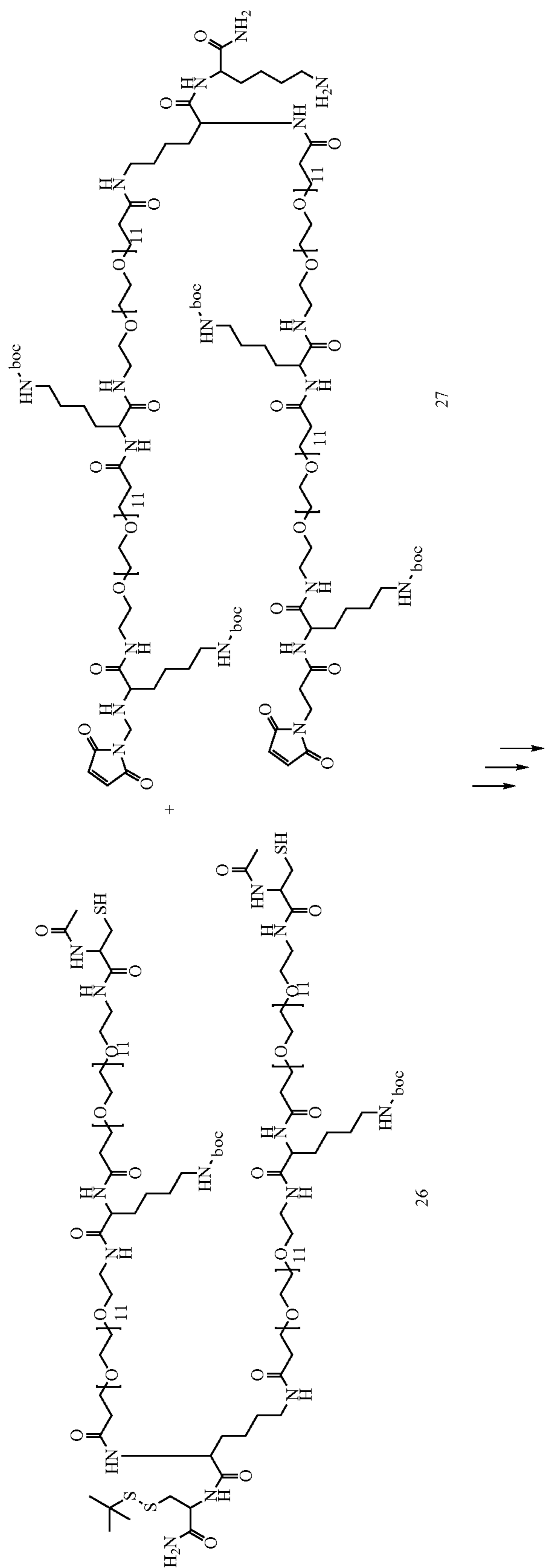
II-4) Synthesis of bis-maleimido-core-macrocylic structure 31
