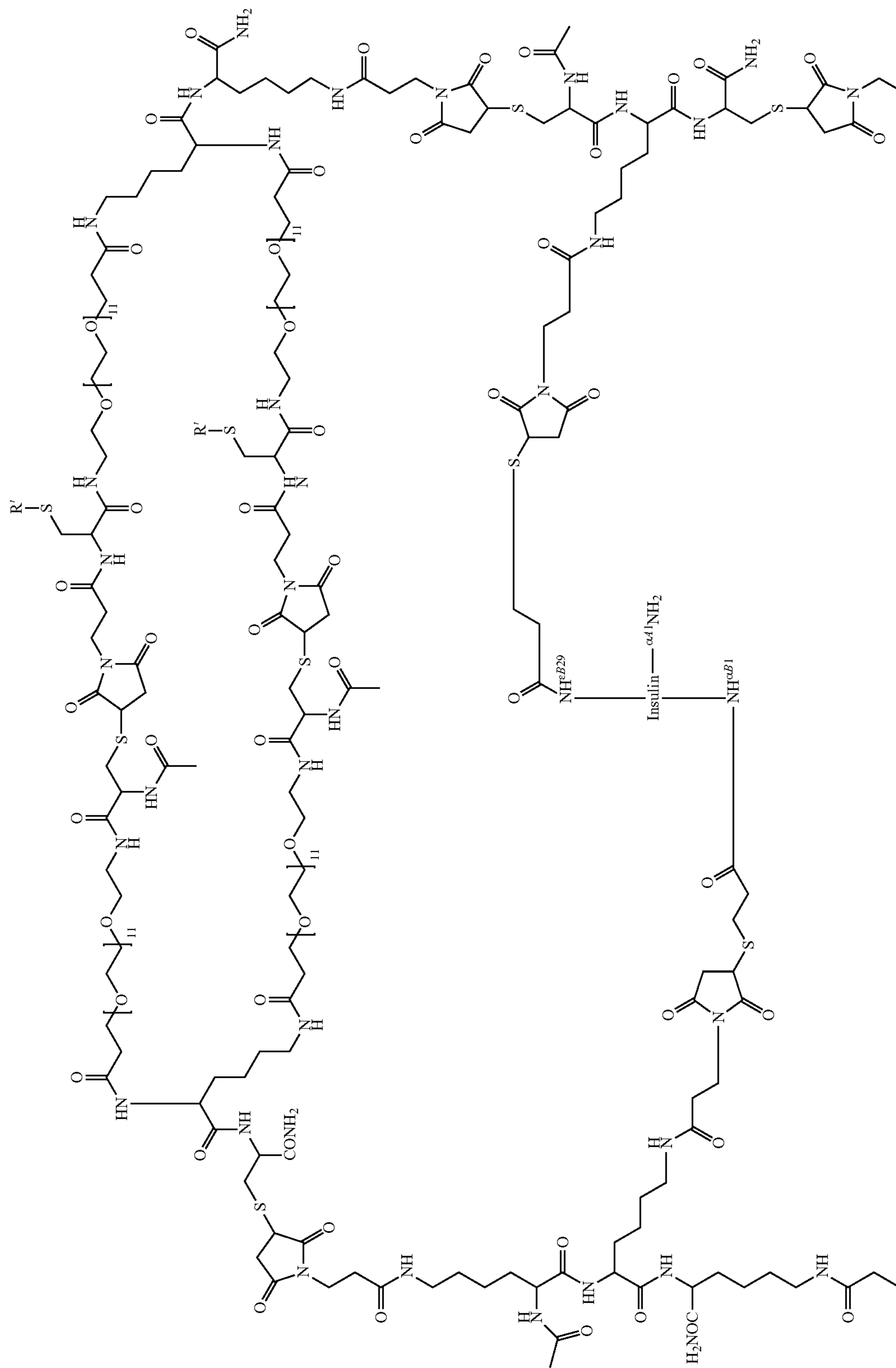
VIII-3) Synthesis of modified Insulin MPIC 57, 58 and 59
