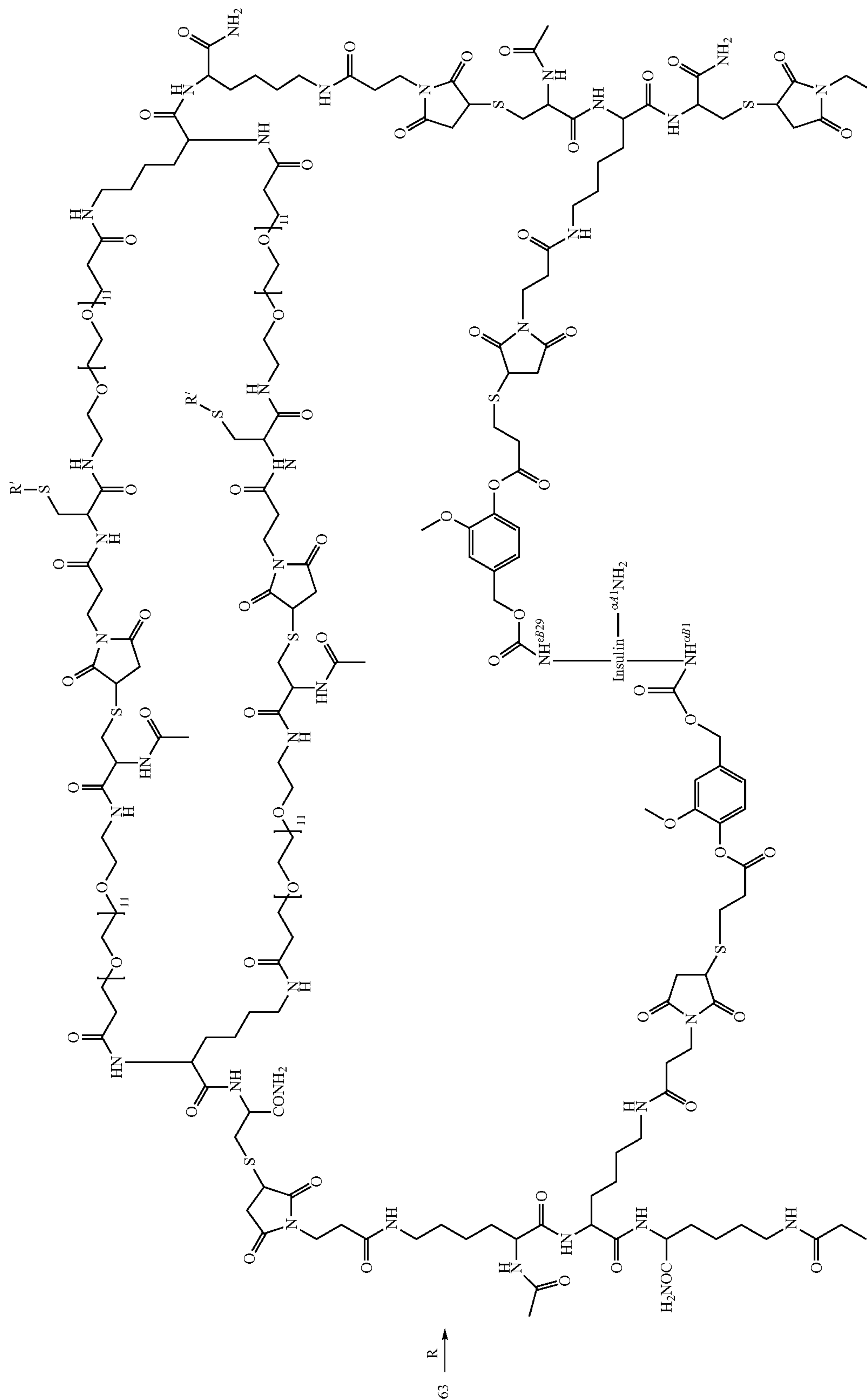
IX-3) Synthesis of modified Insulin_MPIC_64 and 65
