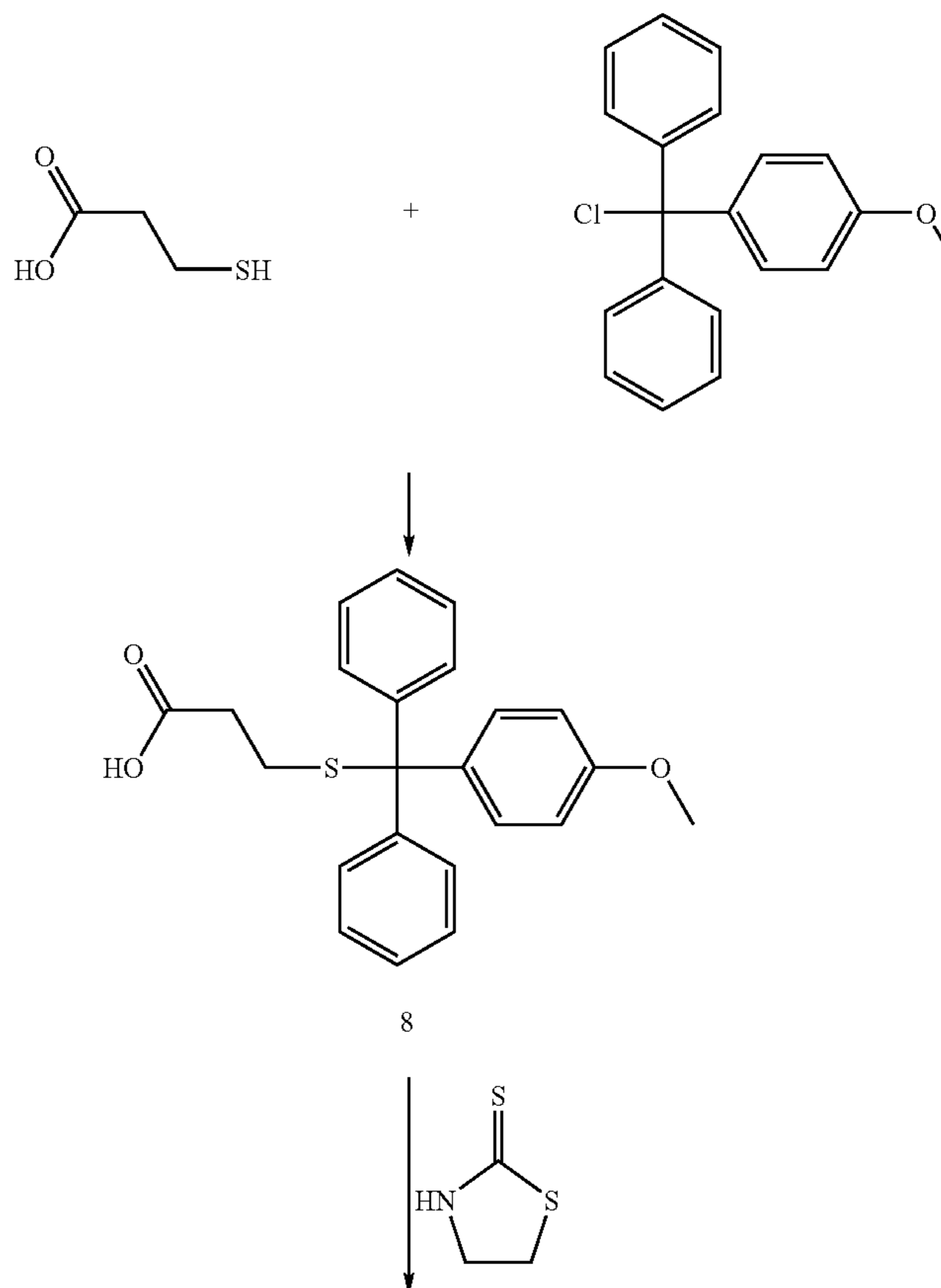
I-6) Synthesis of linker 11
