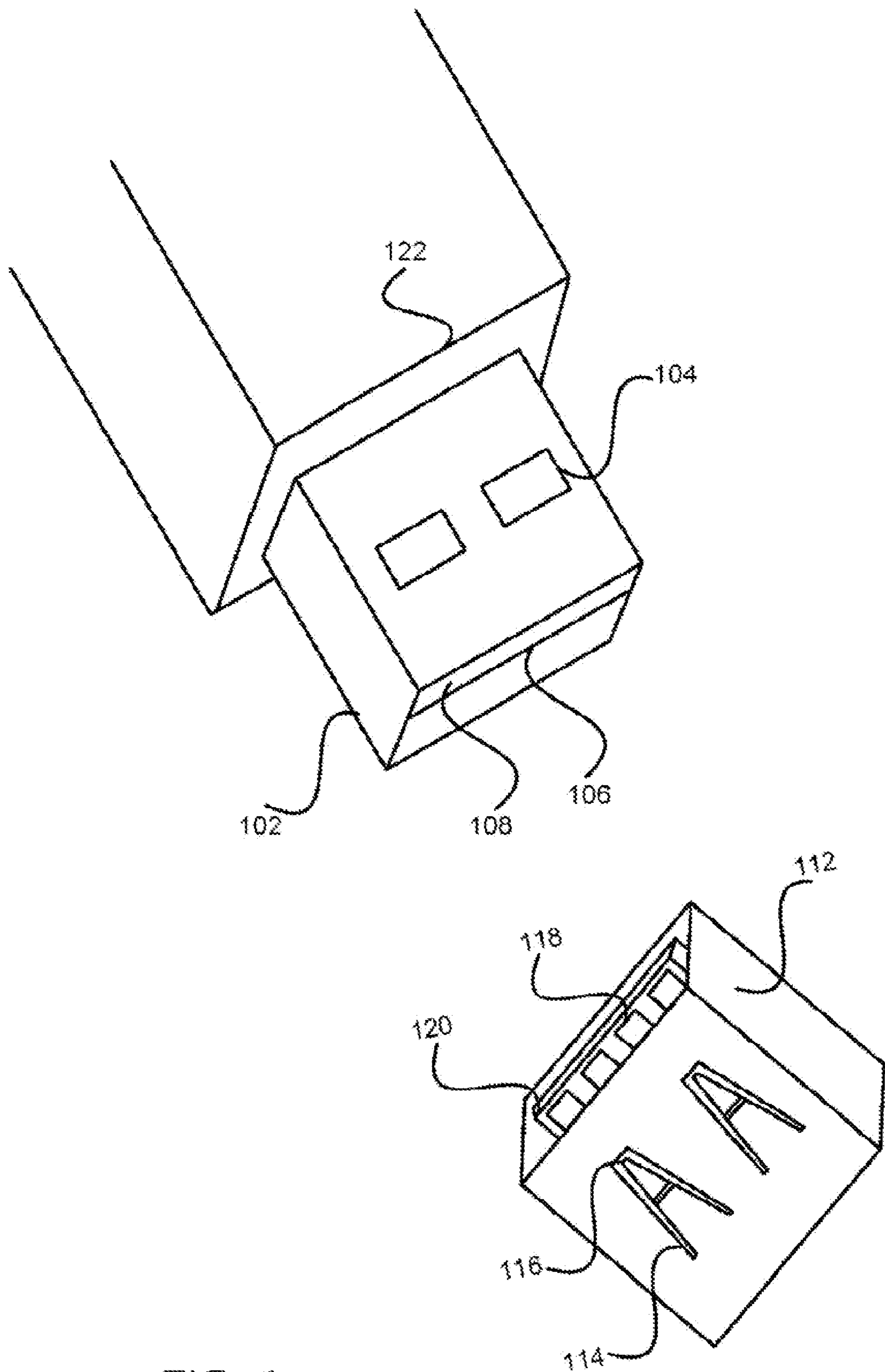
FIG. 1 (PRIOR ART)
