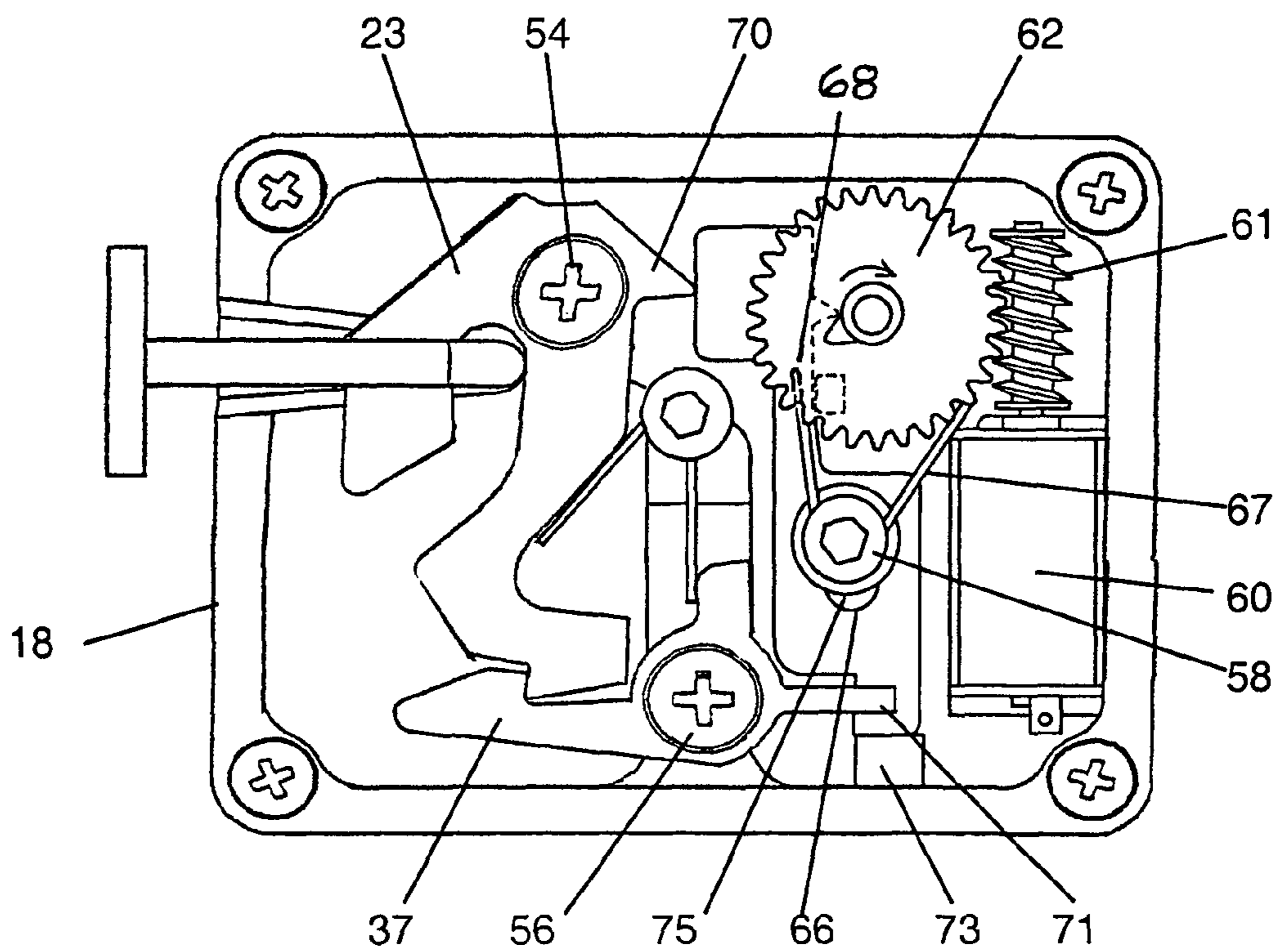
FIG. 7. LOCKED
