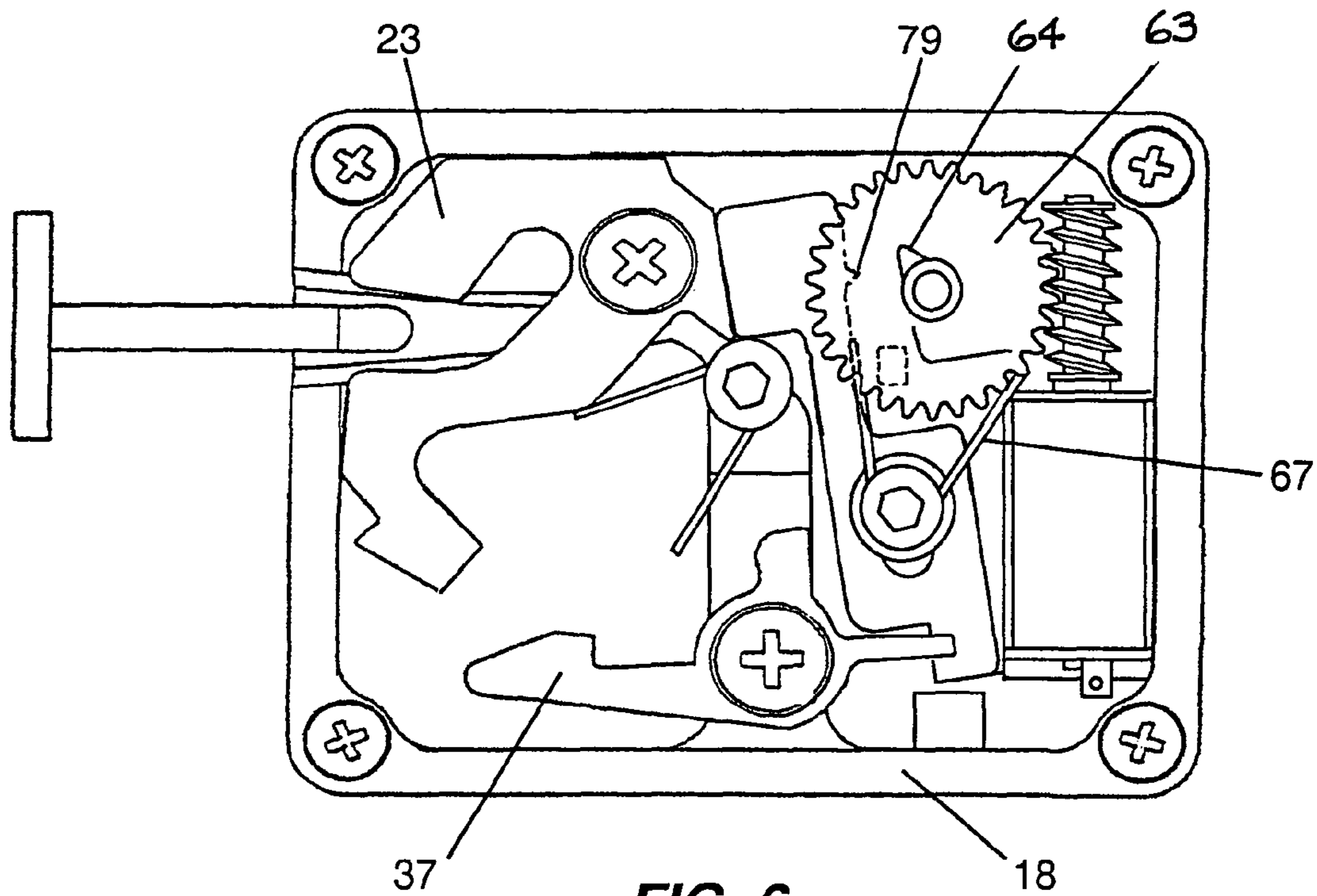
FIG. 6. UNLOCKED
