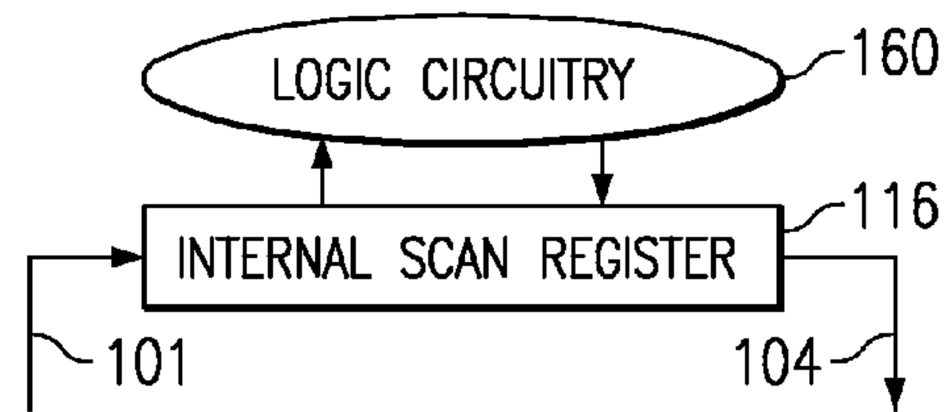
FIG. 1C (PRIOR ART)
