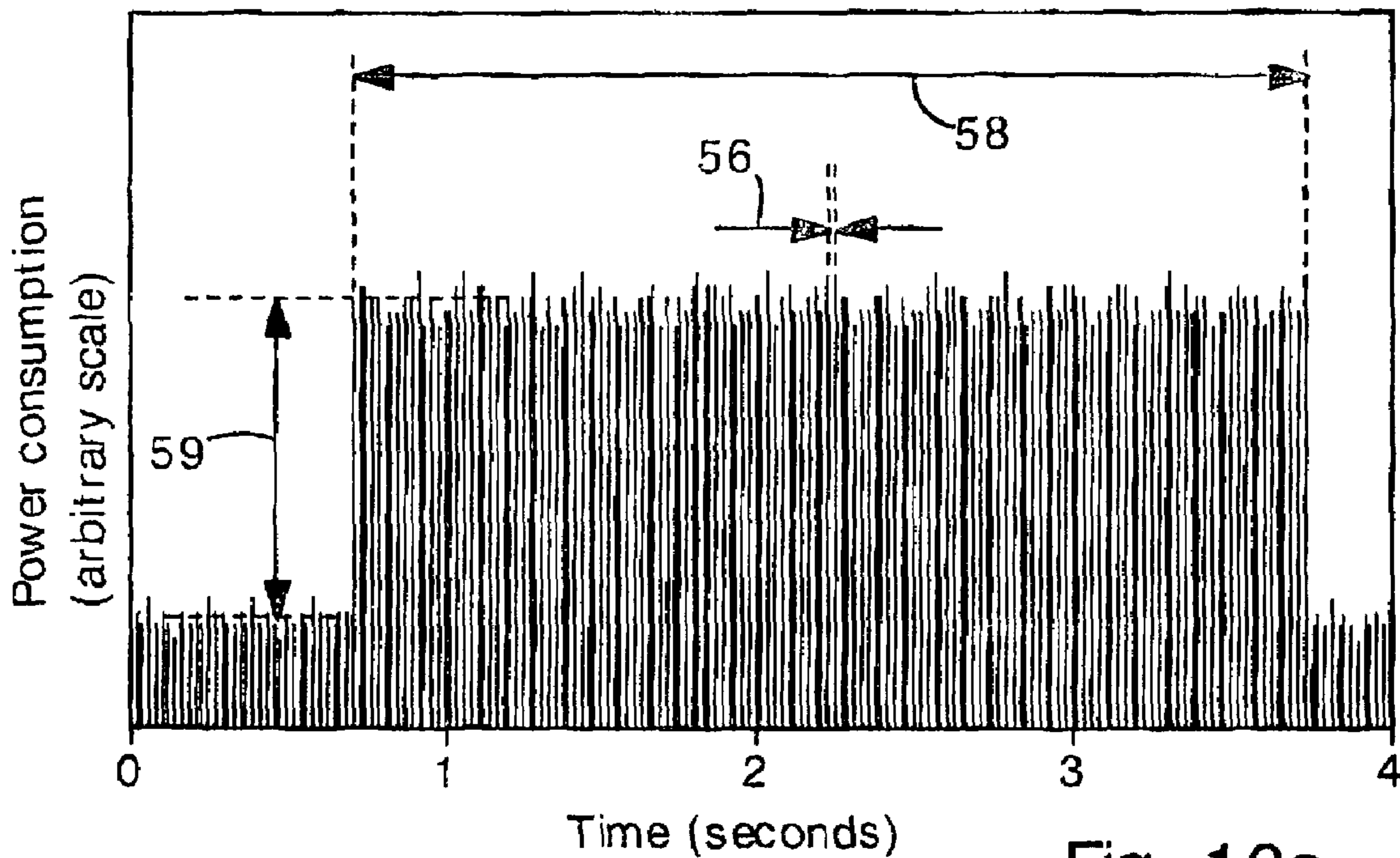
TCP-based Flooding Attack Fig. 10a
