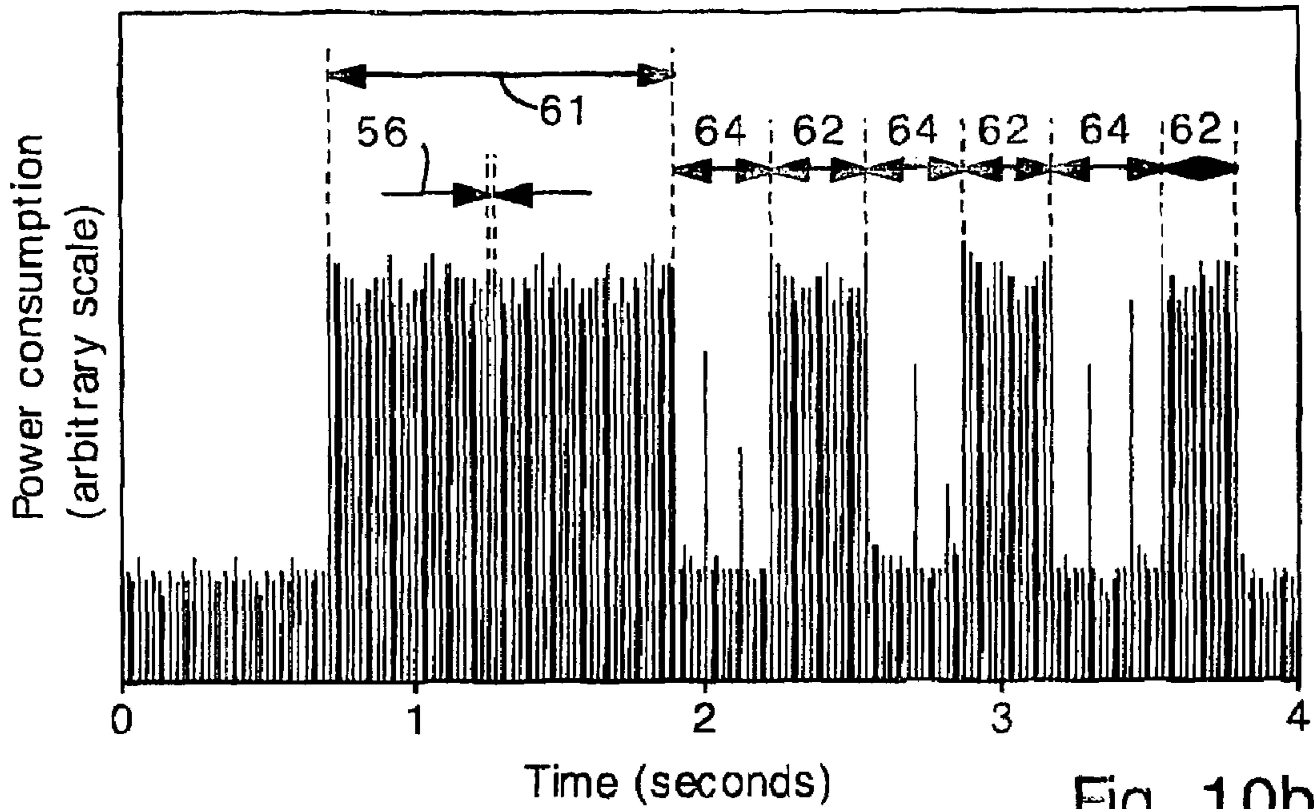
UDP-based Flooding Attack
