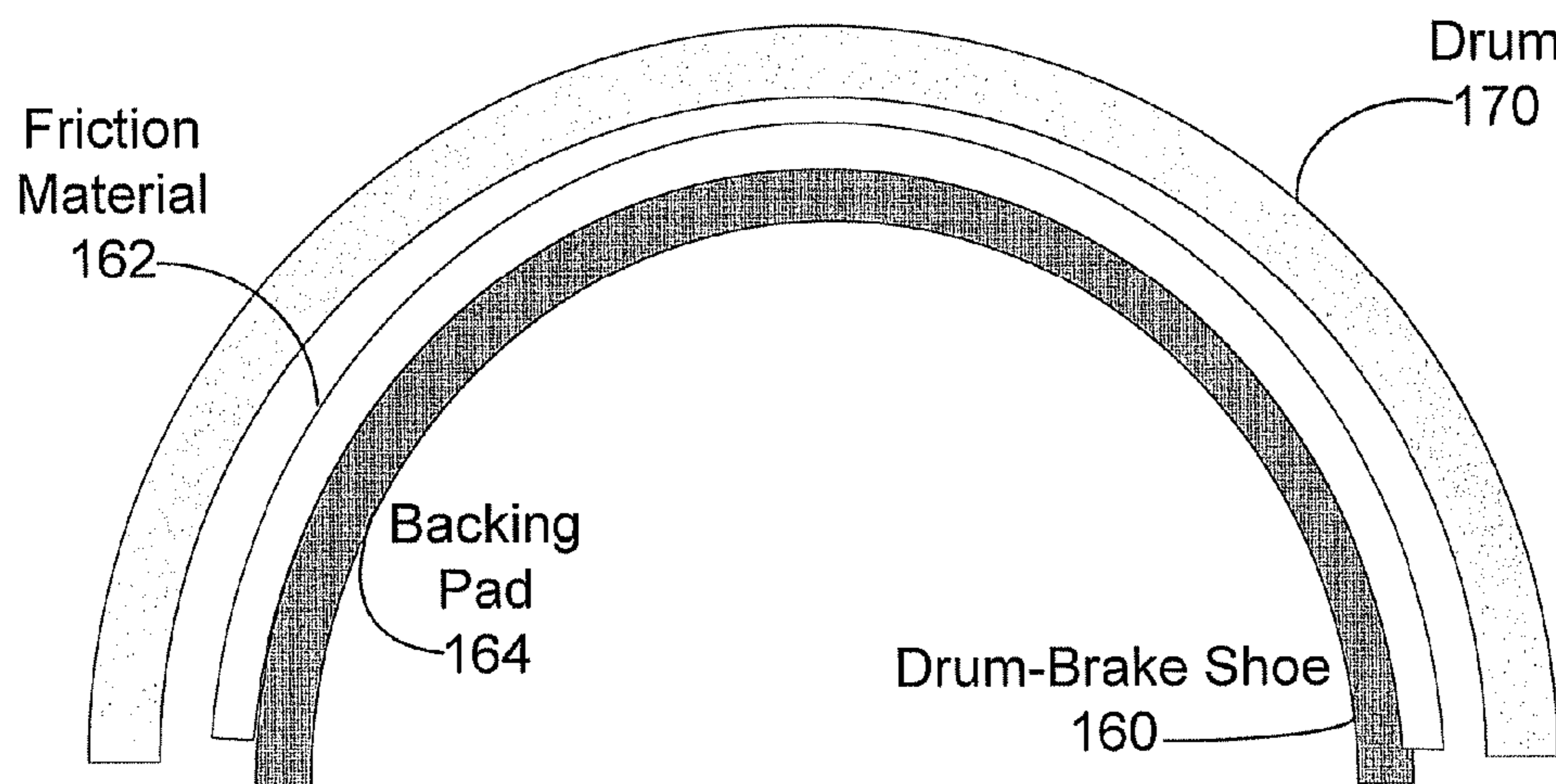
CROSS-SECTIONAL VIEW OF TYPICAL DRUM BRAKE ASSEMBLY 150
