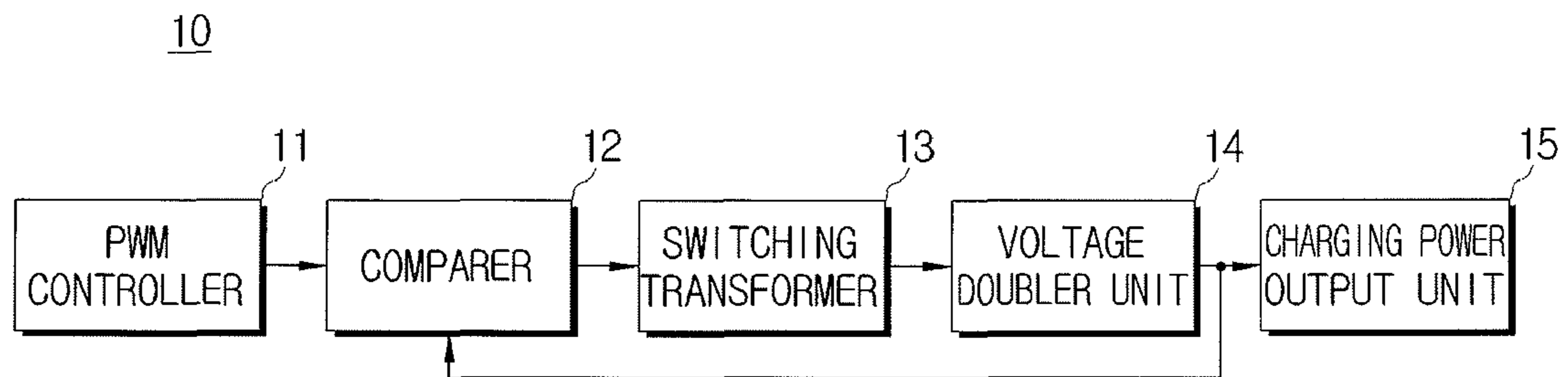
FIG. 1A (RELATED ART)
