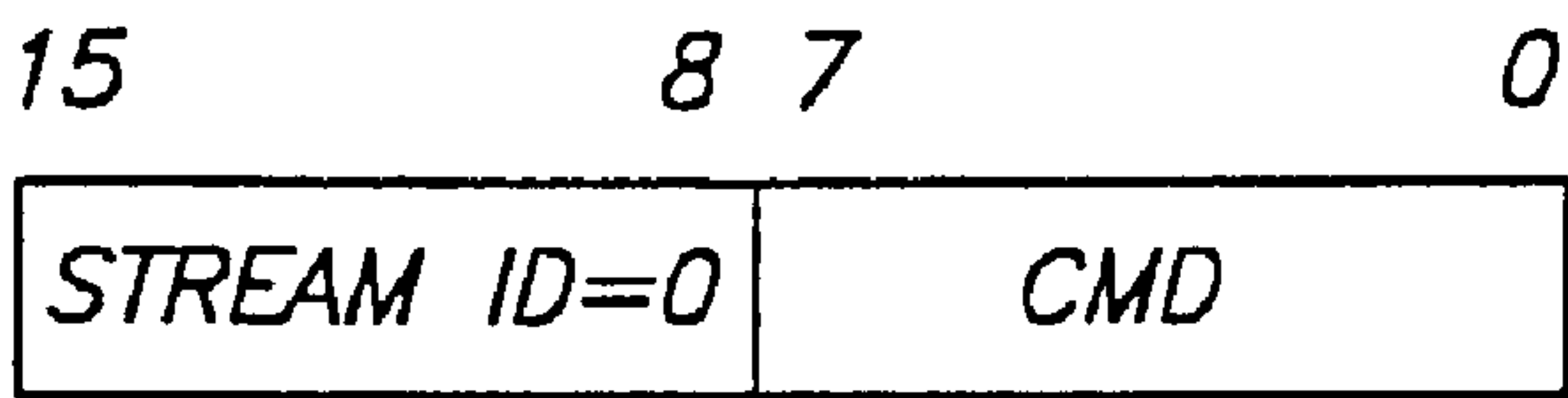
FIG. 4C STREAM ZERO POLL FRAME FORMAT
