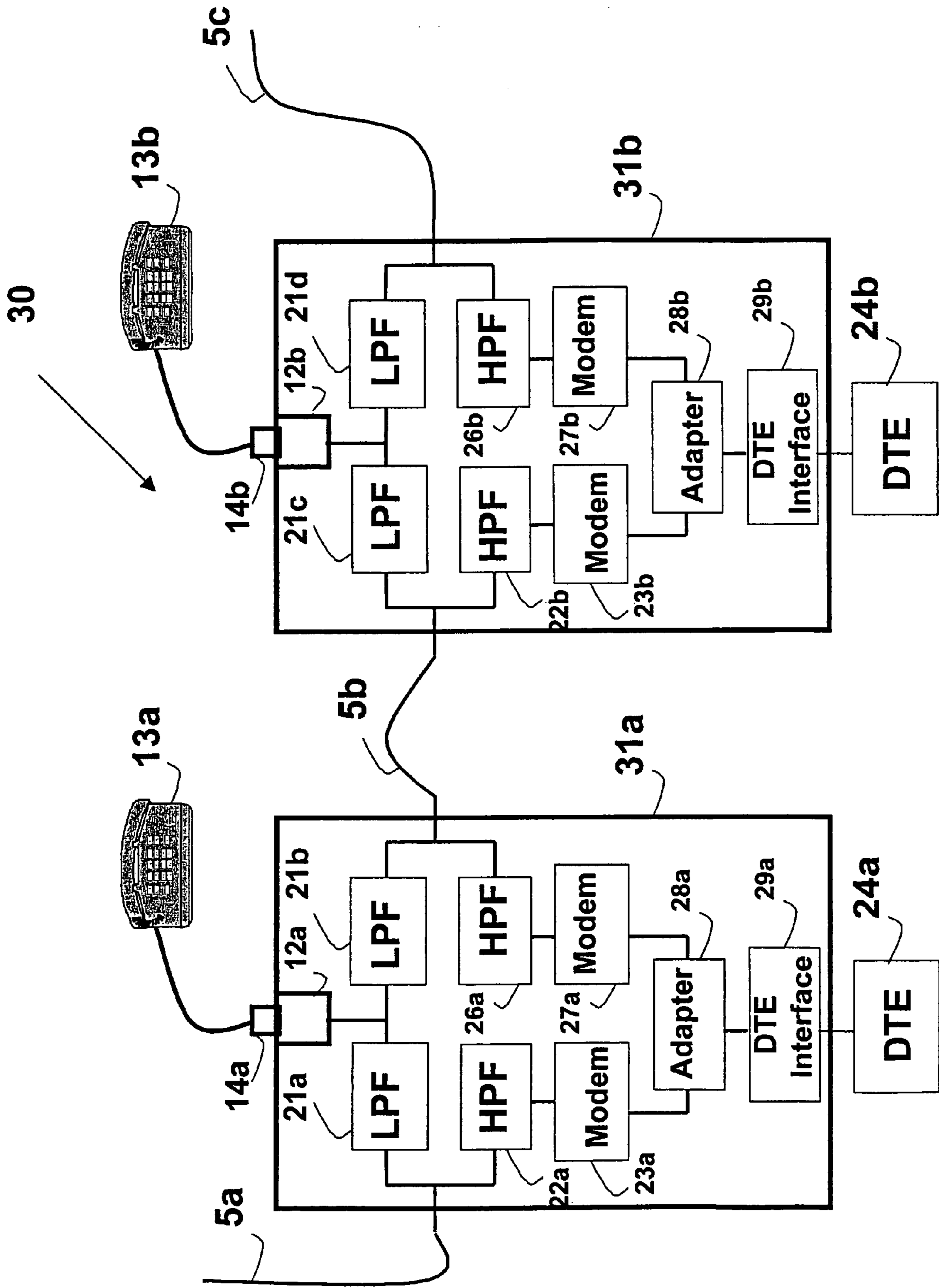
FIGURE 3 (PRIOR-ART)
