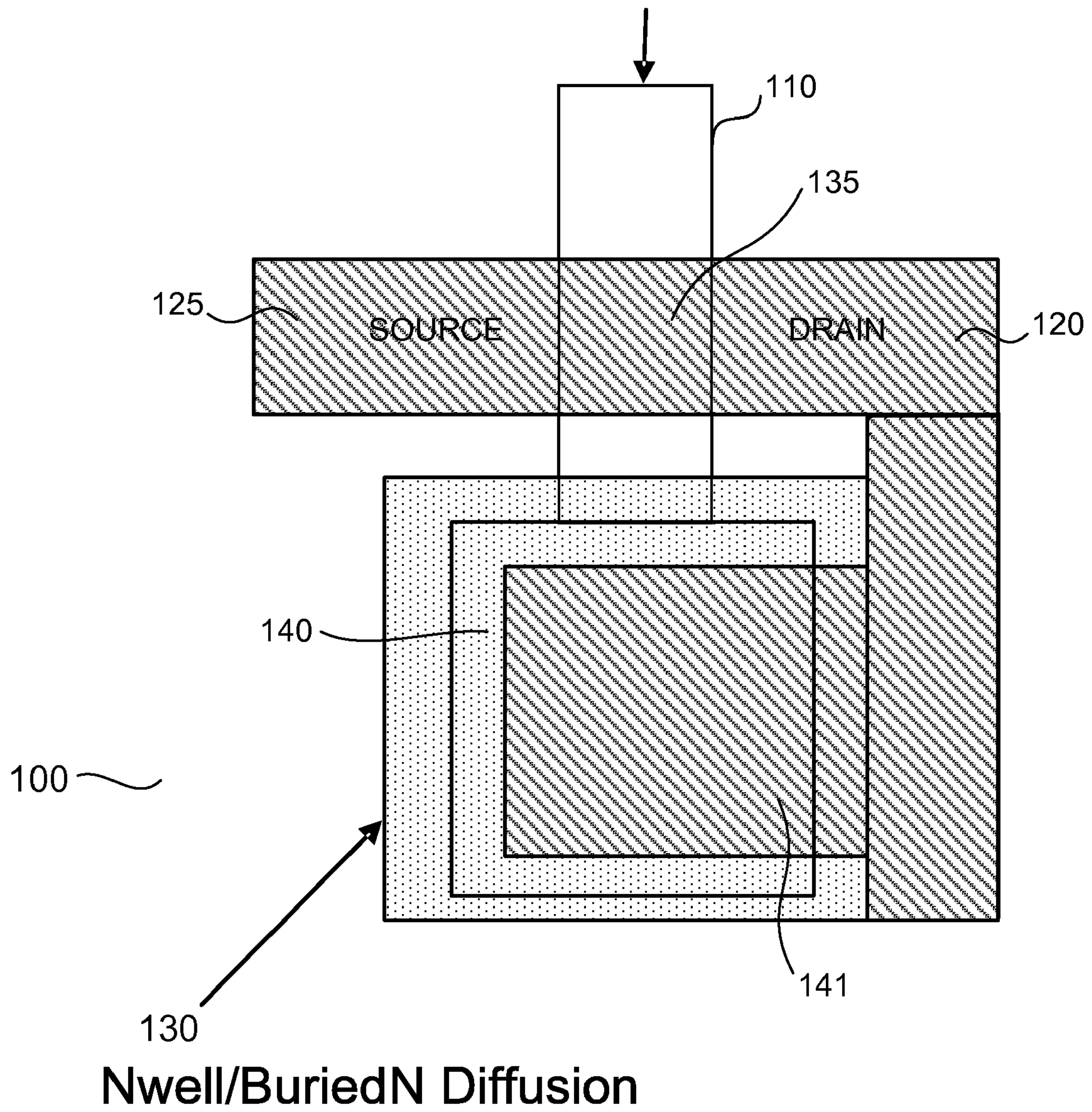
FIG. 1 Floating Gate
