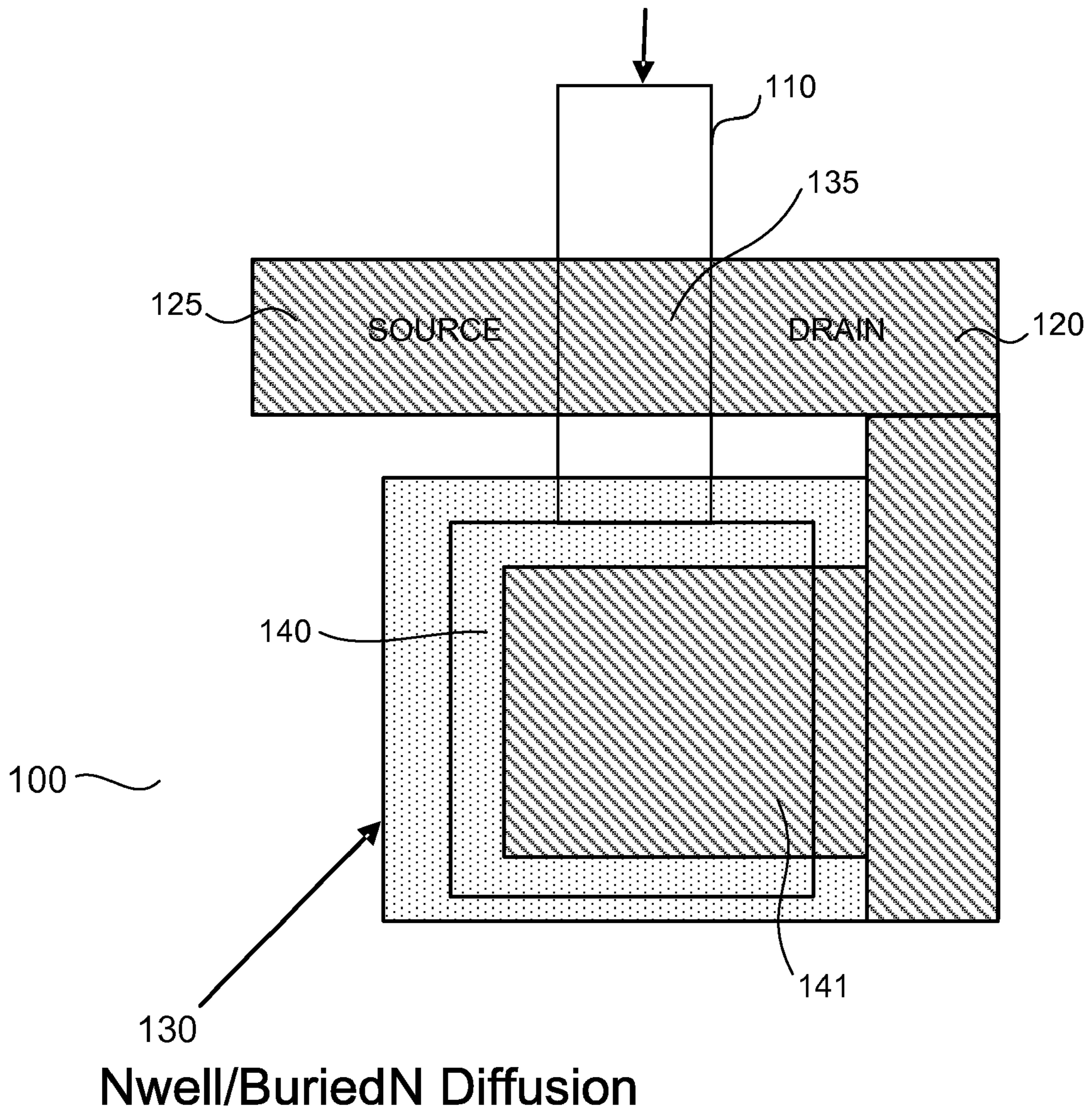
FIG. 1 Floating Gate
