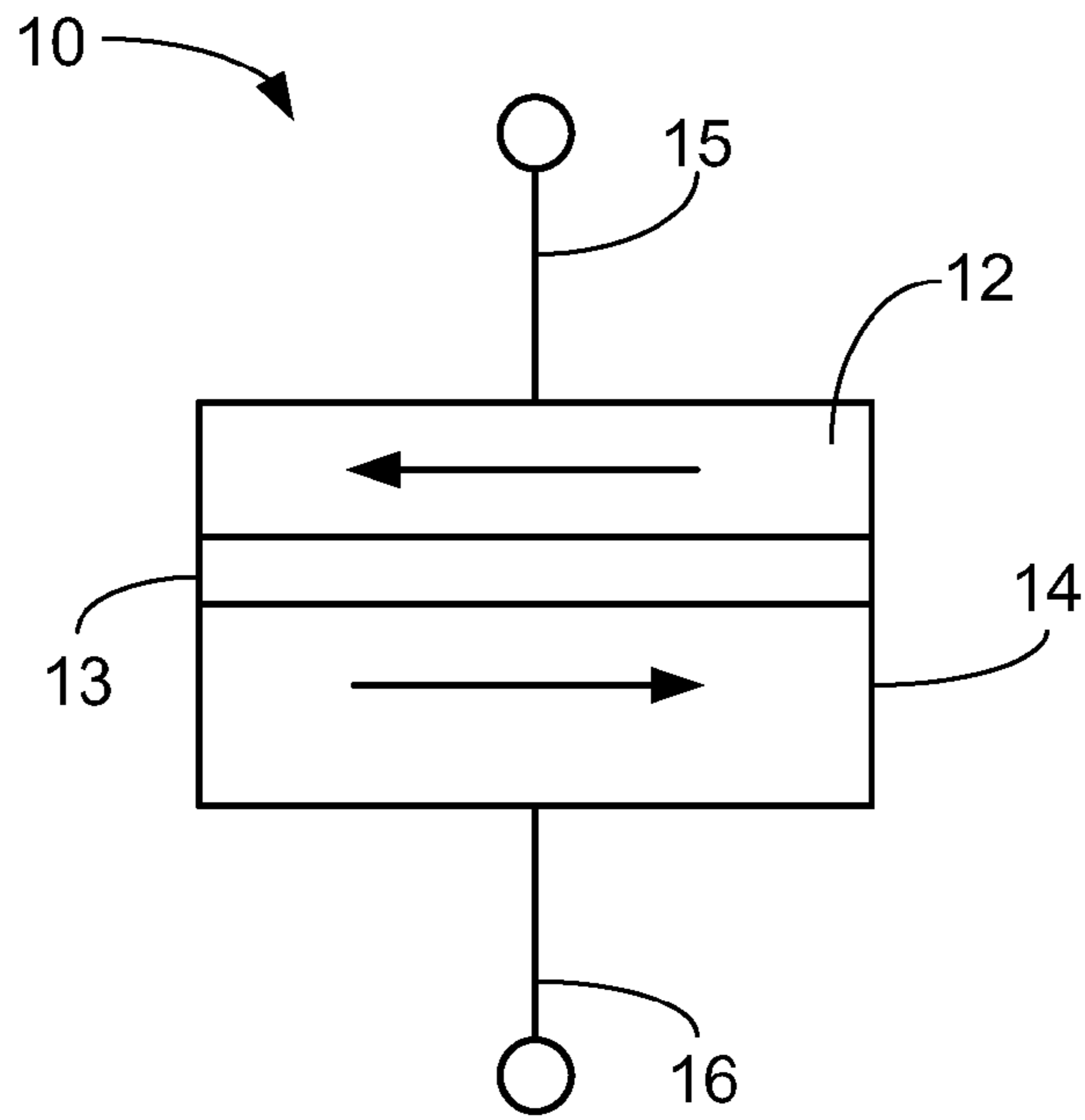
FIG. 2 Prior Art
