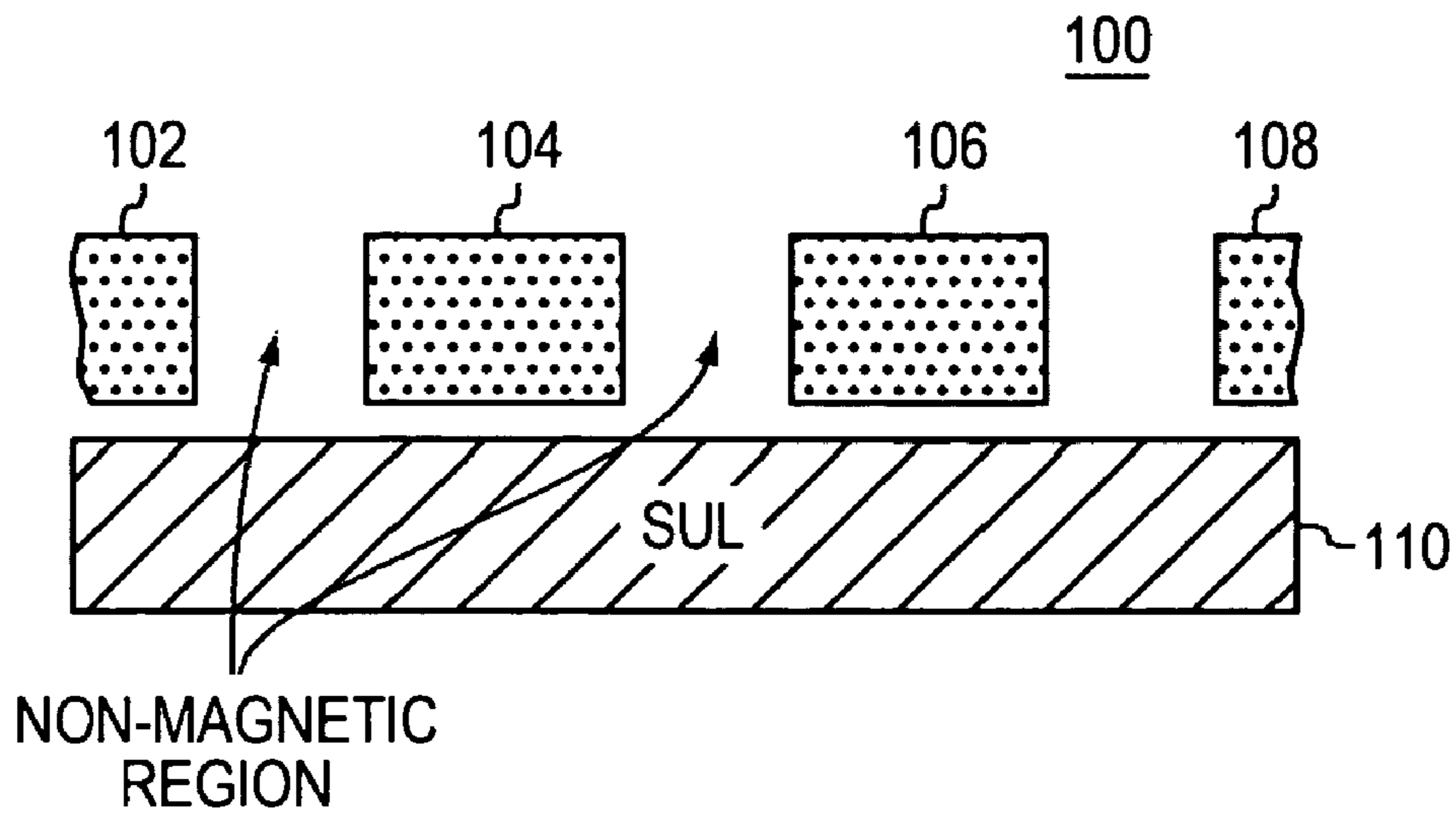
PRIOR ART ACTUAL DTR/PMR MEDIA DESIGN
