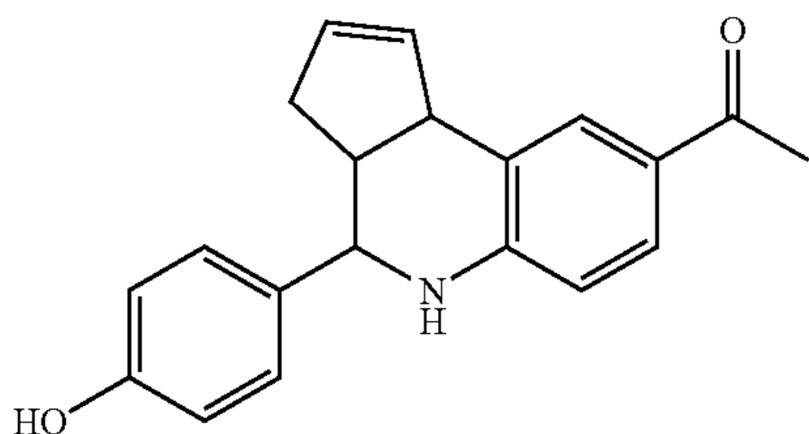
1-[4-(4-Hydroxy-phenyl)-3a,4,5,9b-tetrahydro-3H-cyclopenta[c]quinolin-8-yl]-ethanone
