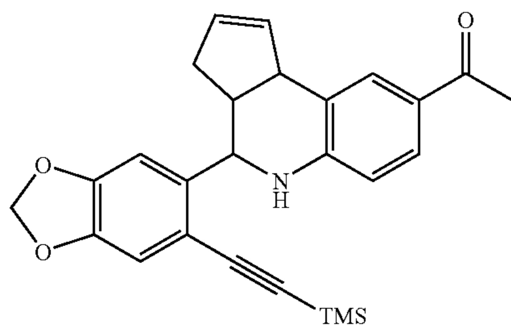
1-[4-(6-Trimethylsilyl-ethynyl-benzo[1,3]dioxol-5-yl)-3a,4,5,9b-tetrahydro-3H-cyclopenta[c]quinolin-8-yl]-ethanone
