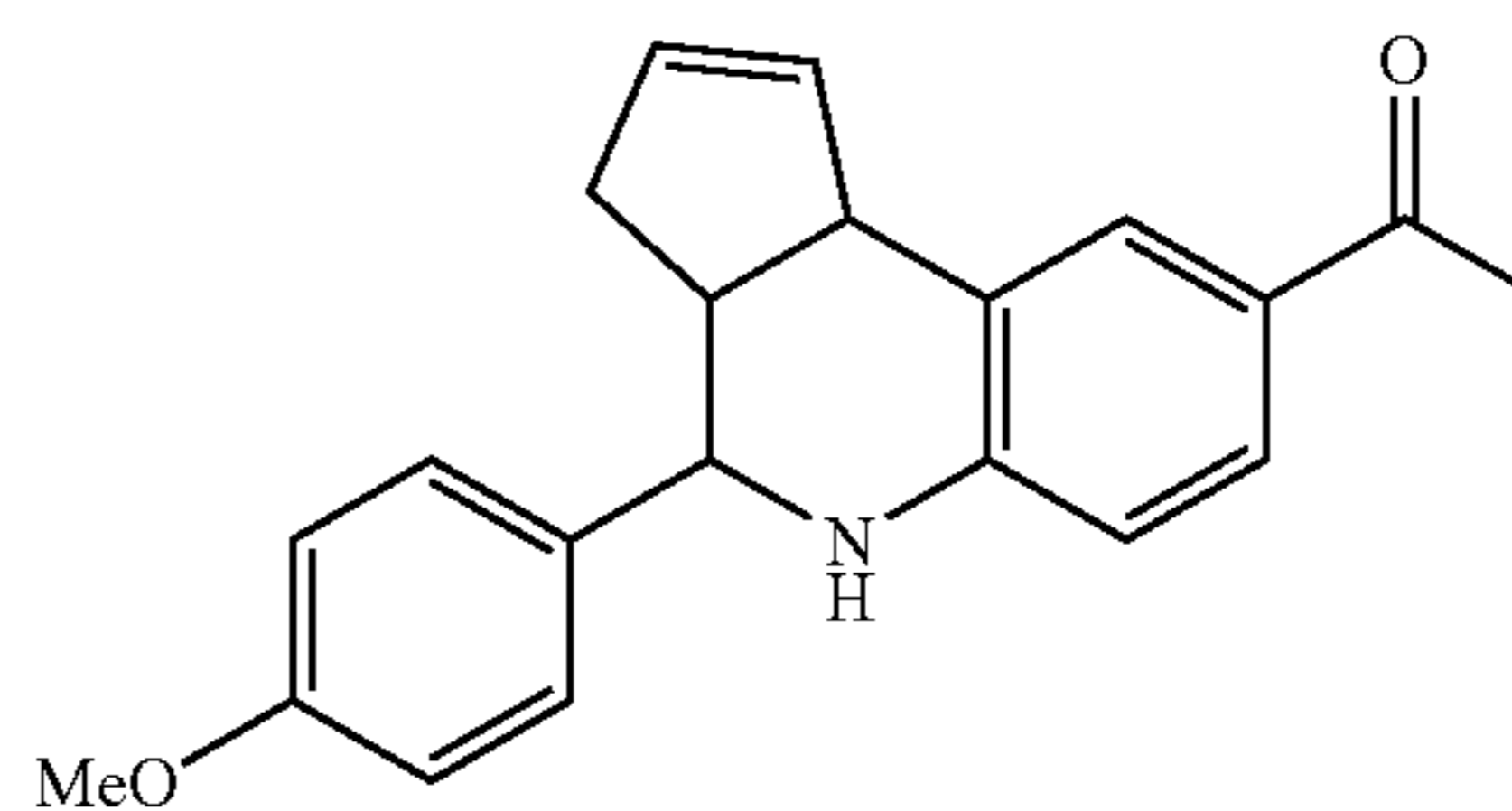
1-[4-(4-Methoxy-phenyl)-3a,4,5,9b-tetrahydro-3H-cyclopenta[c]quinolin-8-yl]-ethanone
