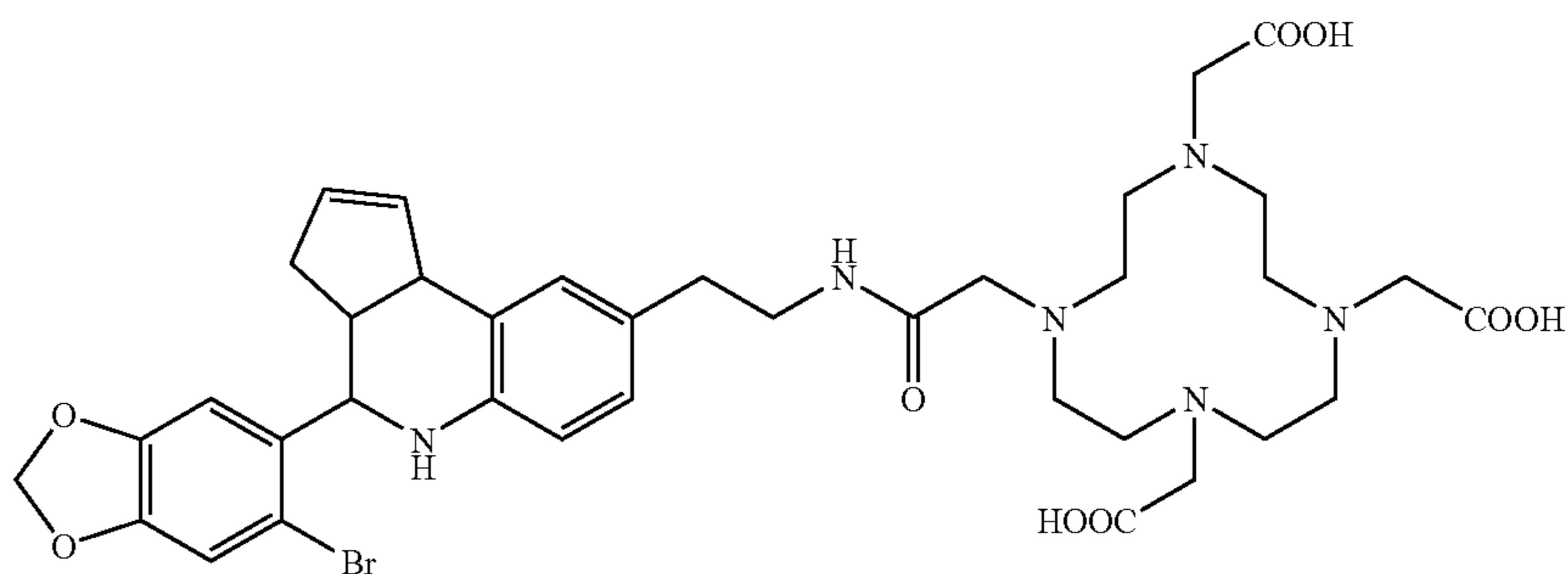
[4-({2-[4-(6-Bromo-benzo[1,3]dioxol-5-yl)-3a,4,5,9b-tetrahydro-3H-cyclopenta[c]quinolin-8-yl]-ethyl}-carbonyl)-methyl]-7,10-bis-carboxymethyl-1,4,7,10-tetraaza-cyclododec-1-yl]-acetic Acid
