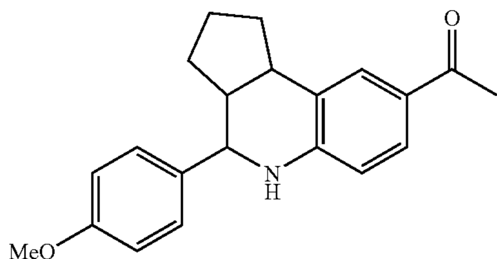
1-[4-(4-Methoxy-phenyl)-2,3,3a,4,5,9b-hexahydro-1H-cyclopenta[c]quinolin-8-yl]ethanone
