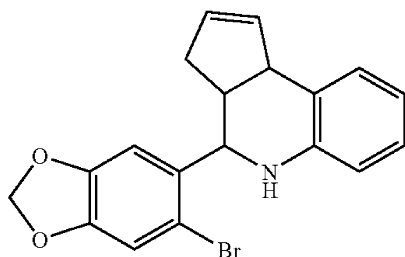
4-(6-Bromo-benzo[1,3]dioxol-5-yl)-3a,4,5,9b-tetrahydro-3H-cyclopenta[c]quinoline
