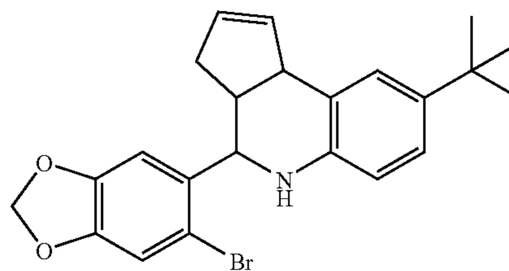
4-(6-Bromo-benzo[1,3]dioxol-5-yl)-8-tert-butyl-3a,4,5,9b-tetrahydro-3H-cyclopenta[c]quinoline
