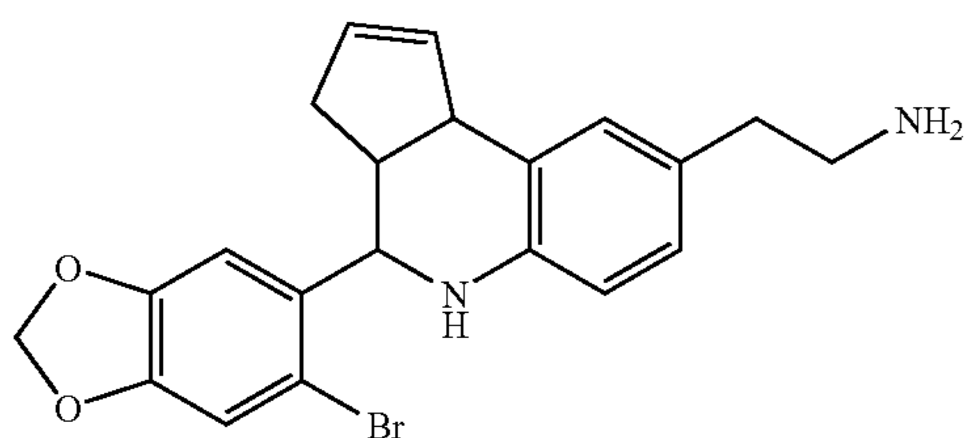
2-[4-(6-Bromo-benzo[1,3]dioxol-5-yl)-3a,4,5,9b-tetrahydro-3H-cyclopenta[c]quinolin-8-yl]-ethylamine
