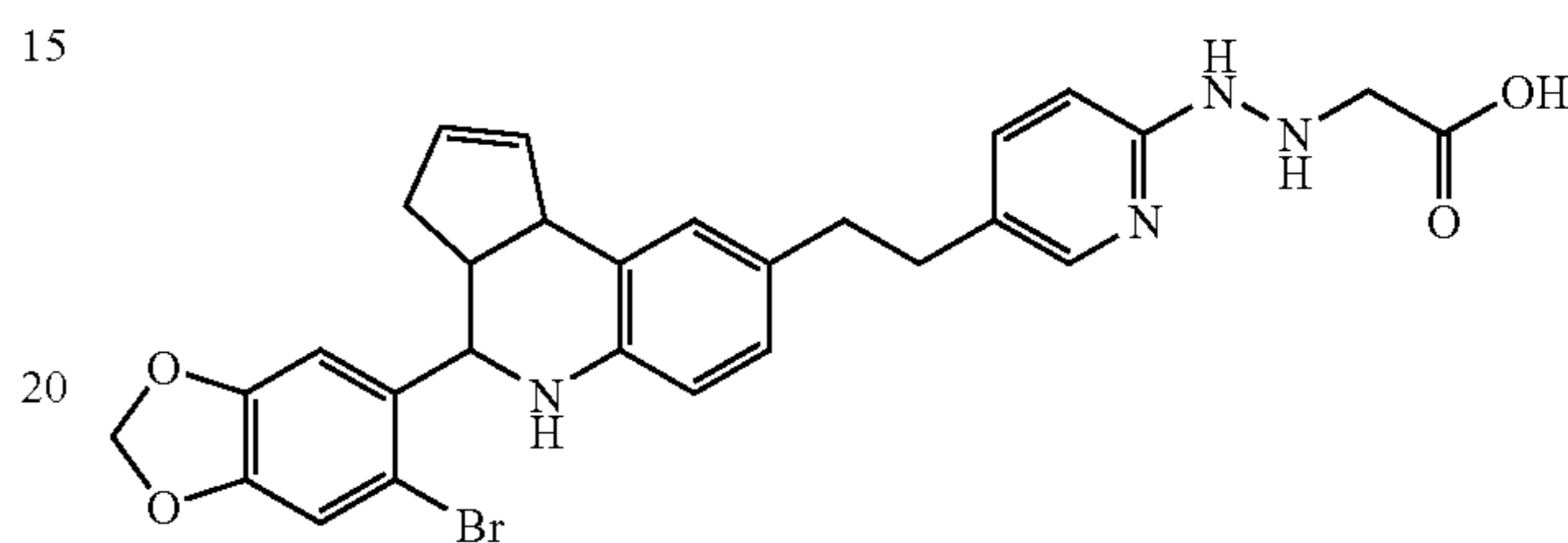
[N'-(5-{2-[4-(6-Bromo-benzo[1,3]dioxol-5-yl)-3a,4,5,9b-tetrahydro-3H-cyclopenta[c]quinolin-8-yl]-ethyl}-pyridin-2-yl)-N,N-bis-tertbutyloxycarbonyl-hydrazino]-acetic Acid
