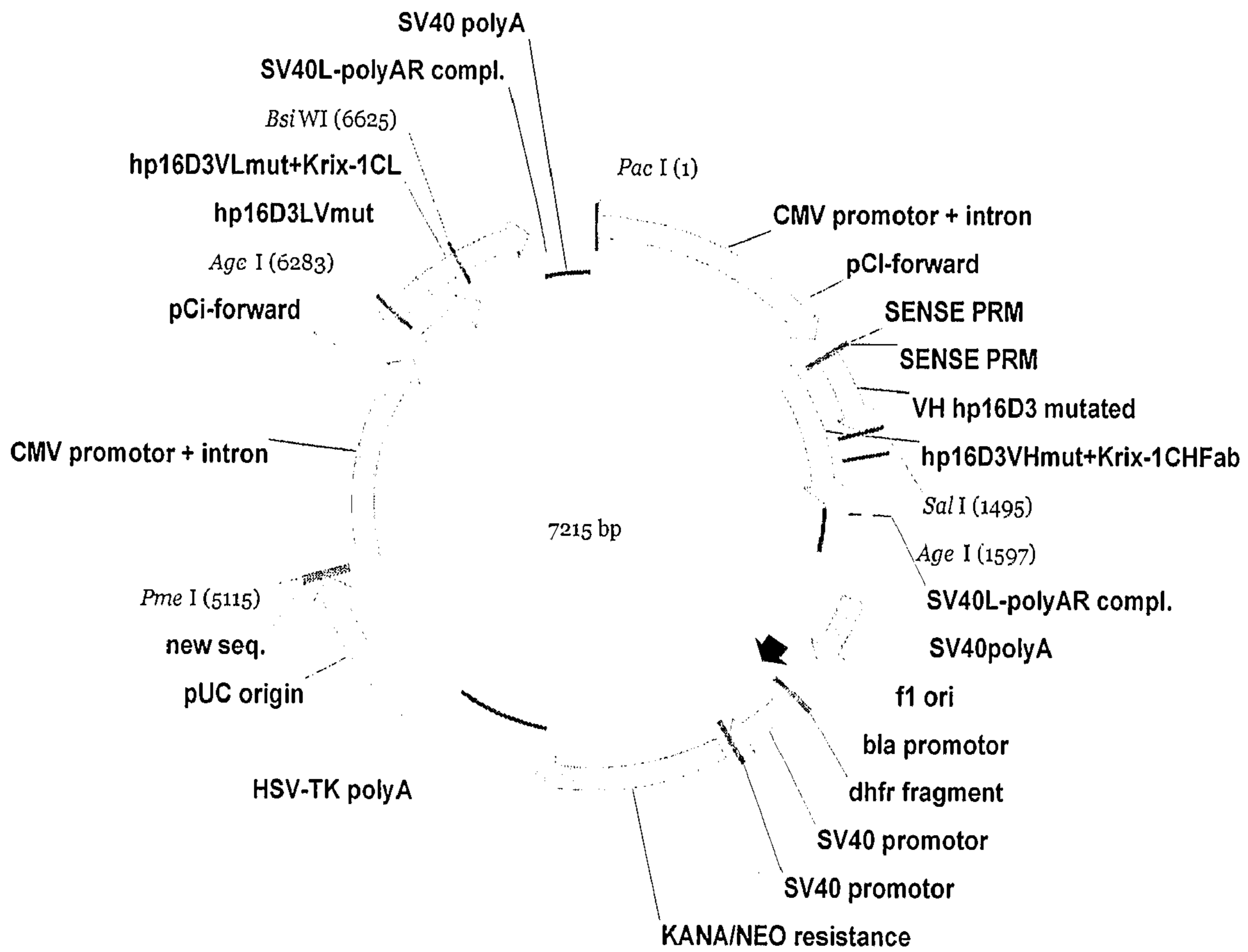
hp16D3mutcomplFab/pKNEO-MCS50-Fabvar #3 new seq
