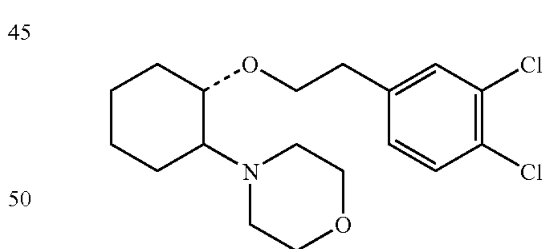
(1R,2R)/(1S,2S)-2-(4-morpholinyl)-1-(3,4-dichlorophenethoxy)cyclohexane
