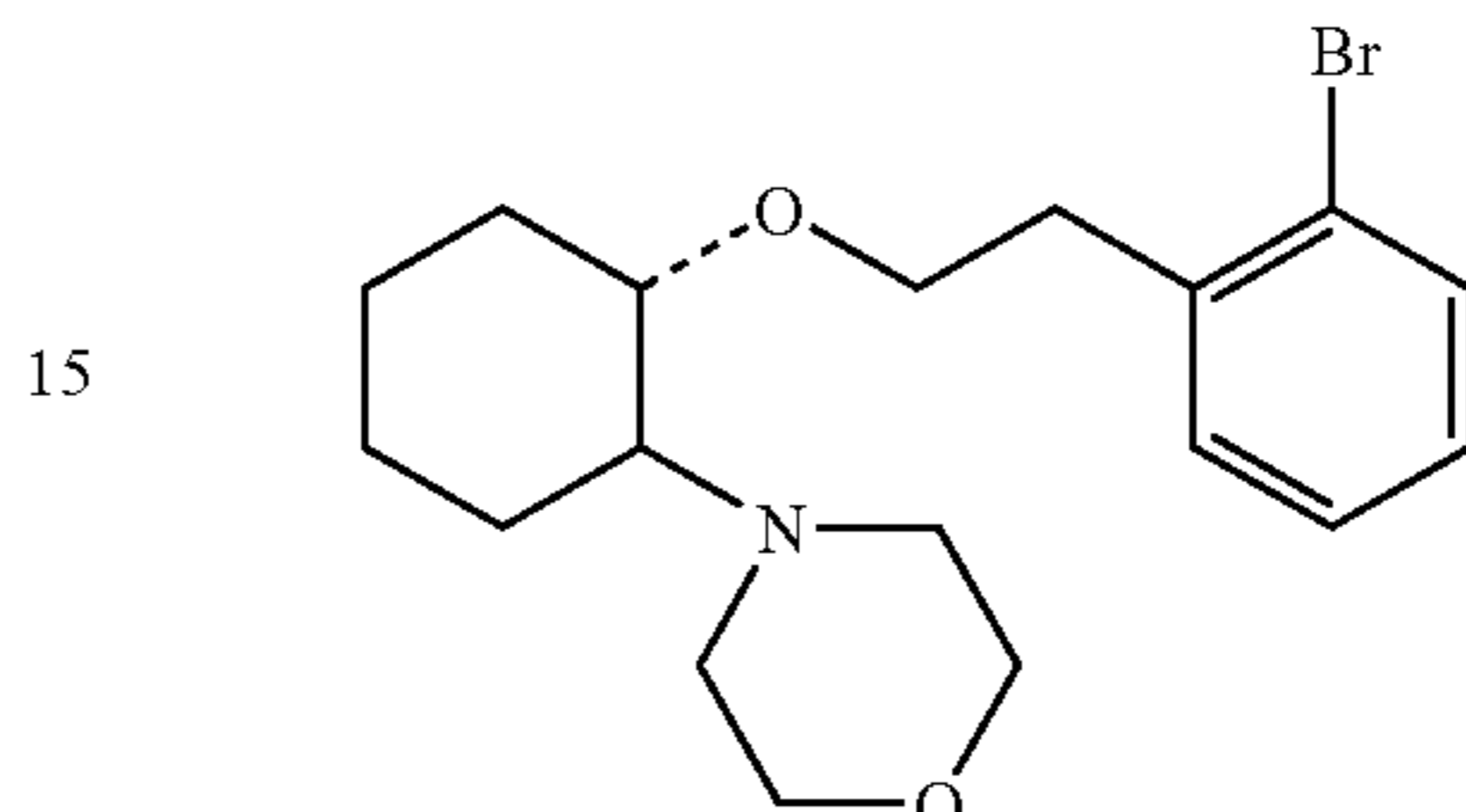
(1R,2R)/(1S,2S)-[2-(4-morpholinyl)-1-(2-bromophenethoxy)]cyclohexane
