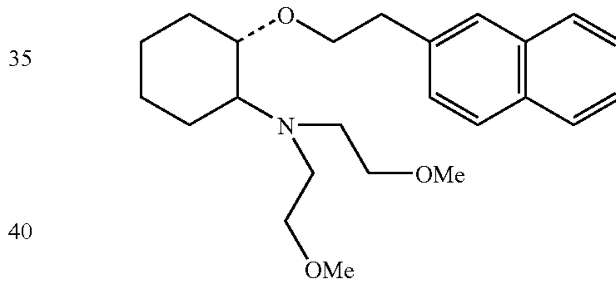
(1R,2R)/(1S,2S)-[2-[bis(2-methoxyethyl)aminyl]-1-(2-naphthenethoxy)]cyclohexane
