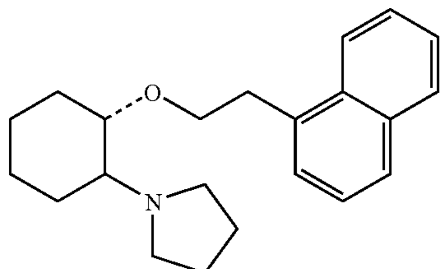
(1R,2R)/(1S,2S)-[2-(1-pyrrolidinyl)-1-(1-naphthenethoxy)]cyclohexane
