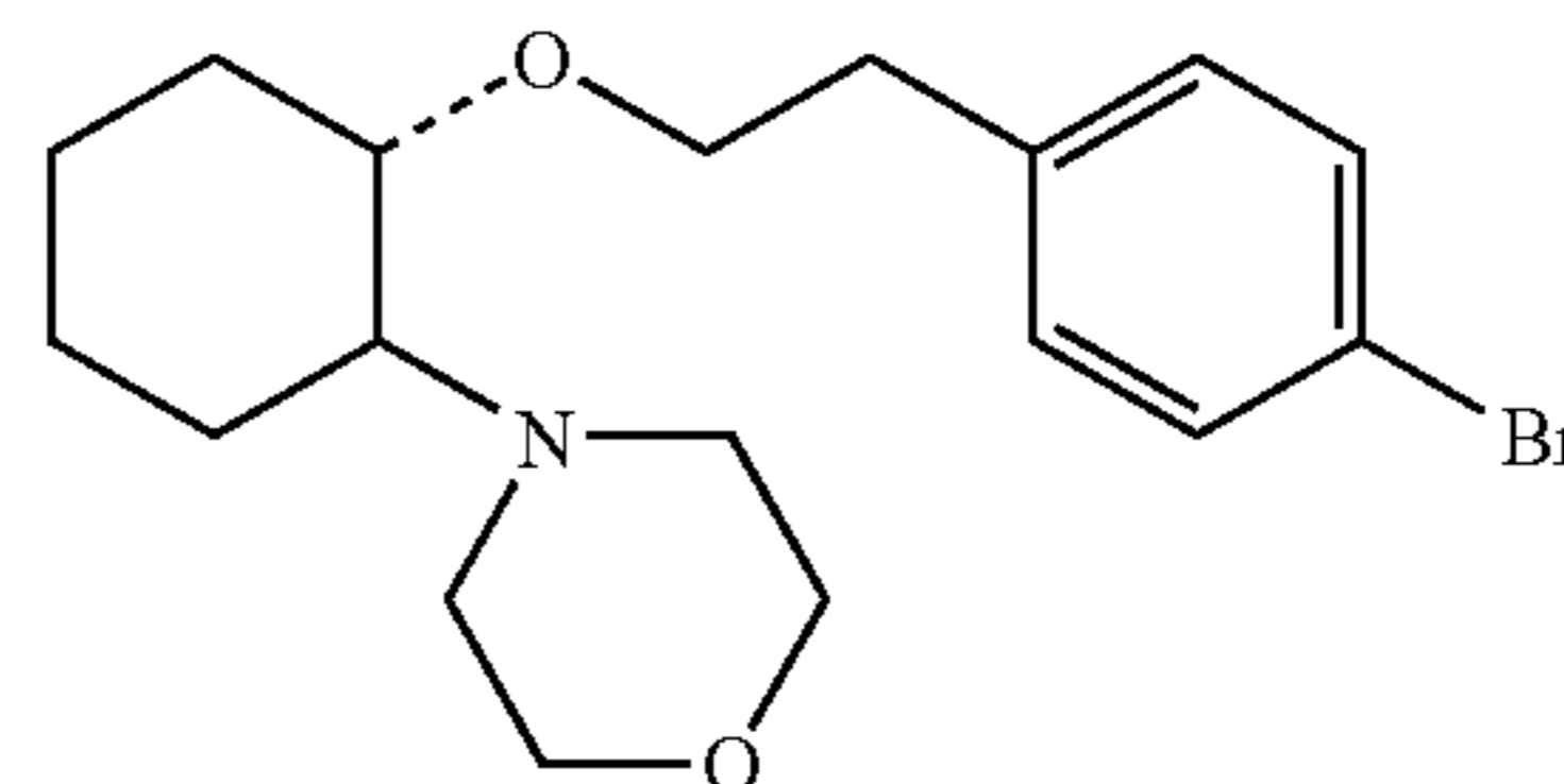
(1R,2R)/(1S,2S)-[2-(4-morpholinyl)-1-(4-bromophenethoxy)]cyclohexane
