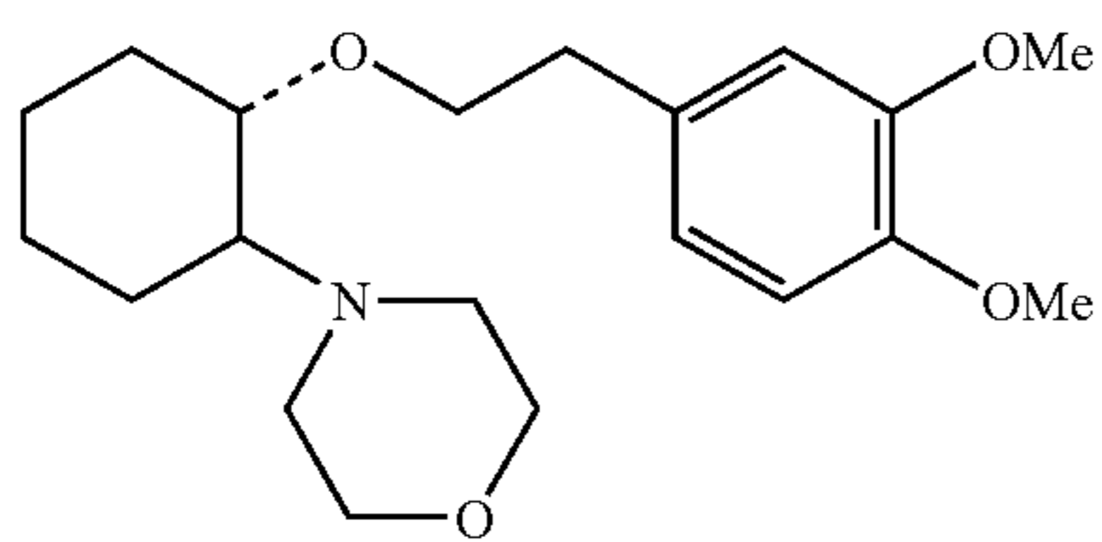
(1R,2R)/(1S,2S)-[2-(4-morpholinyl)-1-[2-(3,4-dimethoxyphenoxy)ethoxy]]cyclohexane
