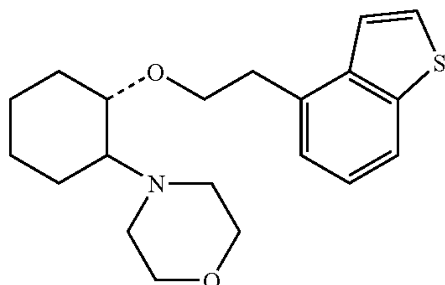
(1R,2R)/(1S,2S)-[2-(4-morpholinyl)-1-(2-benzo[b]thiophen-4-yl)]cyclohexane
