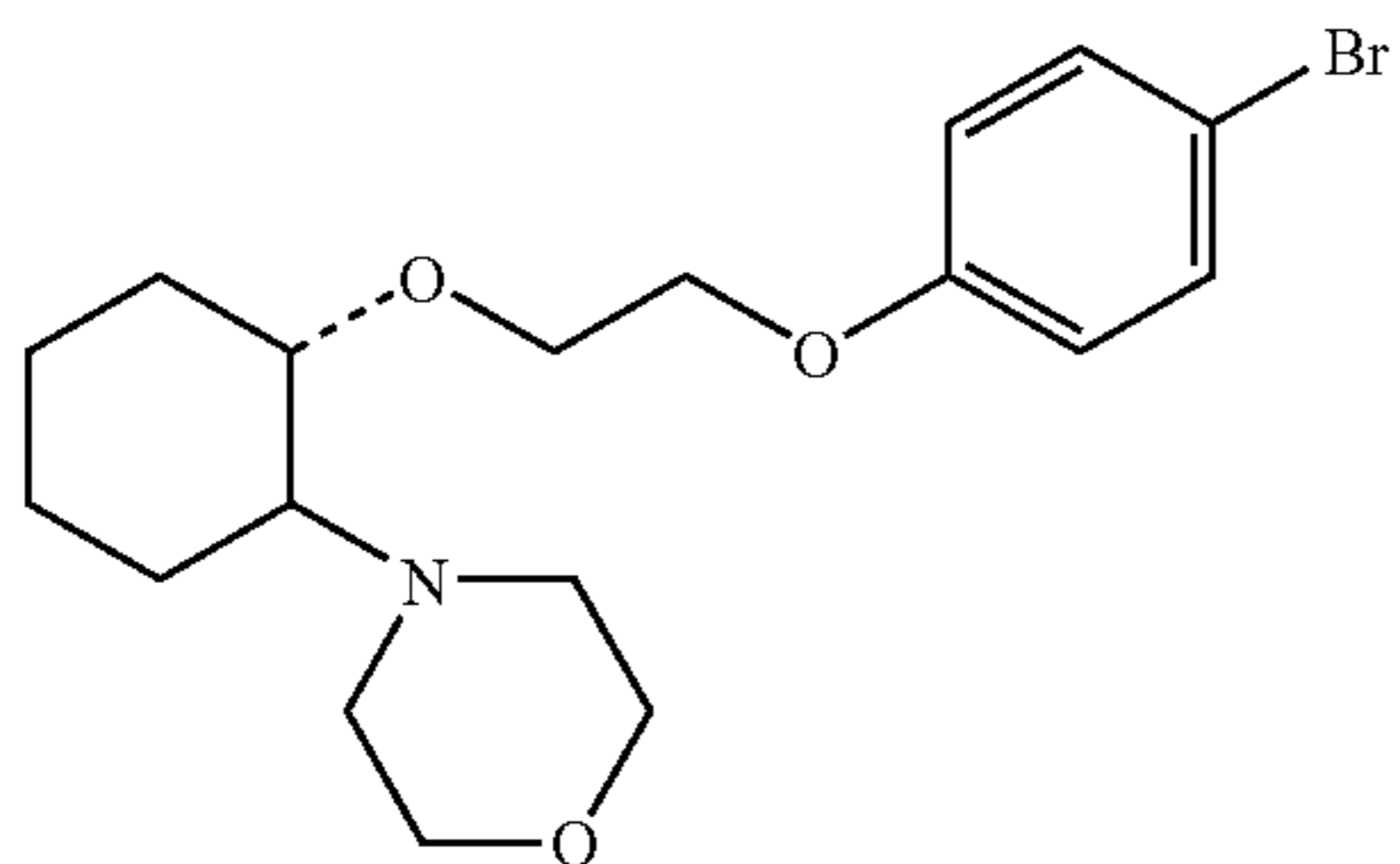
(1R,2R)/(1S,2S)-[2-(4-morpholinyl)-1-[2-(4-bromophenoxy)ethoxy]]cyclohexane
