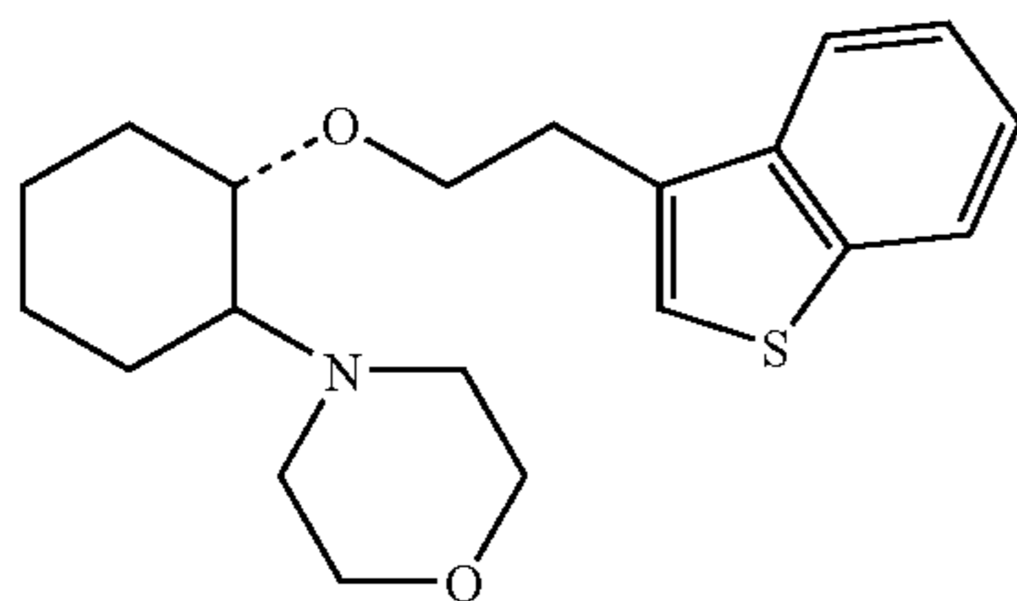
(1R,2R)/(1S,2S)-[2-(4-morpholinyl)-1-(2-benzo[b]thiophen-3-yl)]cyclohexane
