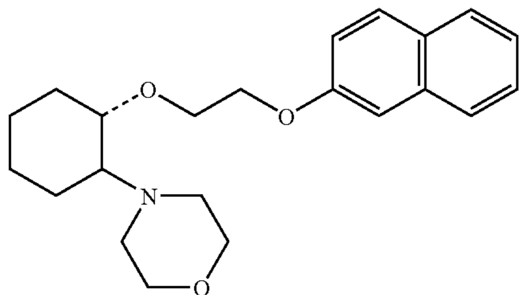
(1R,2R)/(1S,2S)-[2-(4-morpholinyl)-1-[2-(2-naphthoxy)ethoxy]]cyclohexane
