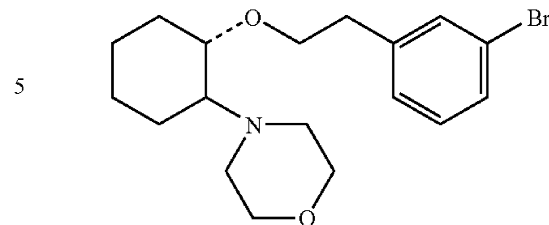
(1R,2R)/(1S,2S)-[2-(4-morpholinyl)-1-(3-bromophenethoxy)]cyclohexane
