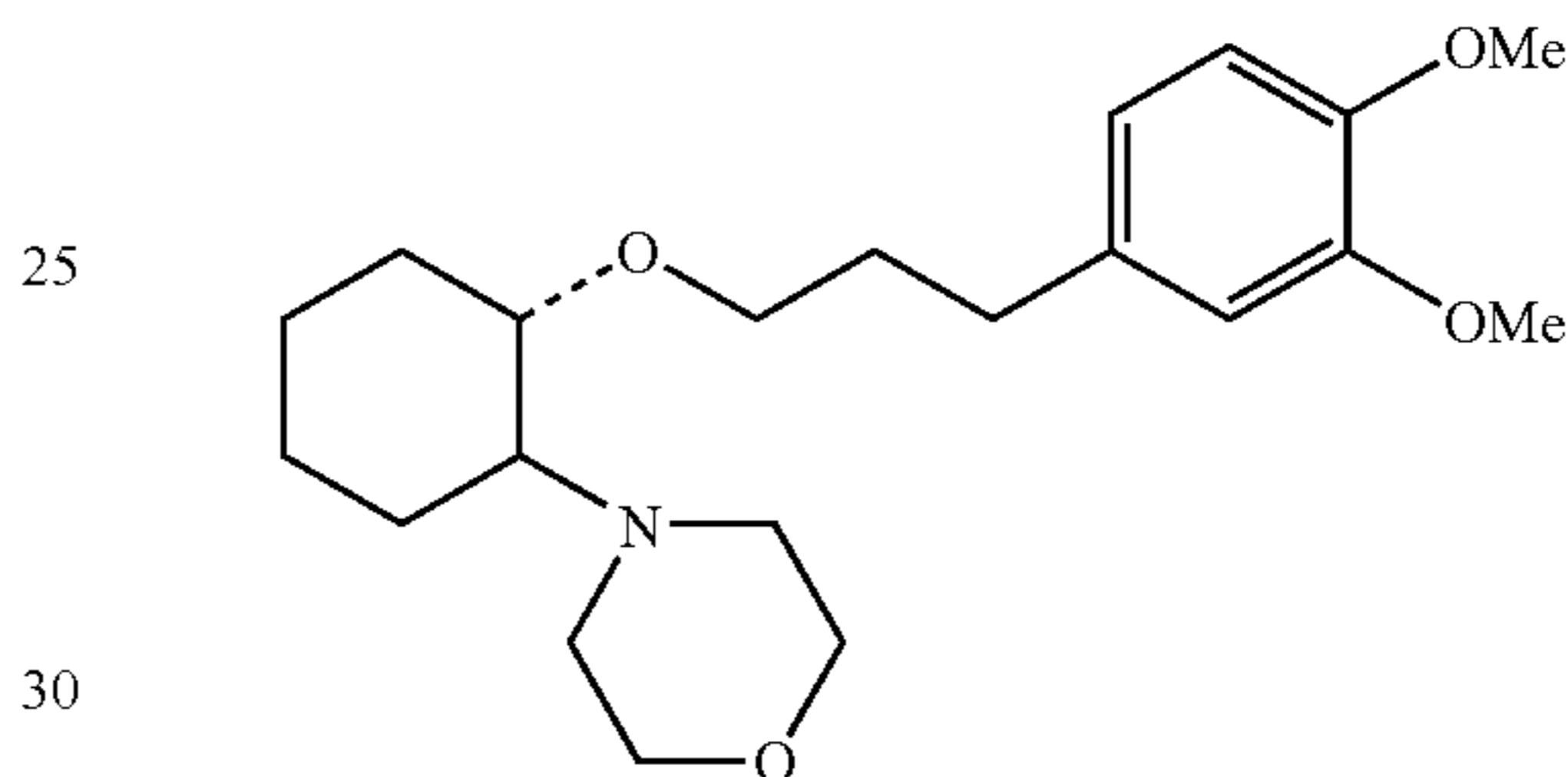
(1R,2R)/(1S,2S)-[2-(4-morpholinyl)-1-(3-(3,4-dimethoxyphenyl)propoxy)]cyclohexane
