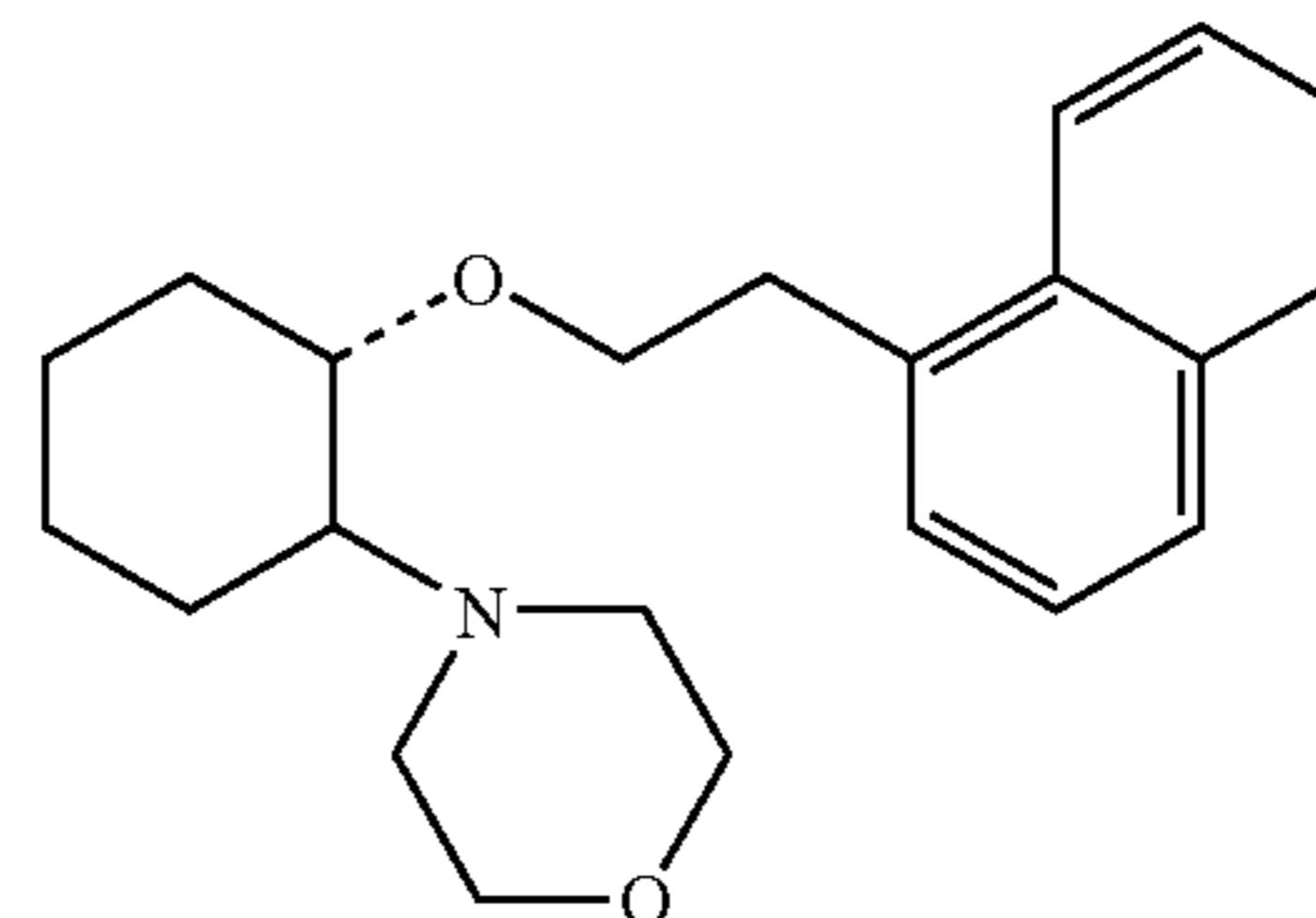
(1R,2R)/(1S,2S)-[2-(4-morpholinyl)-1-(1-naphthenethoxy)]cyclohexane
