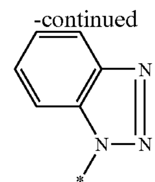
benzotriazole
