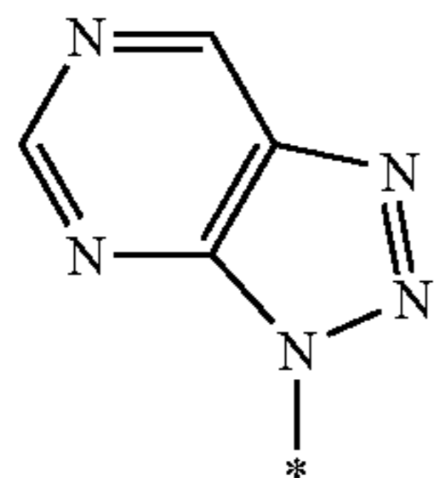
pyrimidinotriazole
