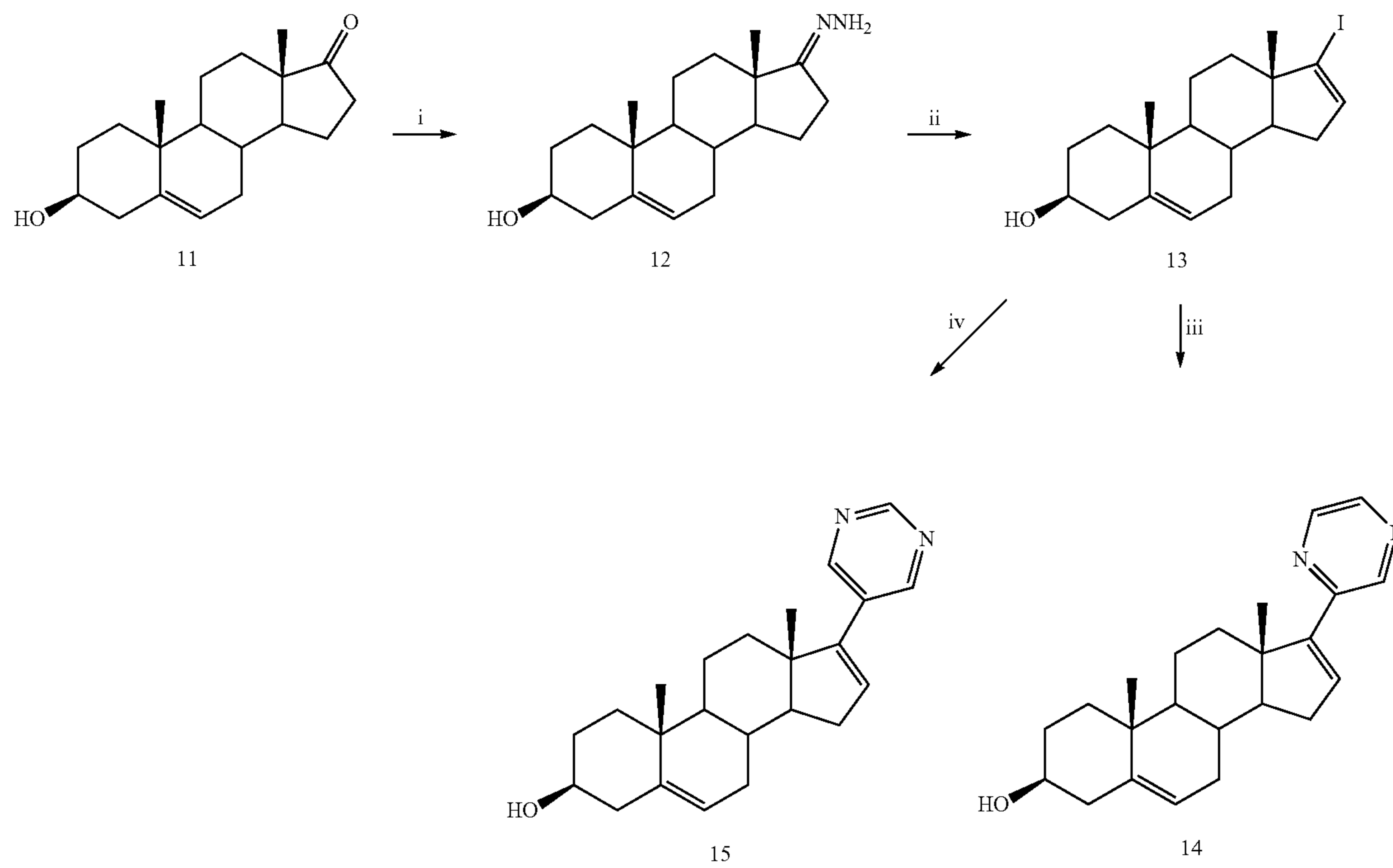
Scheme 2:
