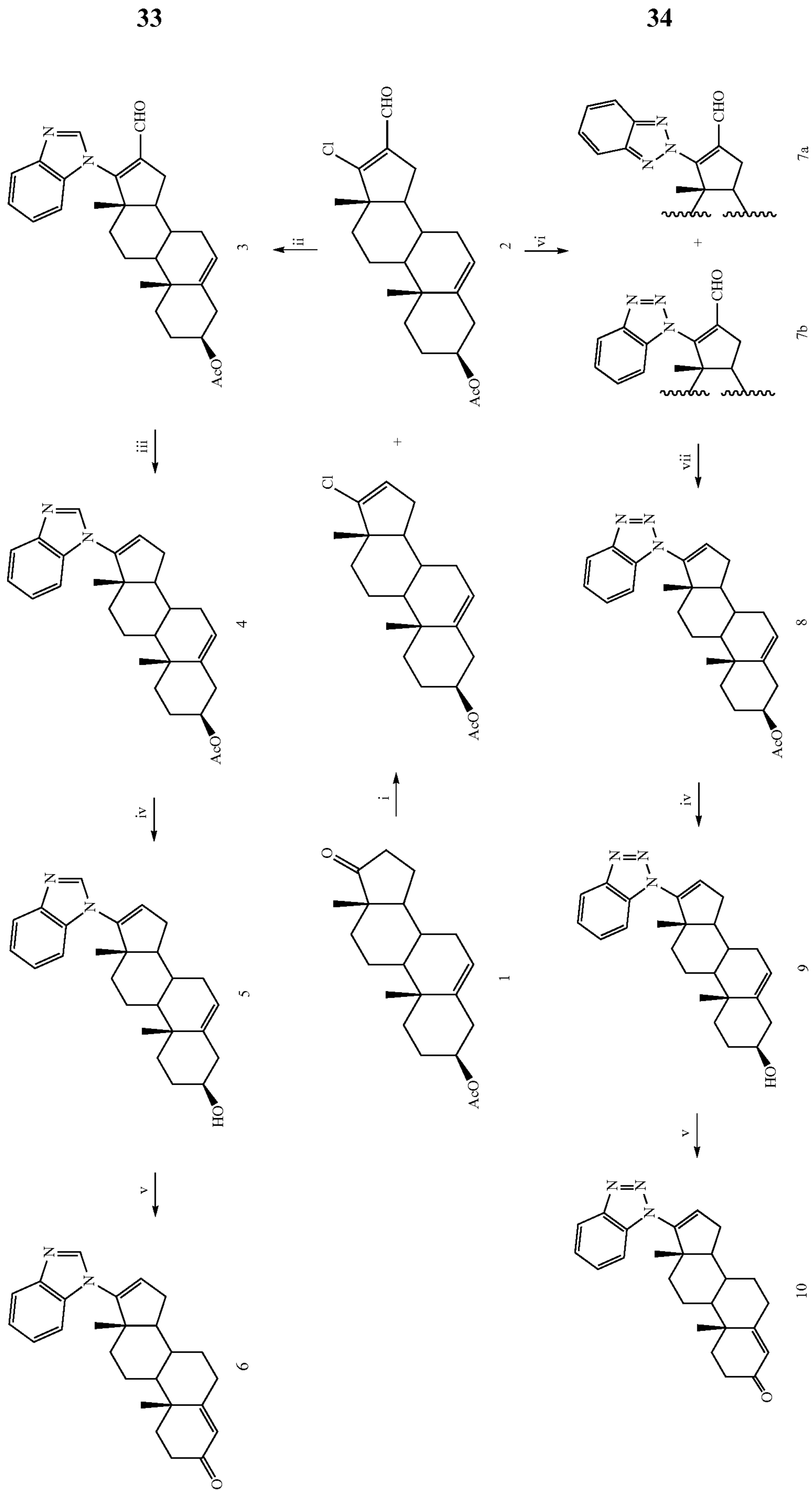
Scheme 1.
