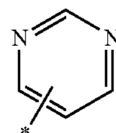
pyrimidine
