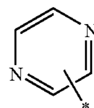
pyrazine
