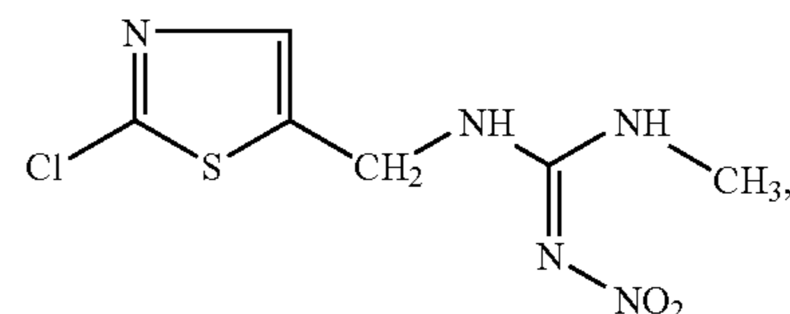
(clothianidin)
