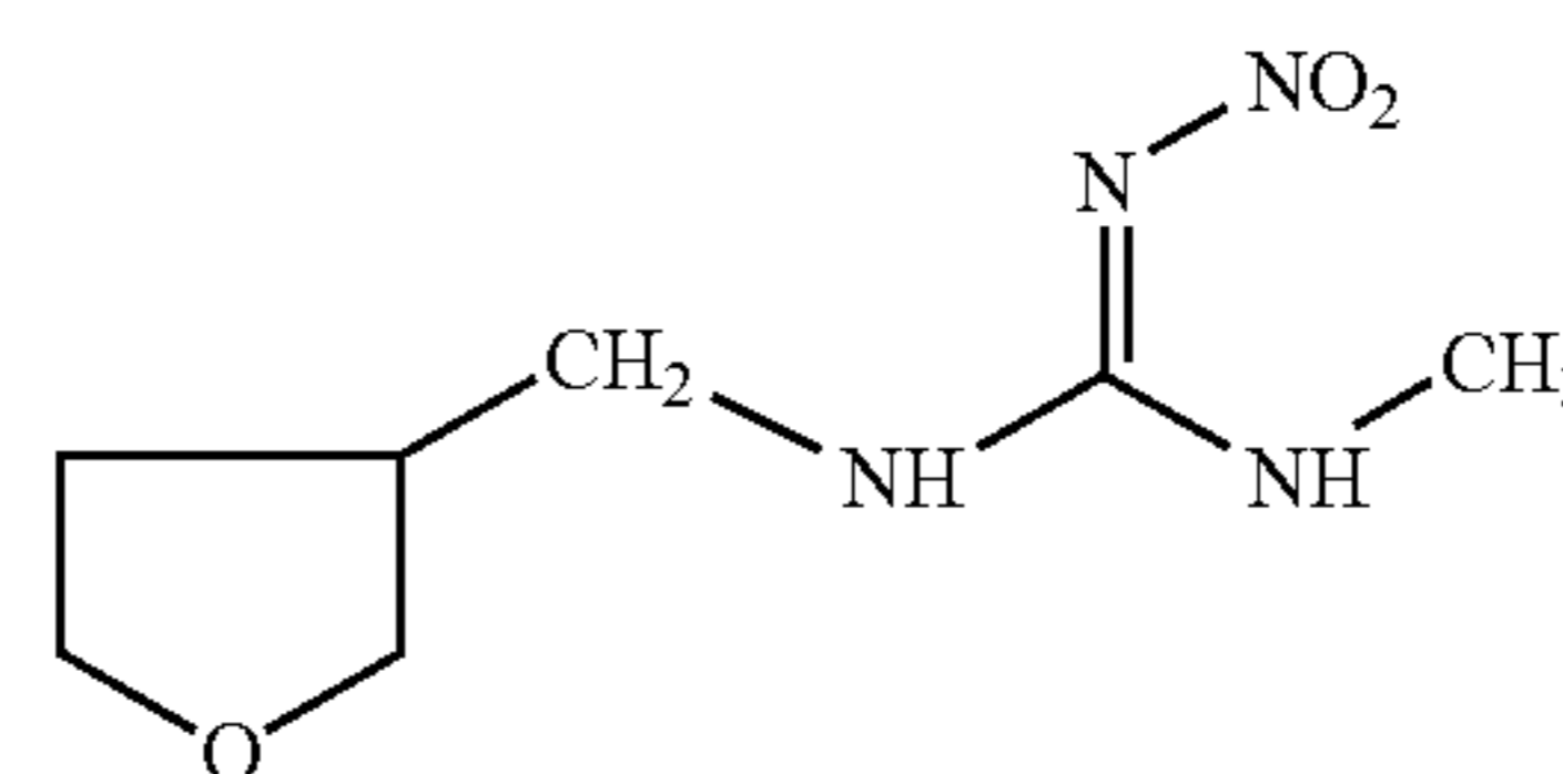
(dinotefuran)
