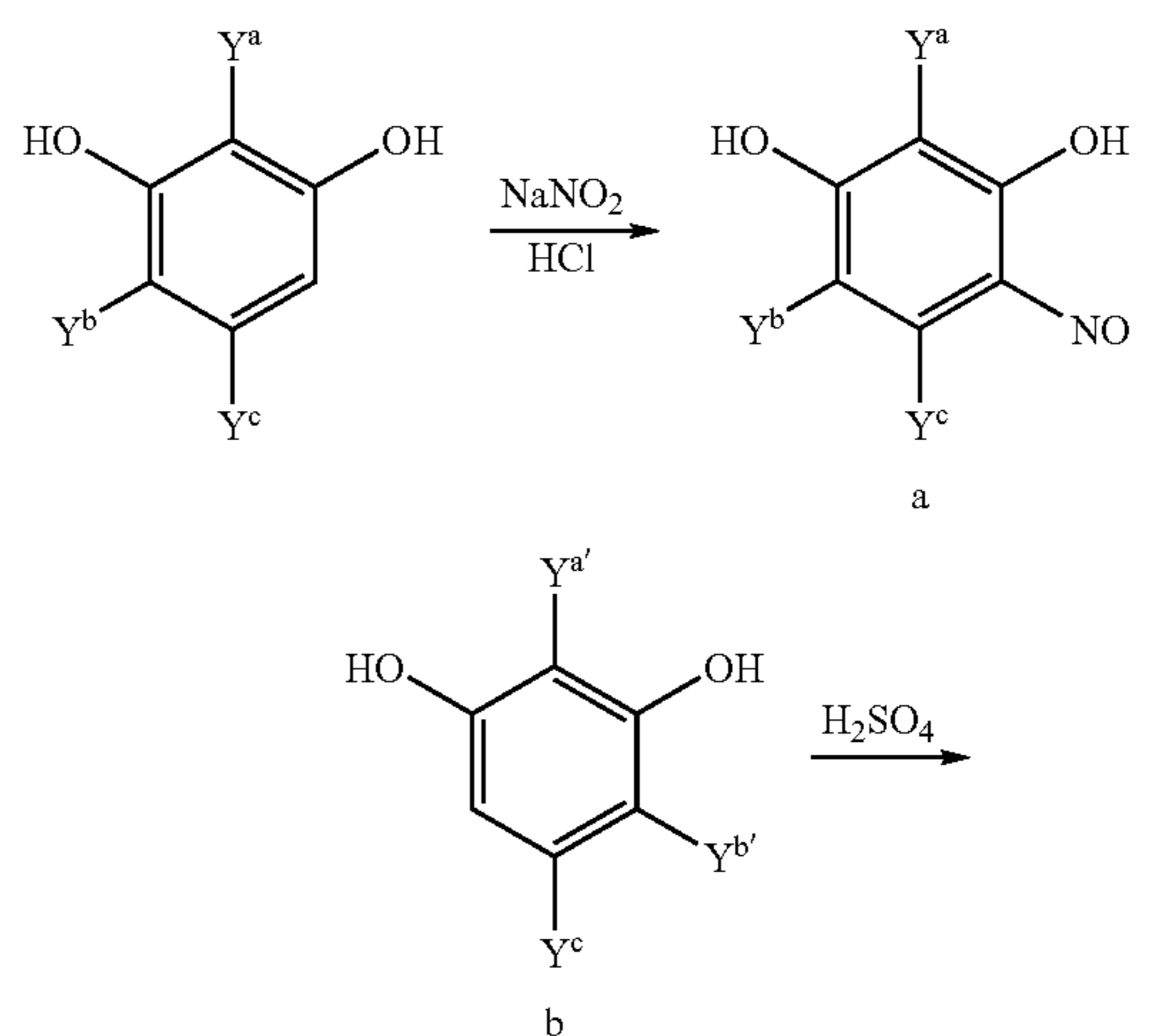
Scheme 1:
