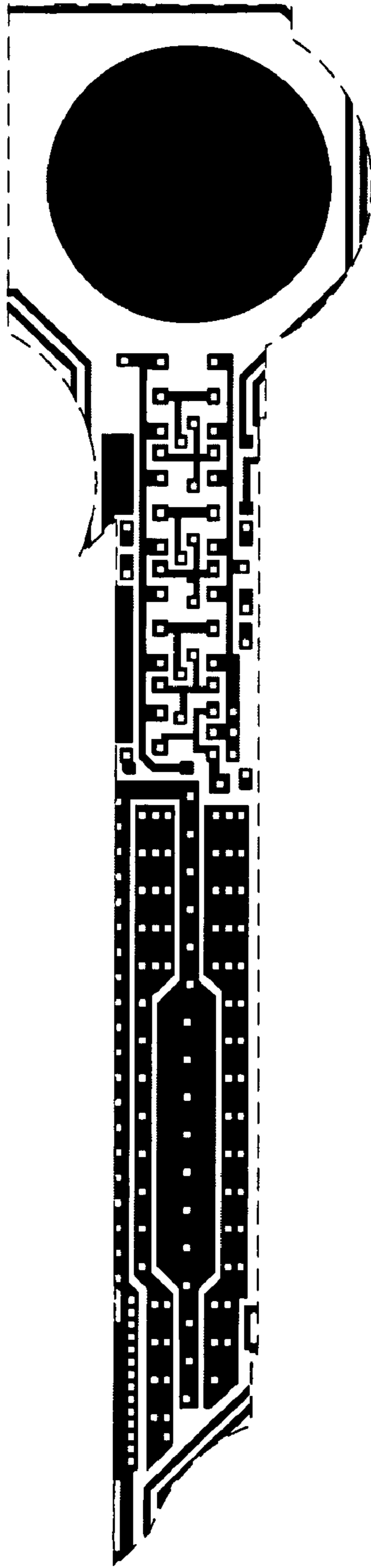
Metal 1 mask
