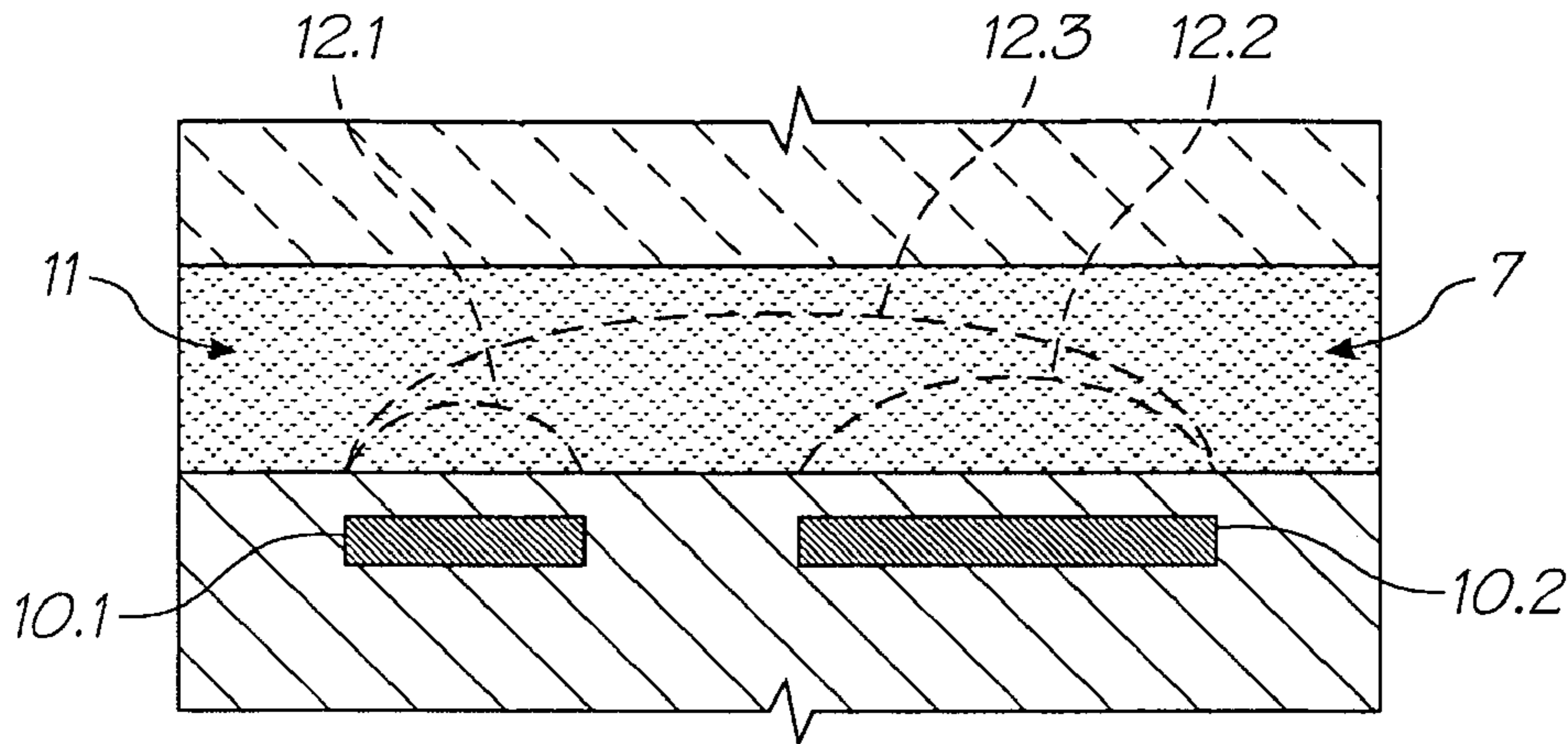
FIG. 52 (PRIOR ART)
