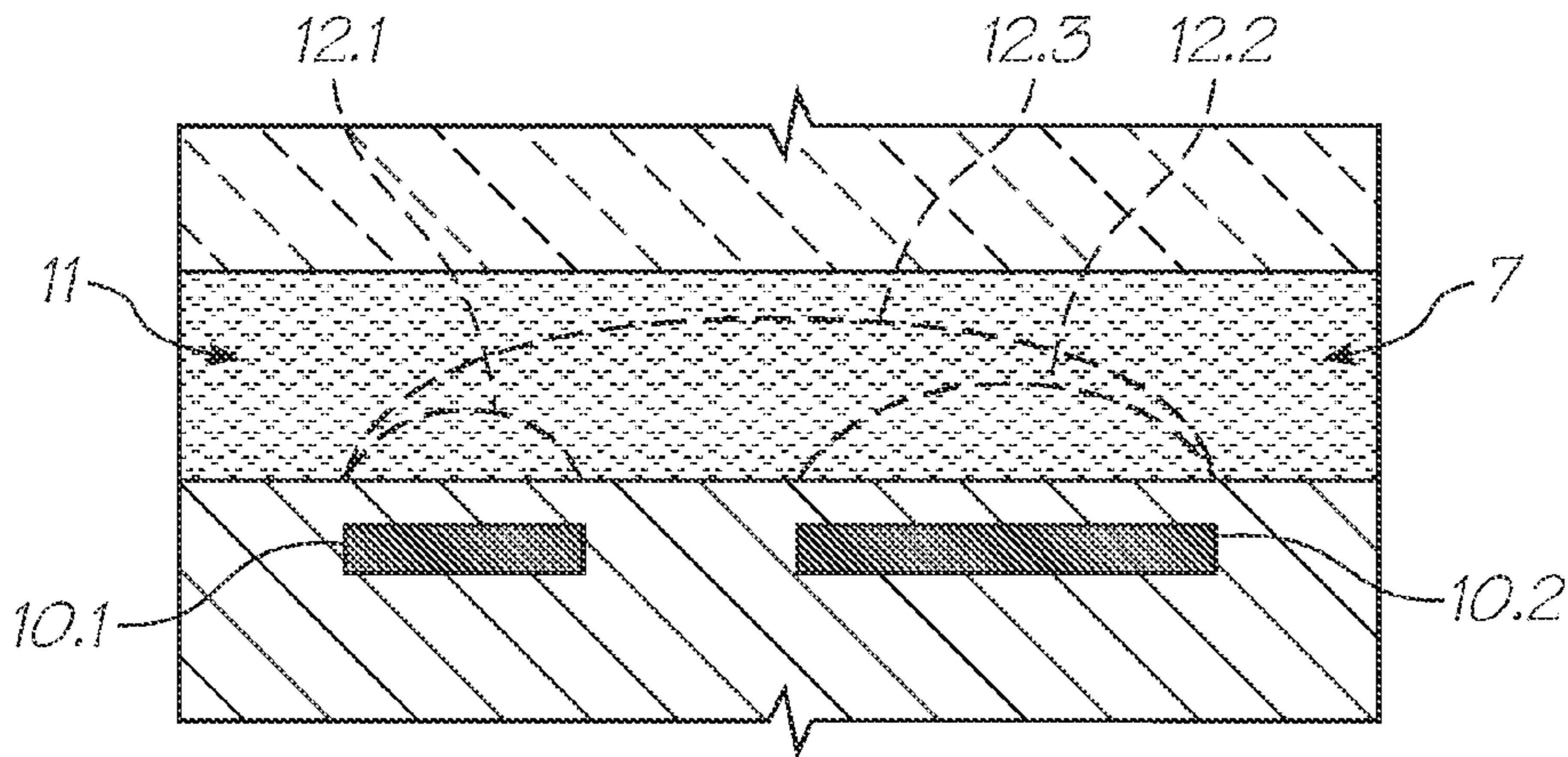
FIG. 52 (PRIOR ART)
