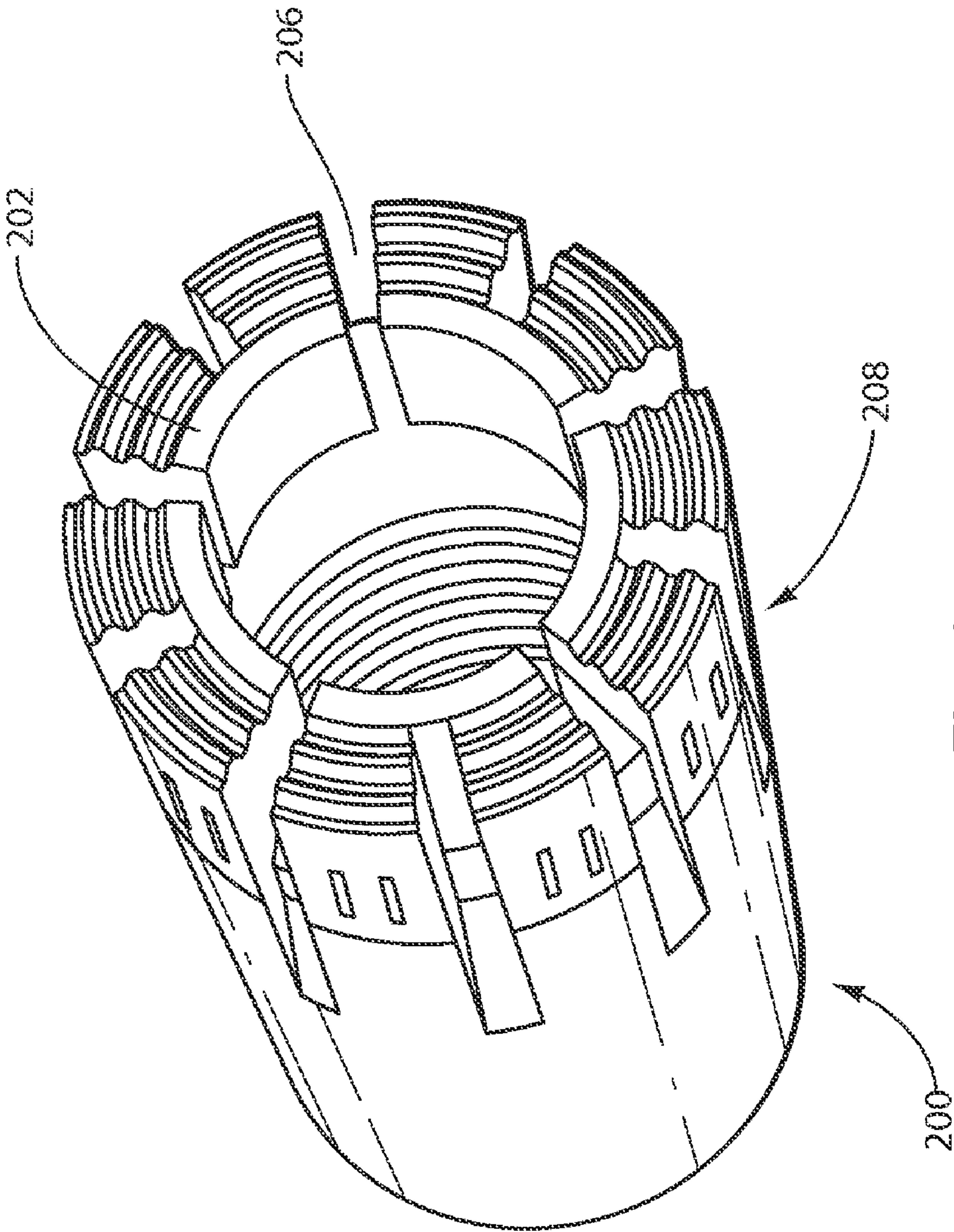
Fig. 1 (Prior Art)
