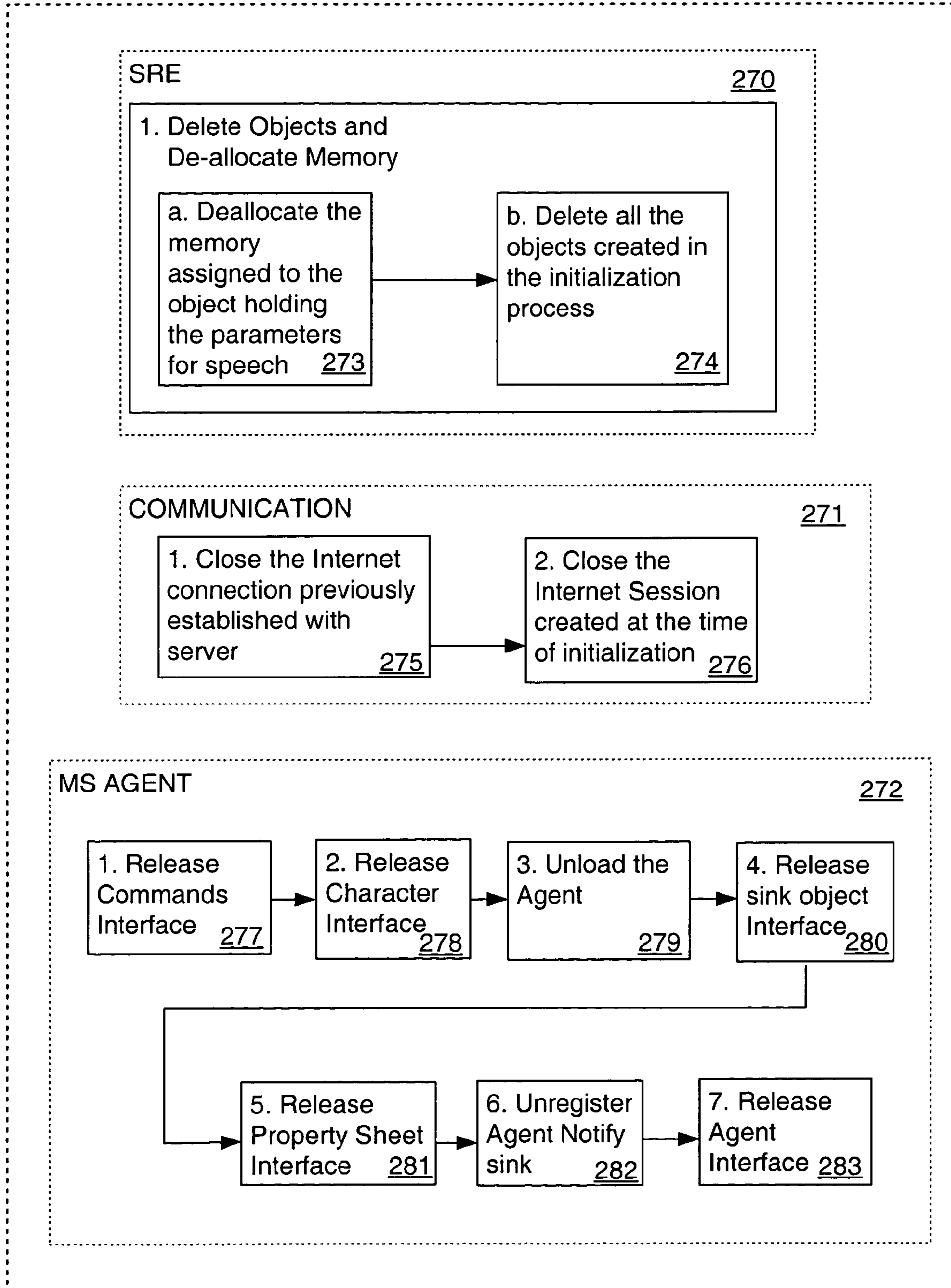
Fig. 4 Client-side Un-Initialization
