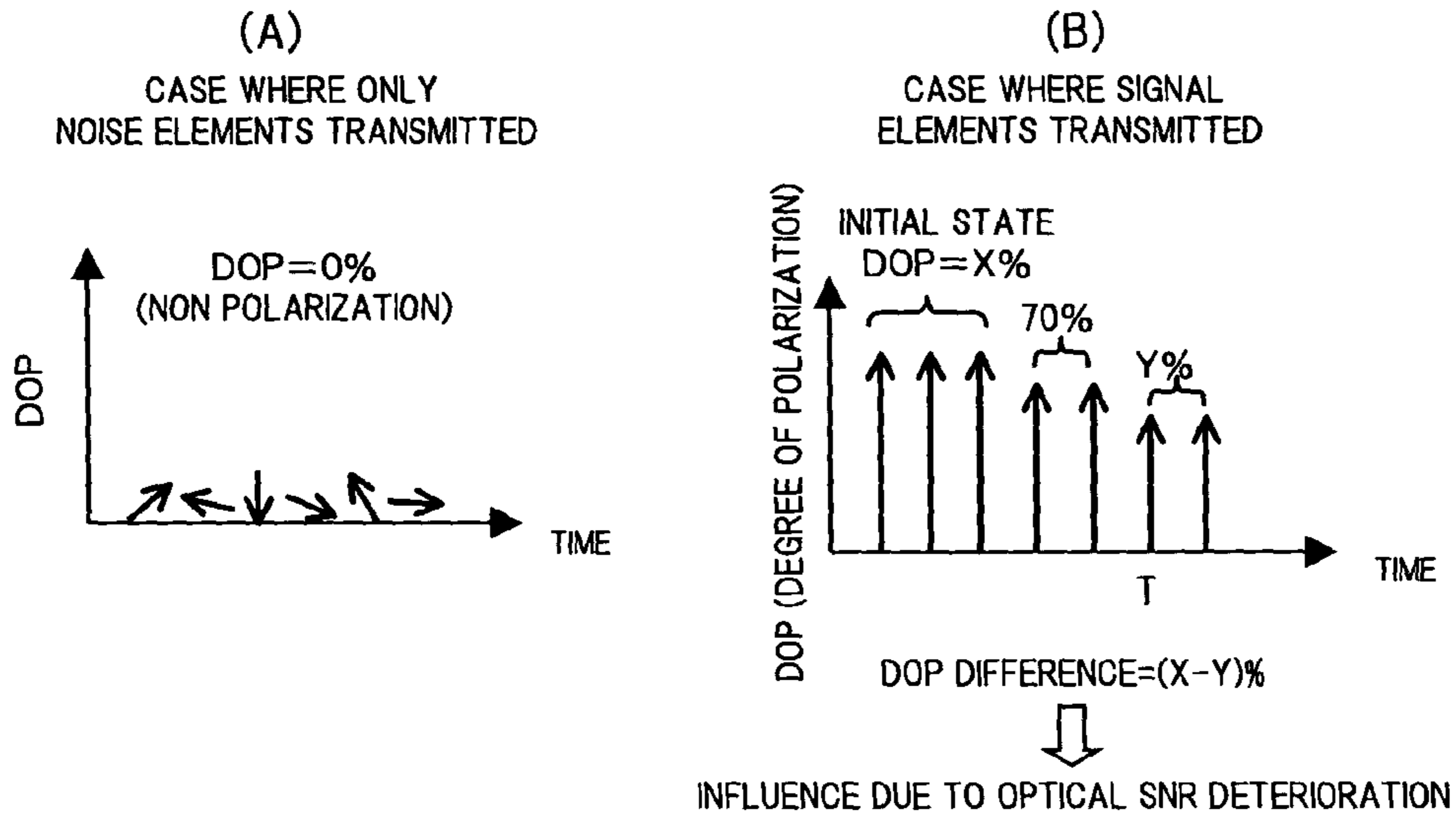
EXAMPLE OF DOP DETERIORATION WITH TIME IN TYPICAL OPTICAL TRANSMISSION SYSTEM
