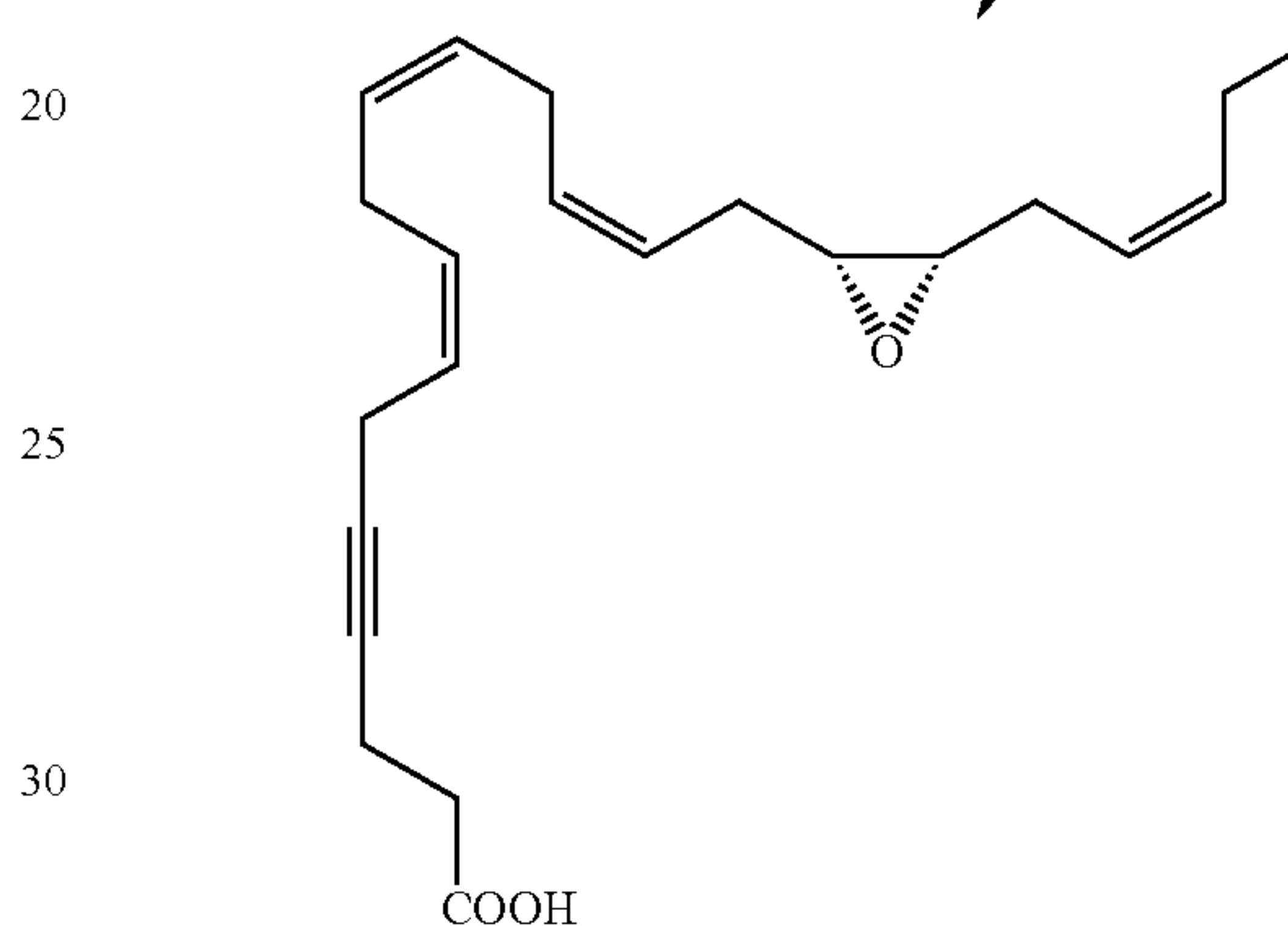
4,5-dehydro 16(17)epoxy-DHA
