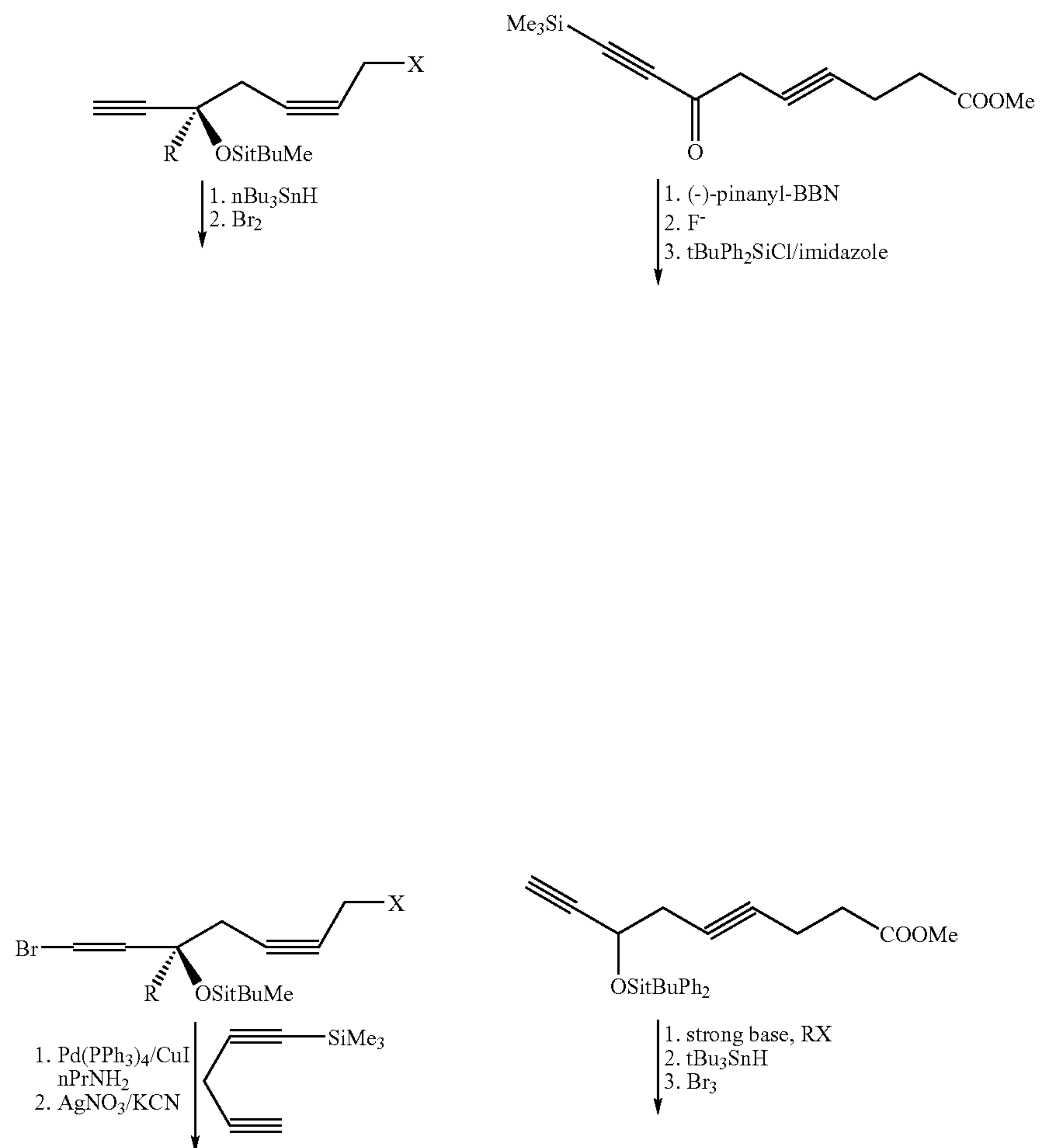
Scheme IV
