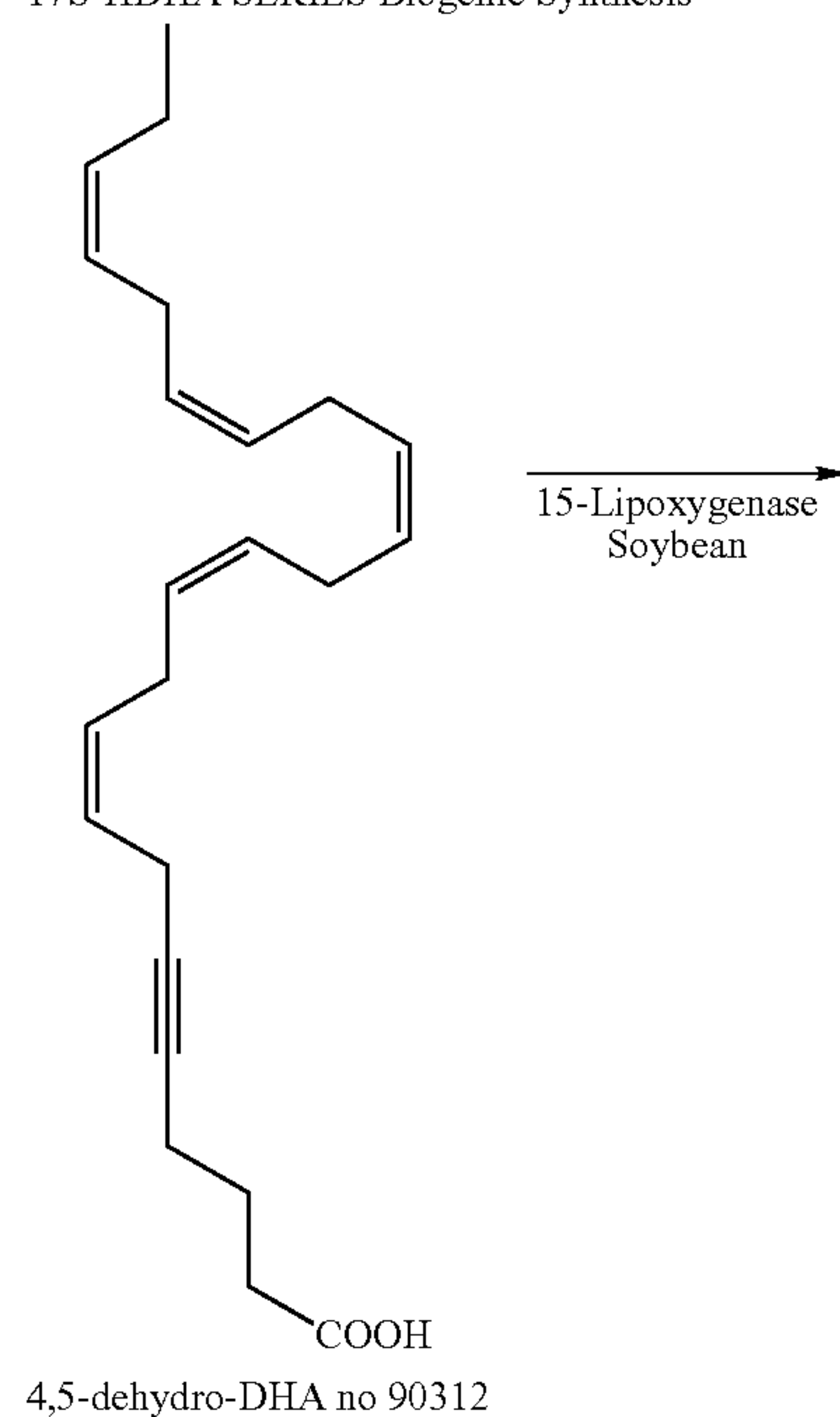
Scheme D
