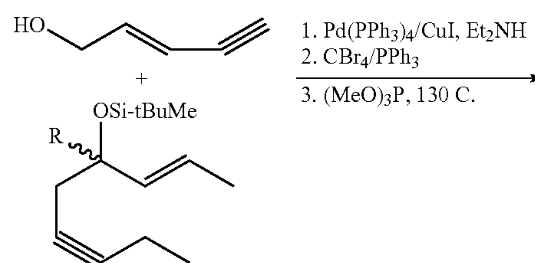
Scheme II
