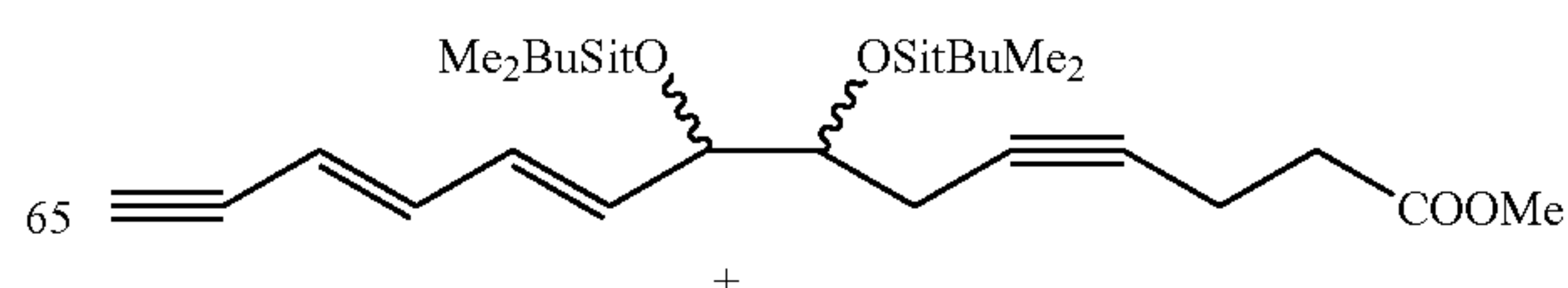
Scheme III
