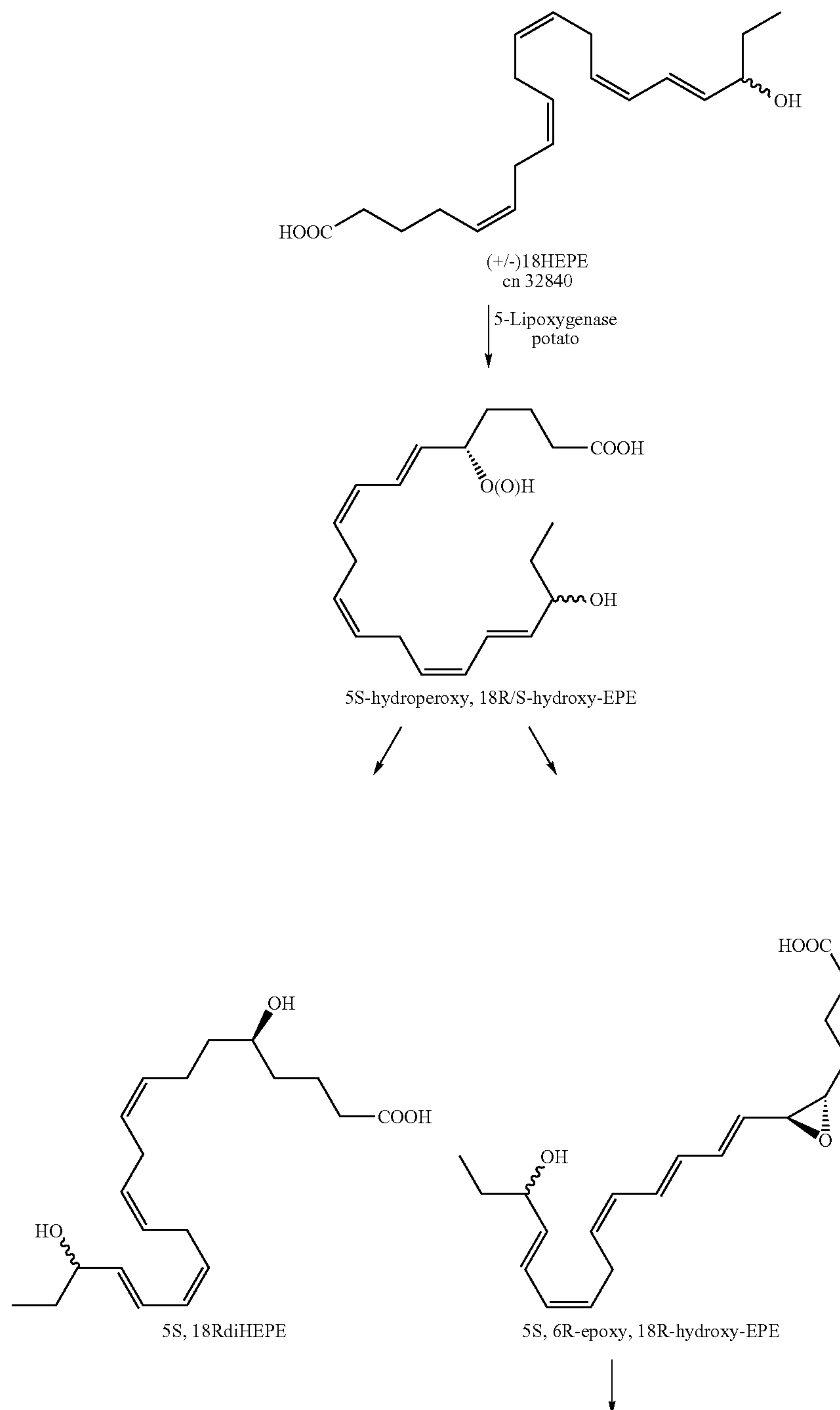
Scheme C
