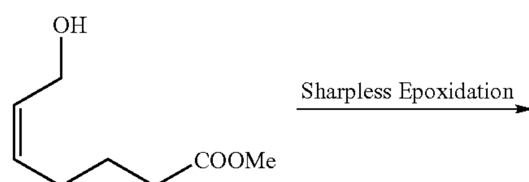
Scheme VII
