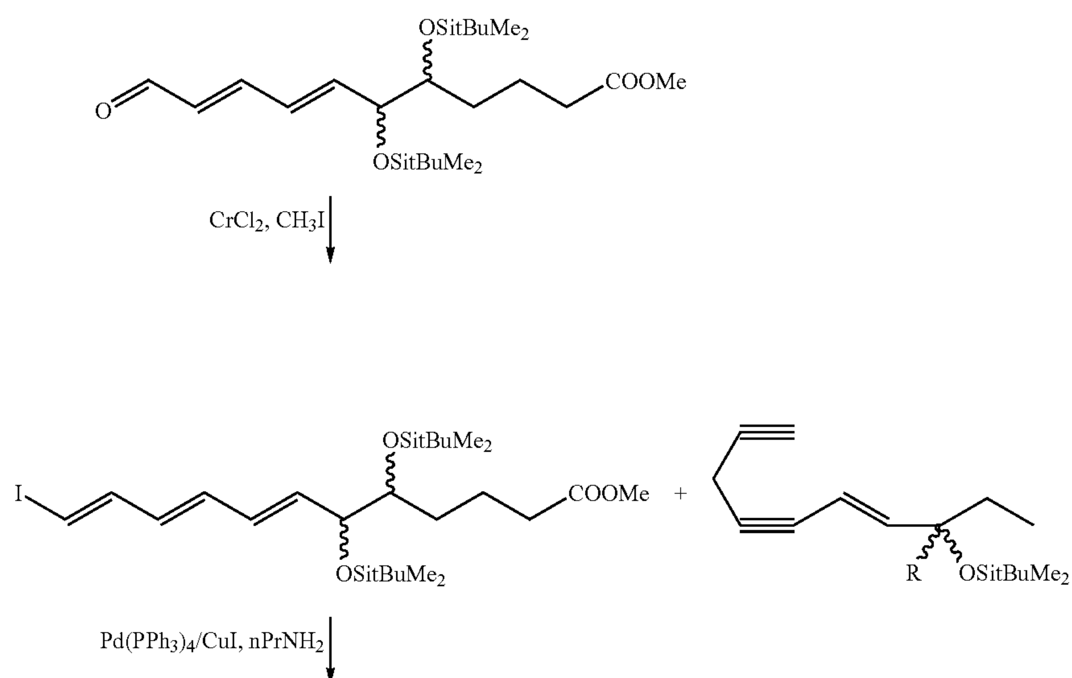
Scheme VIII
