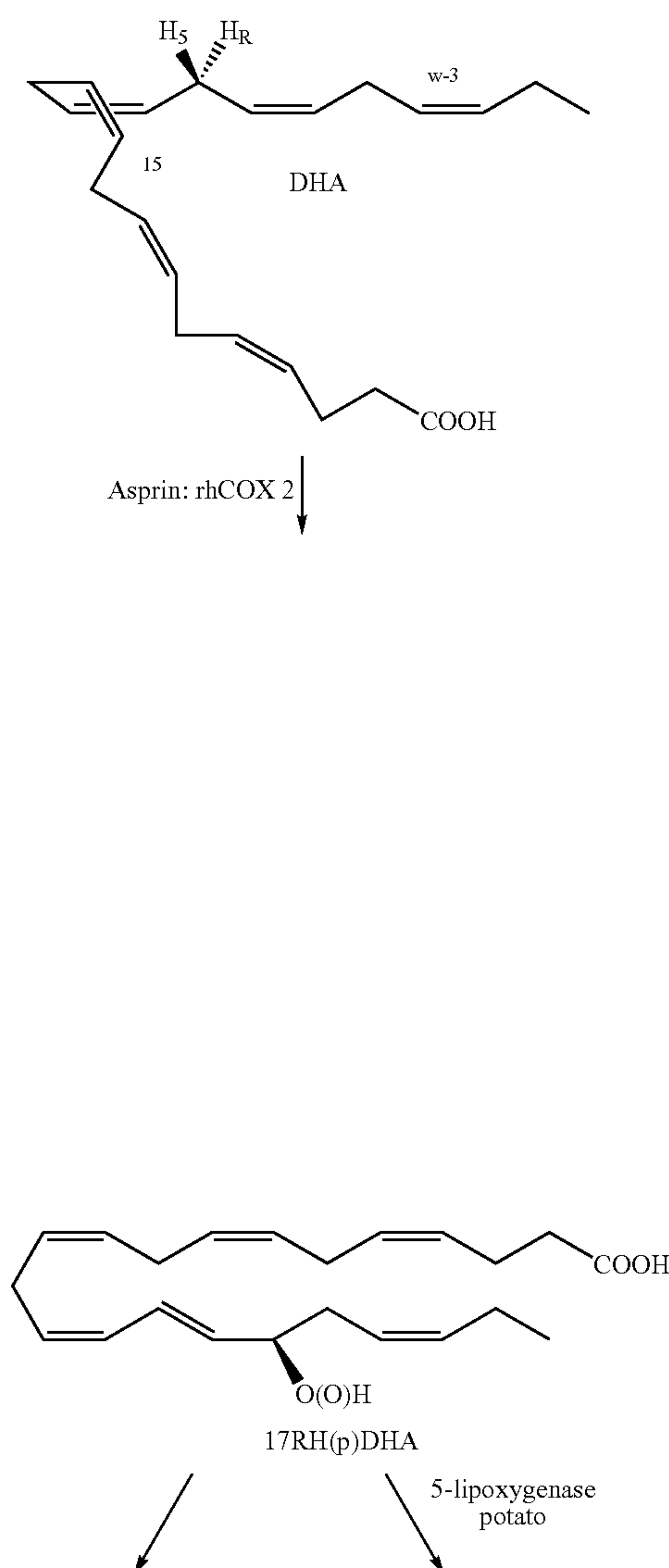
Scheme A
