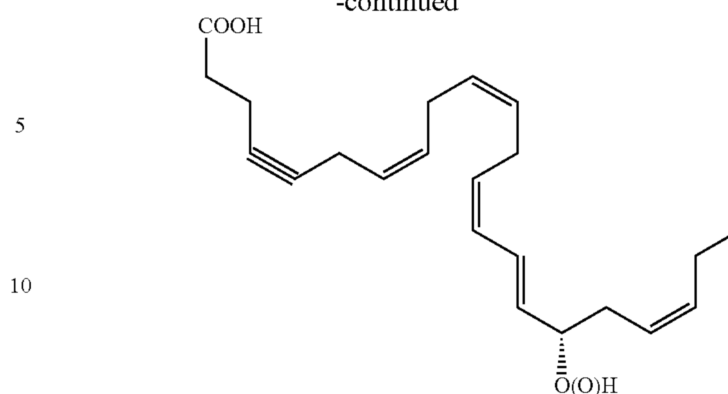
4,5-dehydro-17S-H(p)DHA
