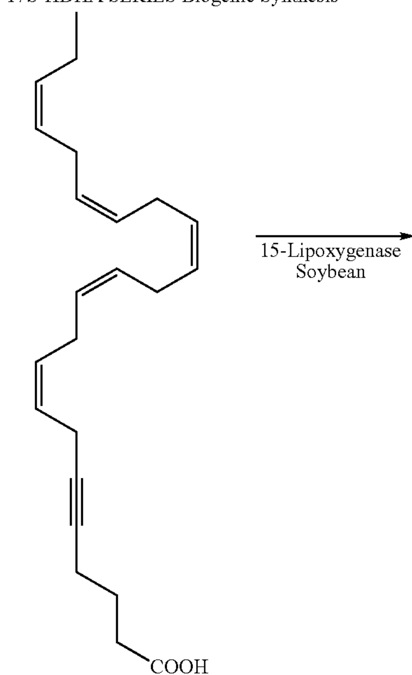
4,5-dehydro-DHA no 90312
