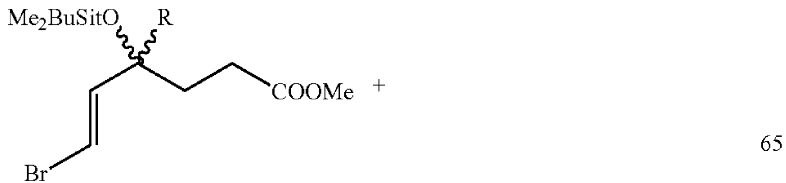
Scheme V Alternative
