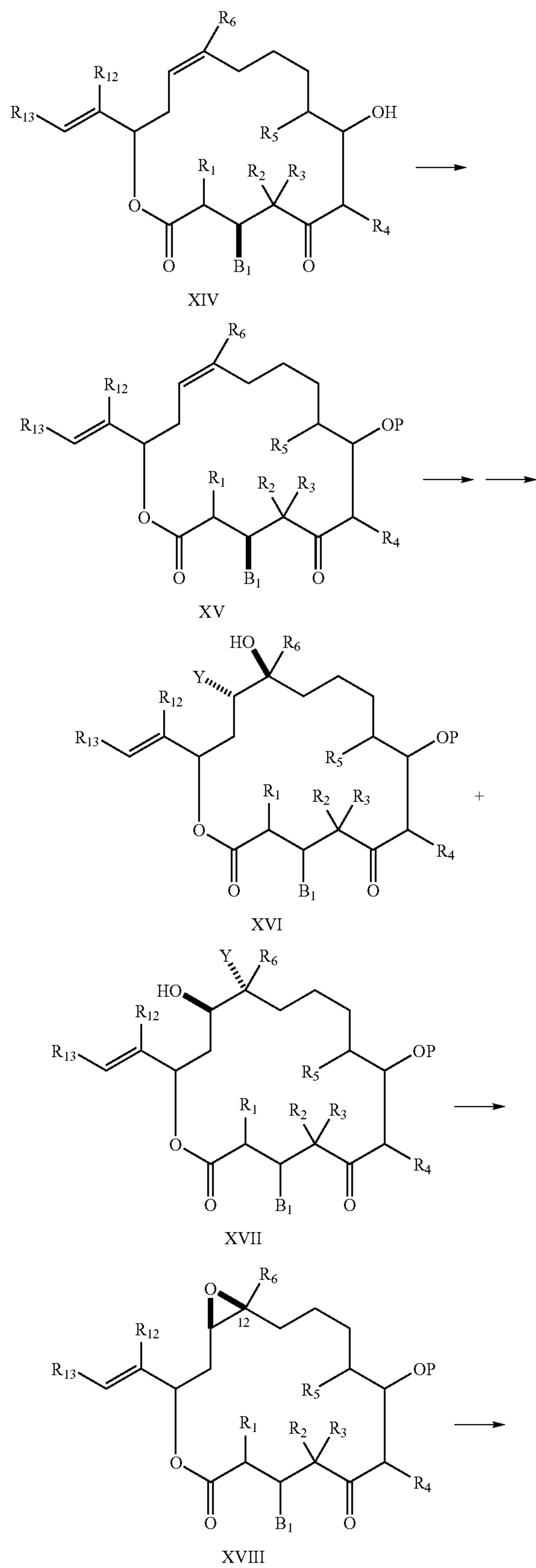
SCHEME 4
