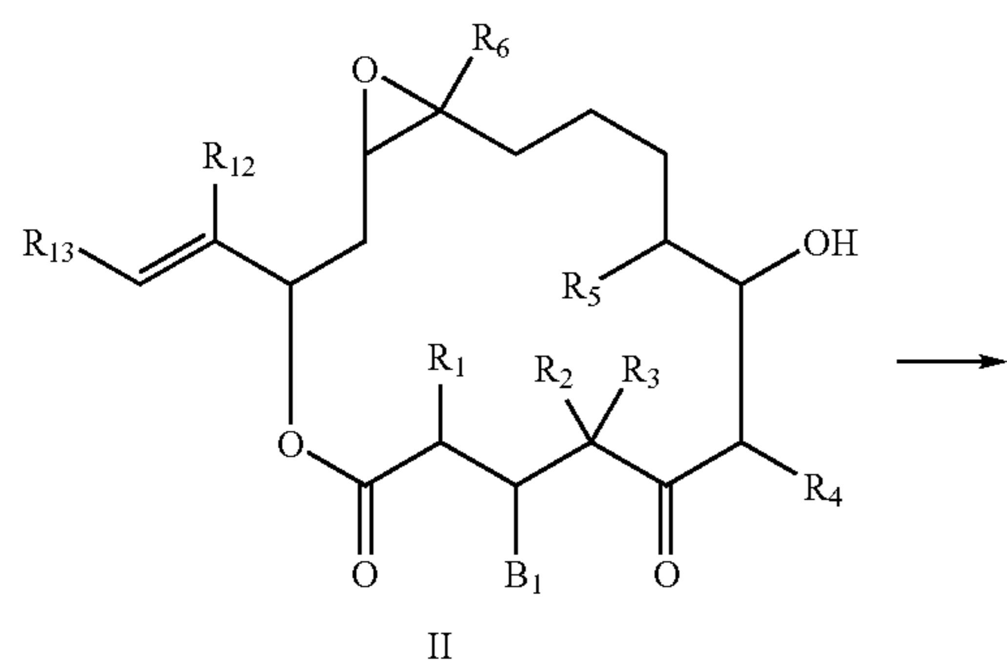
SCHEME 1
