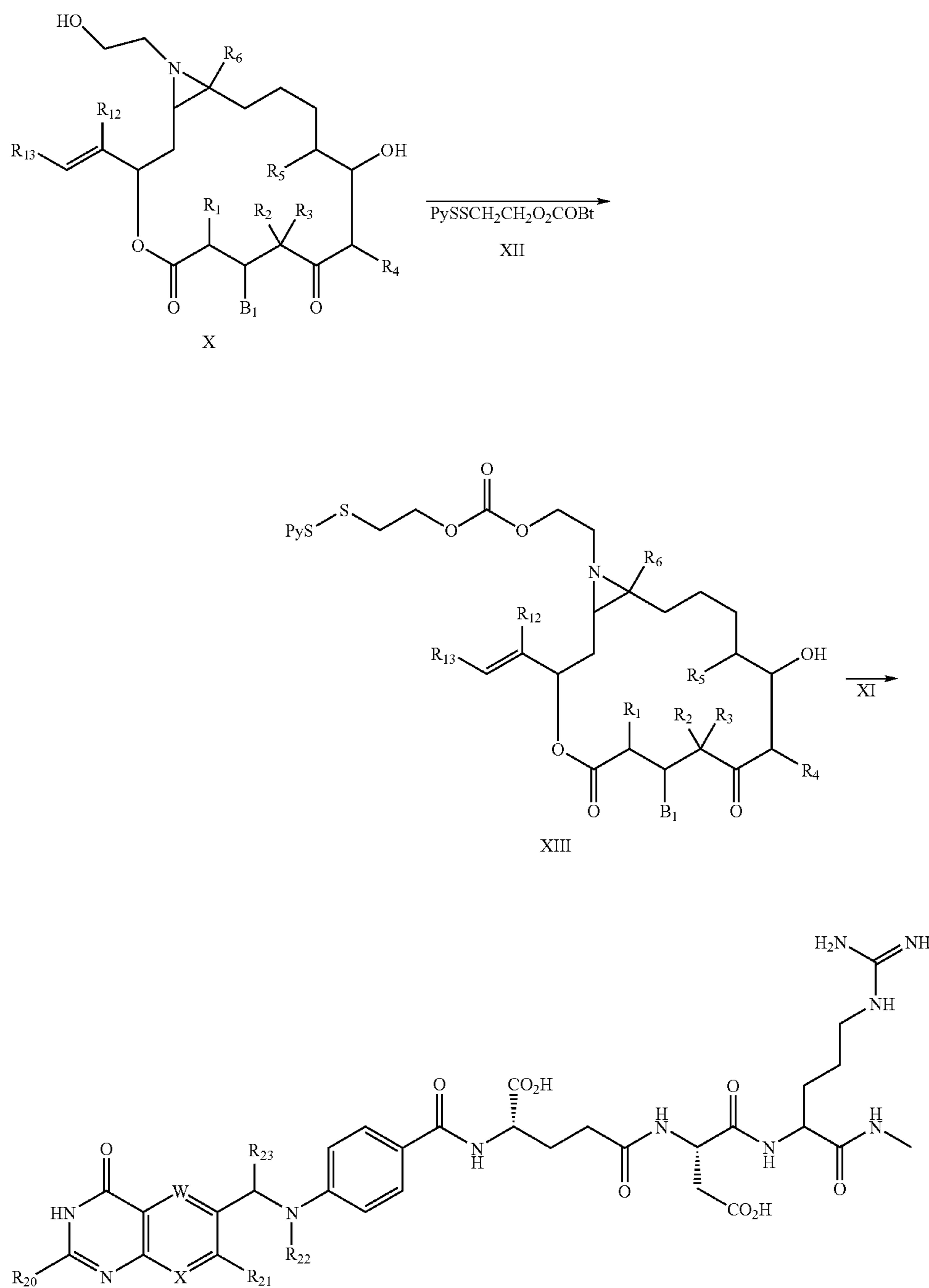
SCHEME 3
