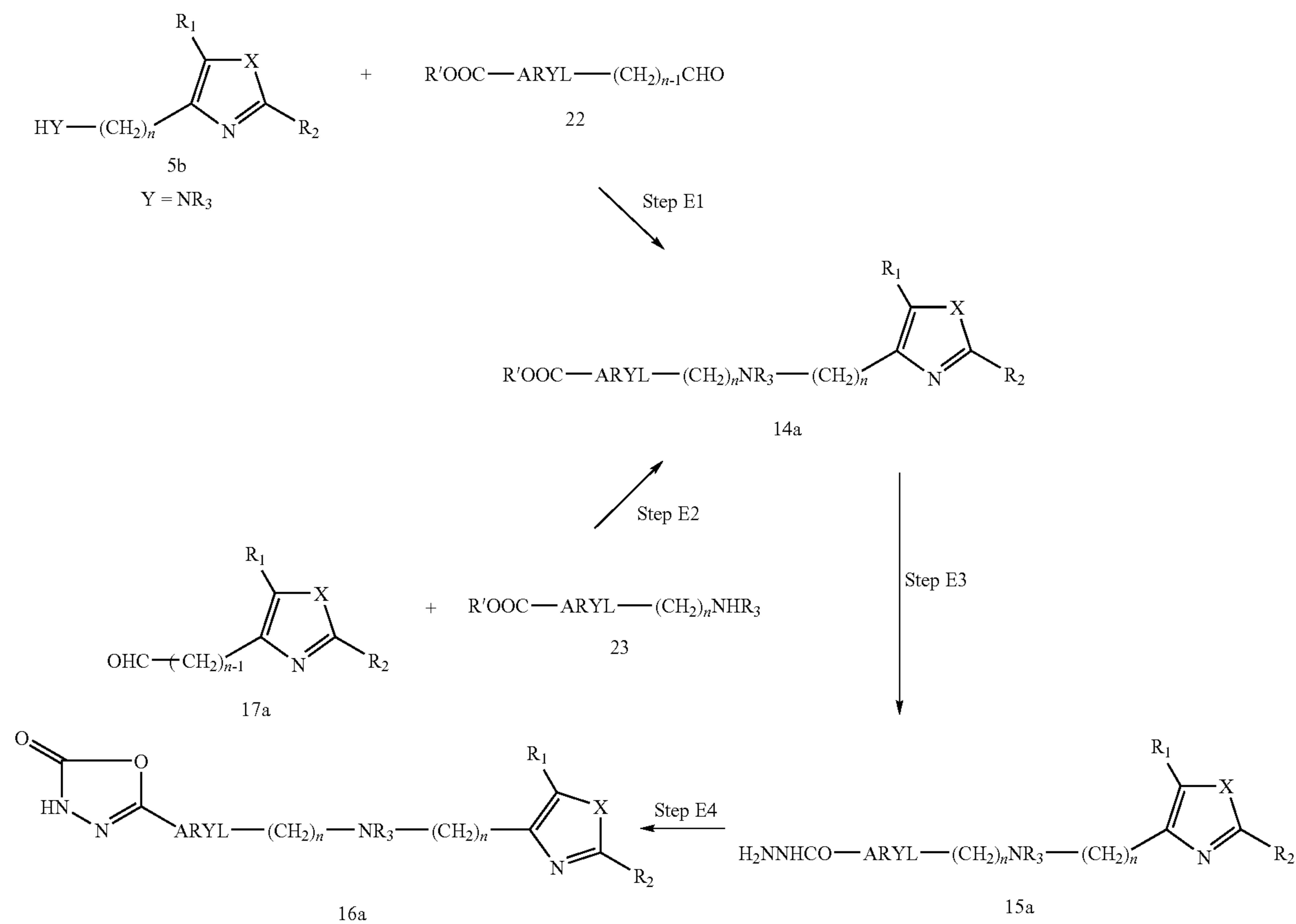
Scheme E
