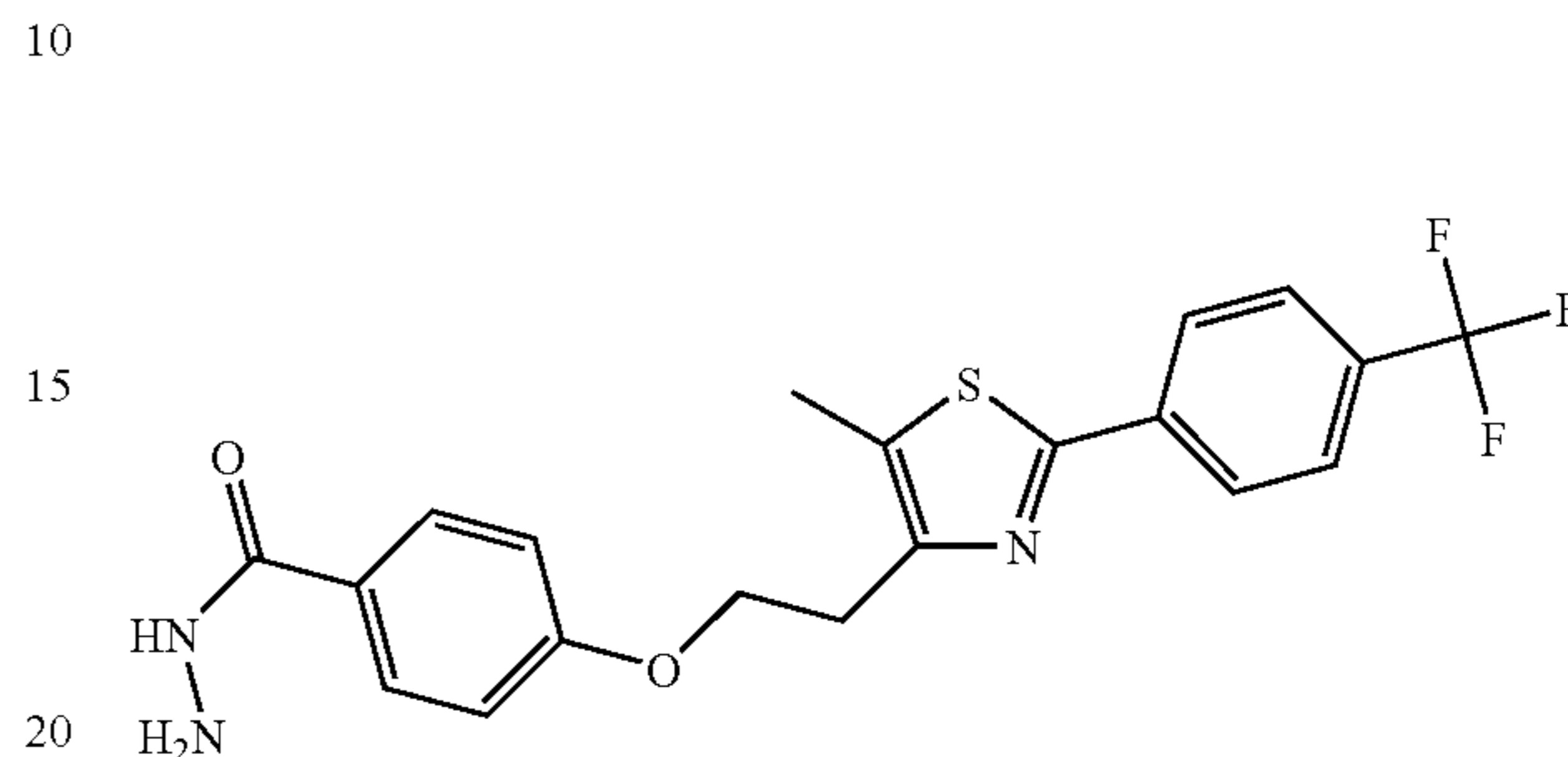
Intermediate: 4-{2-[5-Methyl-2-(4-trifluoromethyl-phenyl)-thiazol-4-yl]-ethoxy}-benzoic Acid Hydrazide
