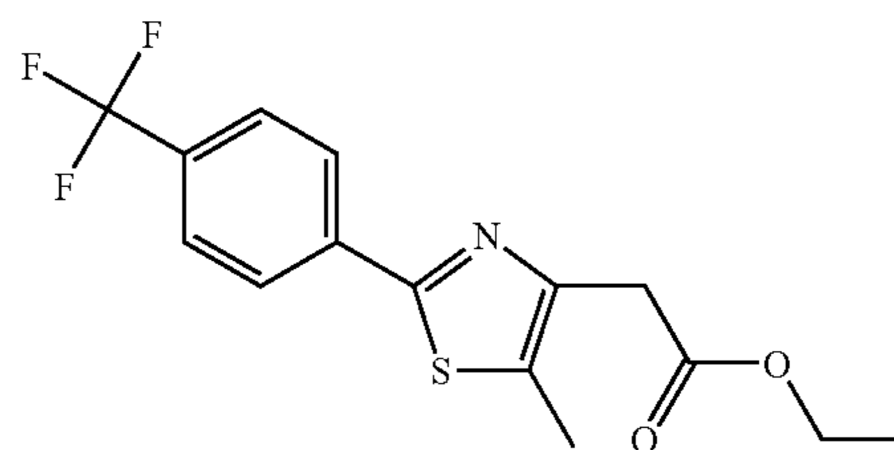
Intermediate: [5-Methyl-2-(4-trifluoromethyl-phenyl)-thiazol-4-yl]-acetic Acid Ethyl Ester
