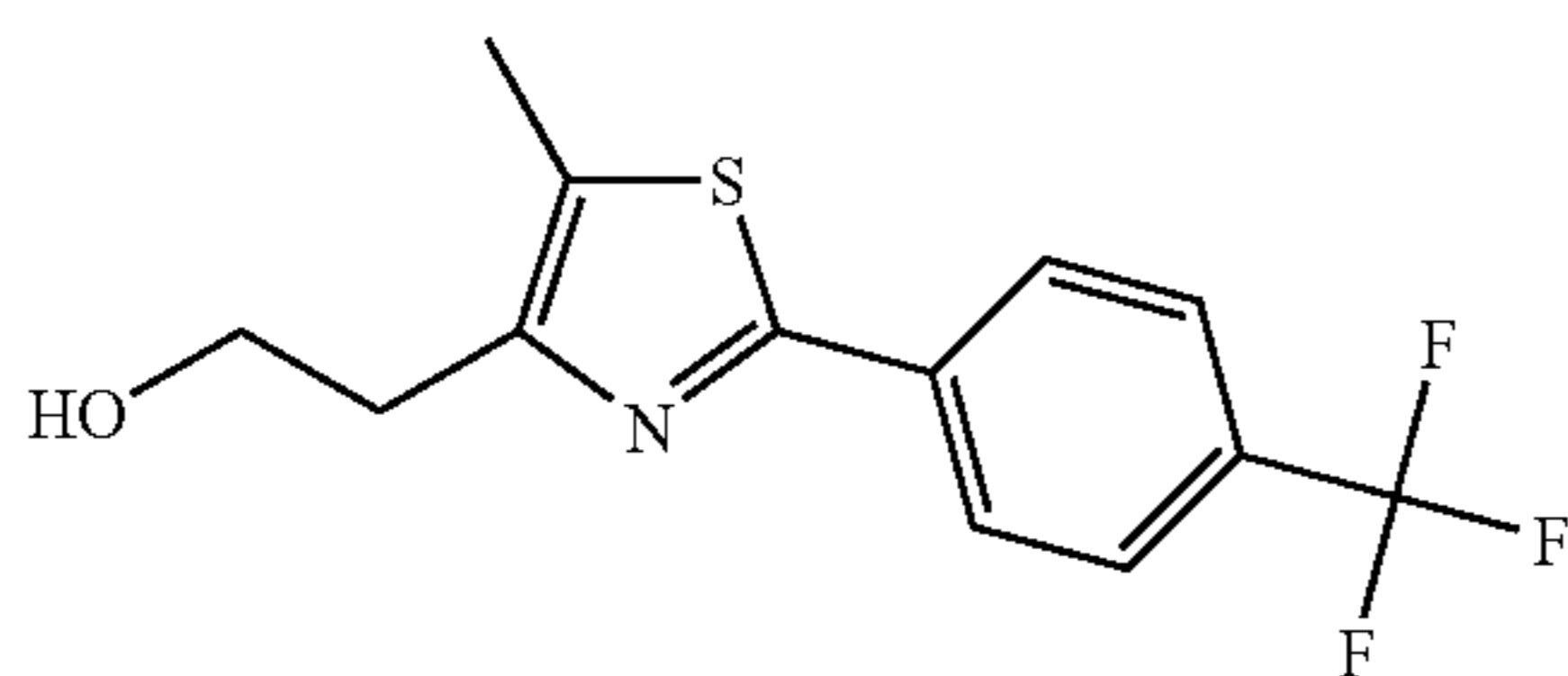
Intermediate: 4-(2-hydroxy-ethyl)-5-methyl-2-(4-trifluoromethyl-phenyl)thiazole
