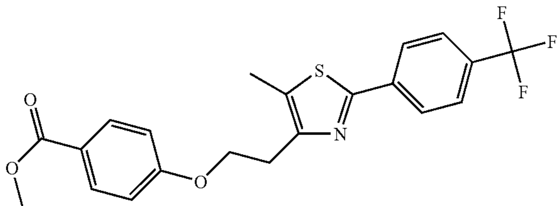
Intermediate: 4-[5-Methyl-2-(4-trifluoromethyl-phenyl)-thiazol-4-yl]ethoxy]-benzoic Acid Methyl Ester
