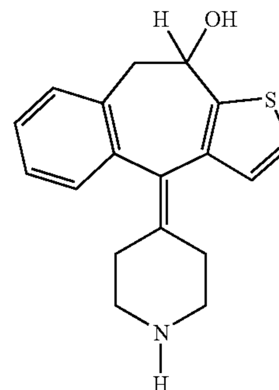
10-HYDROXY-NORKETOTIFEN
