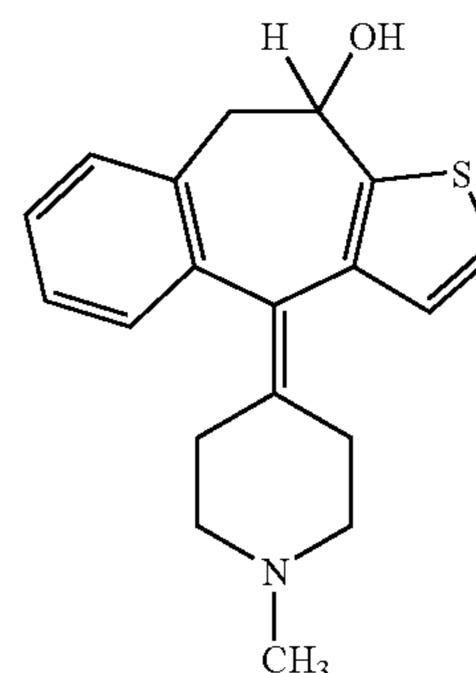
10-HYDROXY-KETOTIFEN
