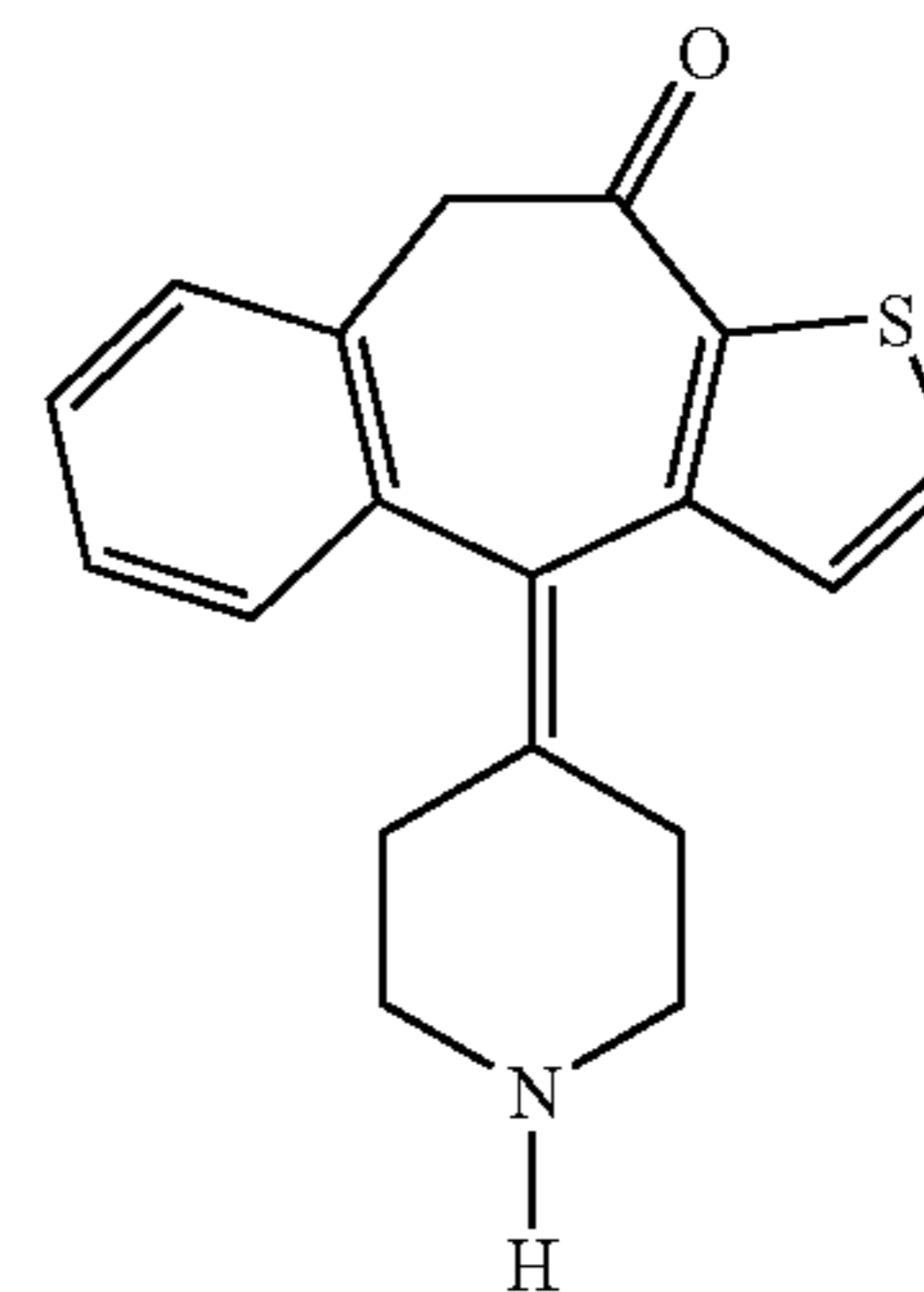
NOR-KETOTIFEN
